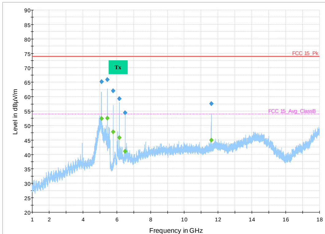
Figure 18: 1-18 GHz 802.11n HT Mode 5 MHz, Mid Channel
