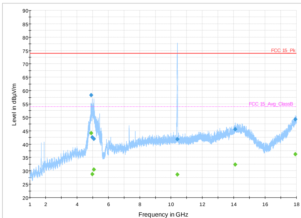
Figure 33: 1-18 GHz 802.11n HT Mode 40 MHz, High Channel
