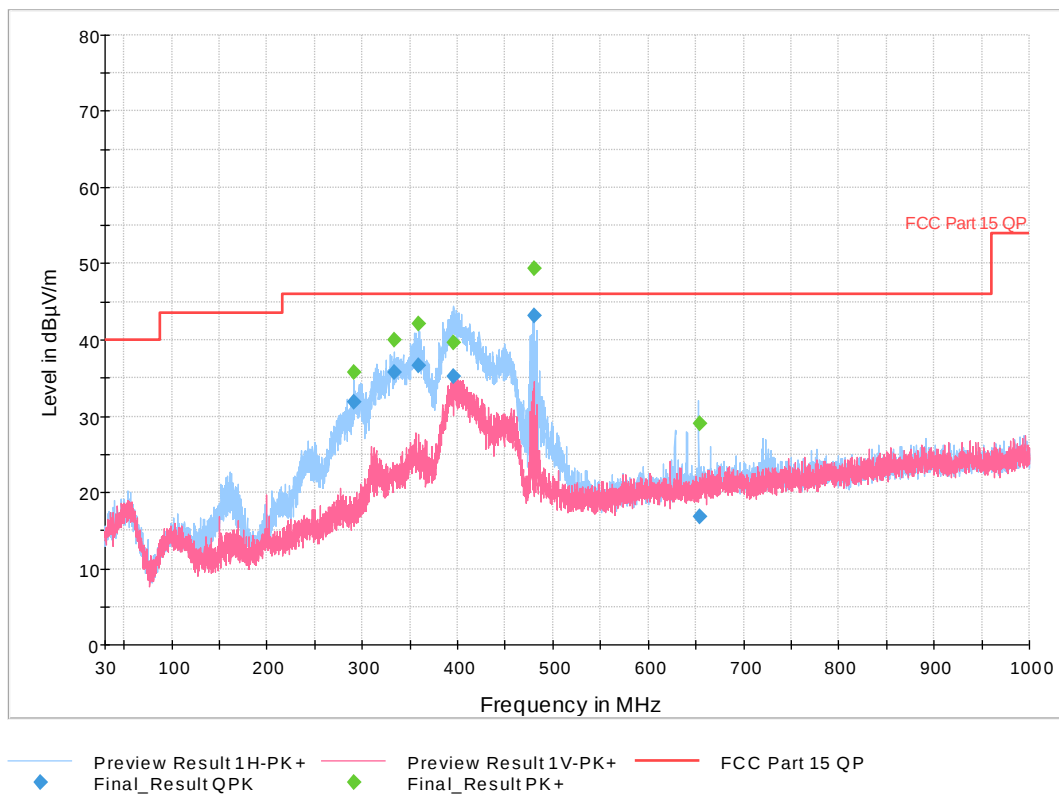
Figure 31: 30 MHz-1 GHz 802.11n HT Mode 40 MHz, Low Channel
