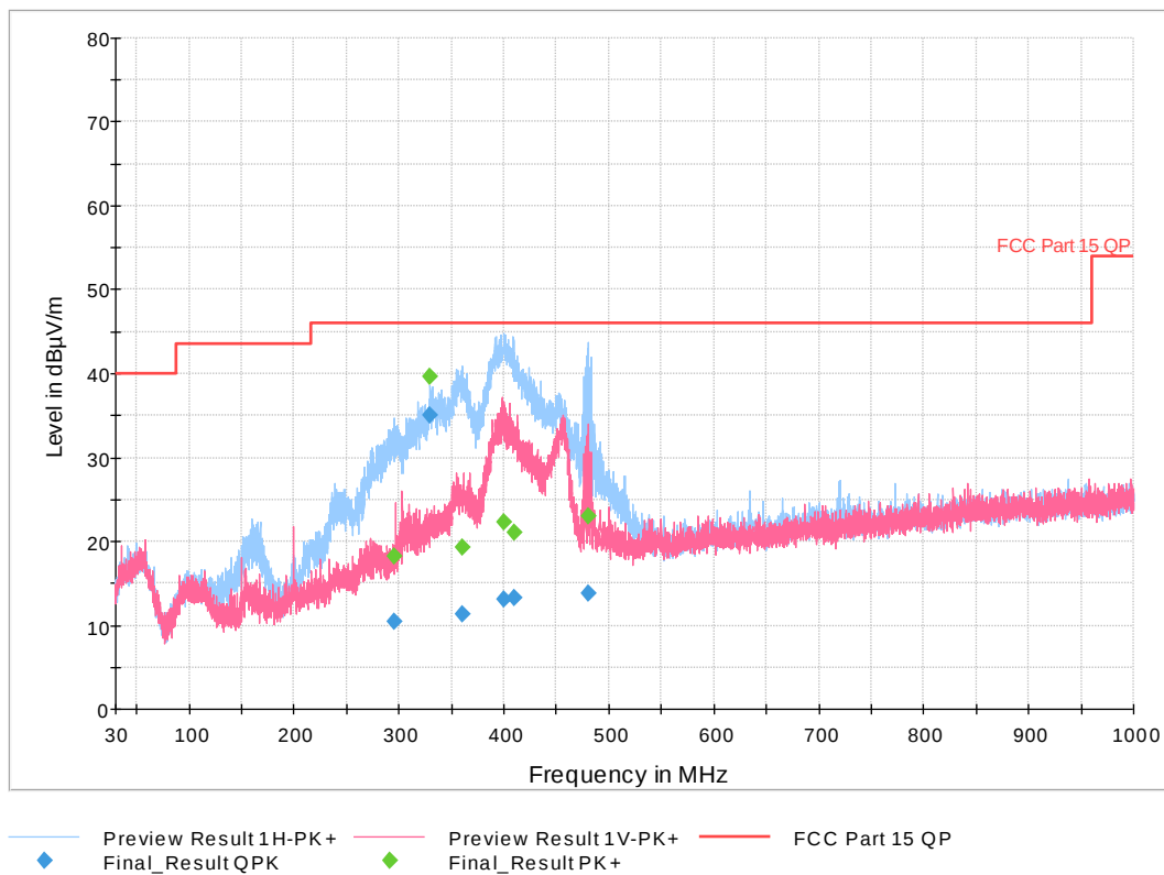
Figure 1: 30 MHz-1 GHz 802.11a Mode 5 MHz, Mid Channel
