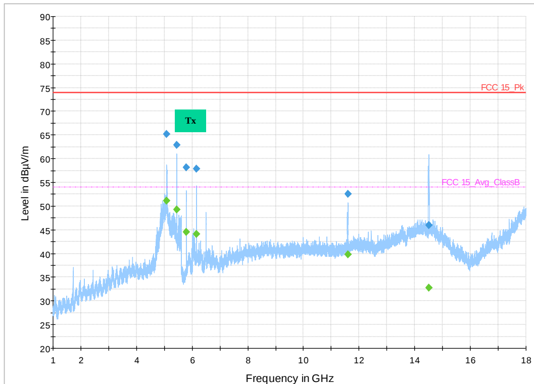
Figure 23: 1-18 GHz 802.11n HT Mode 10 MHz, Mid Channel
