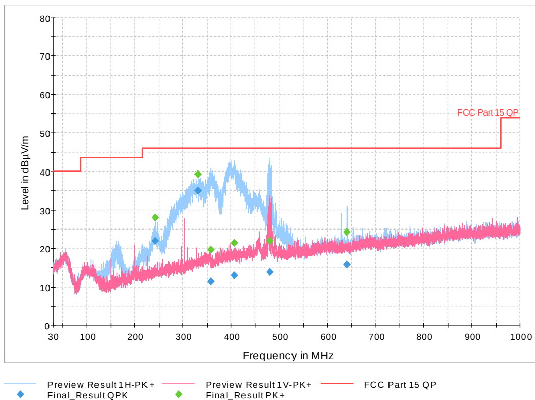
Figure 16: 30 MHz-1 GHz 802.11n HT Mode 5 MHz, Low Channel
