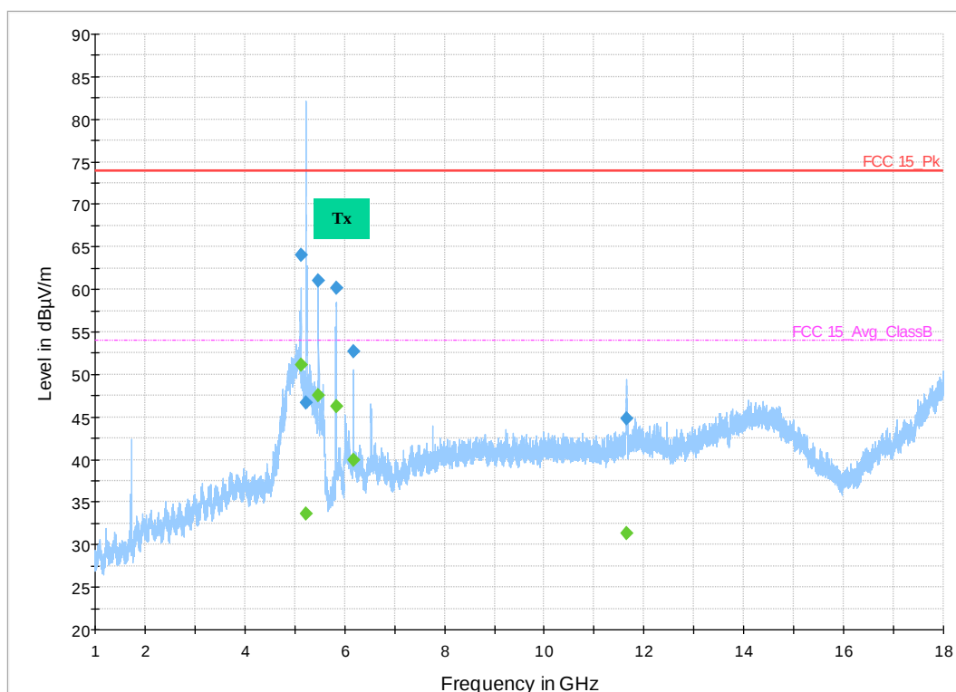
Figure 29: 1-18 GHz 802.11n HT Mode 20 MHz, High Channel
