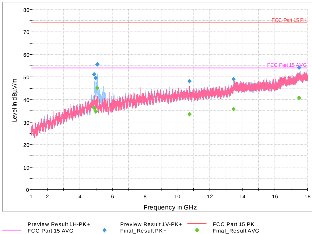
Figure 42: 1-18 GHz 802.11ac VHT Mode 40 MHz, High Channel
