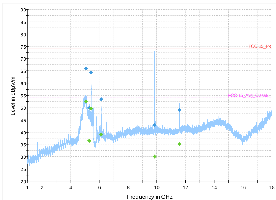
Figure 28: 1-18 GHz 802.11n HT Mode 20 MHz, Mid Channel
