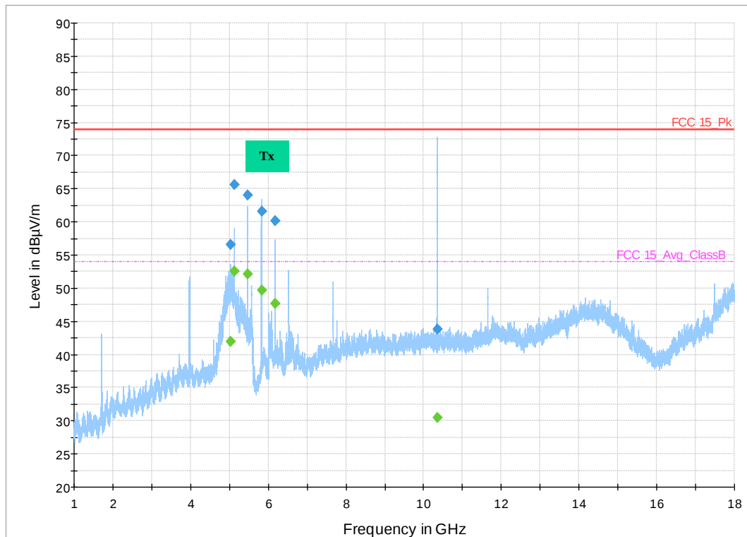
Figure 4: 1-18 GHz 802.11a Mode 5 MHz, High Channel
