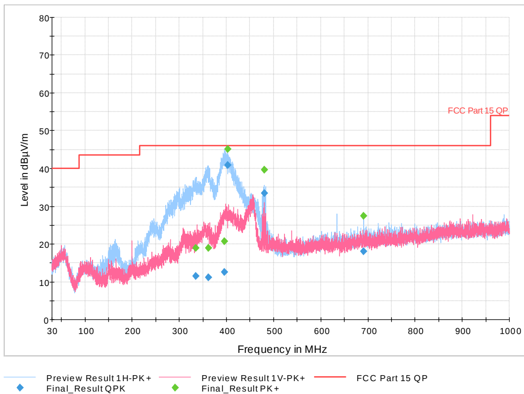
Figure 21: 30 MHz-1 GHz 802.11n HT Mode 10 MHz, Mid Channel
