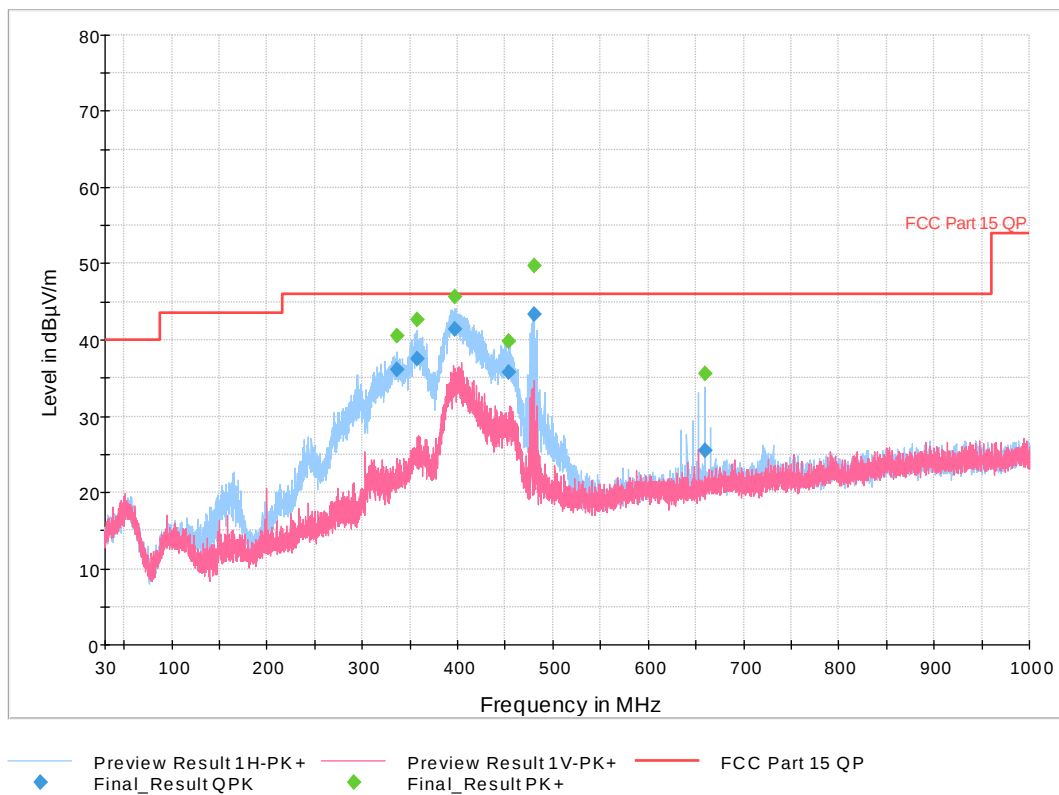
Figure 26: 30 MHz-1 GHz 802.11n HT Mode 20 MHz, Mid Channel
