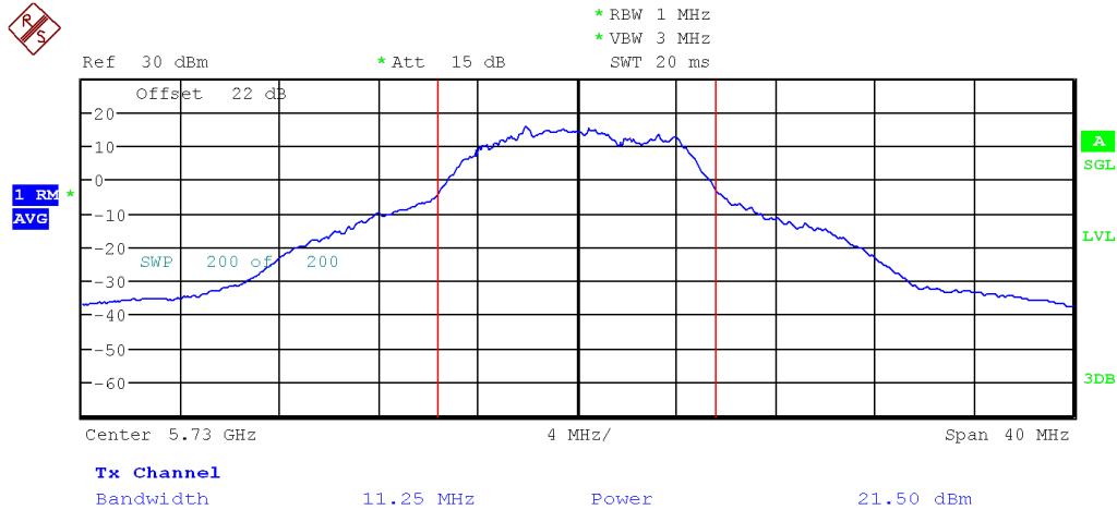
Figure 8: FCC Uncorrelated Max Conducted Power-5730 MHz-802.11n-MCS 0-10MHz-Ch1
