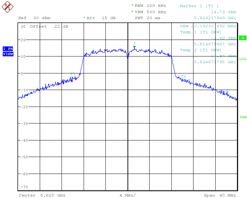
Figure 16: Occupied Bandwidth-5825 MHz-802.11a
