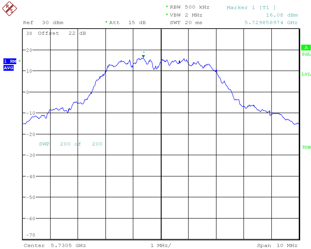
Figure 30: FCC Uncorrelated Power Spectral Density-5730.5 MHz-802.11n-HT MCSO -5MHz-Ch1
