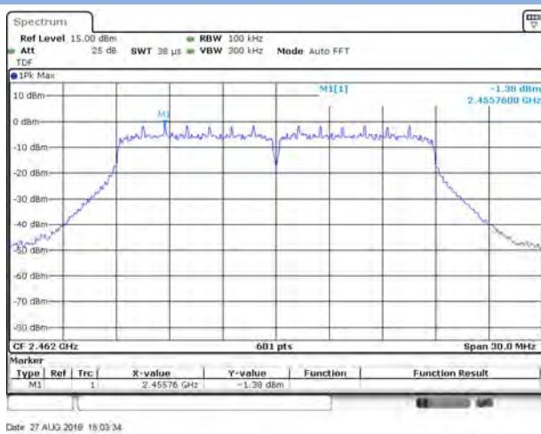
802.11n-20 MHz HIGH CHANNEL, Carrier level
