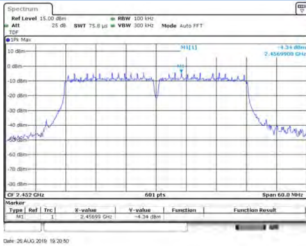
802.11n-40 MHz HIGH CHANNEL, Carrier level
