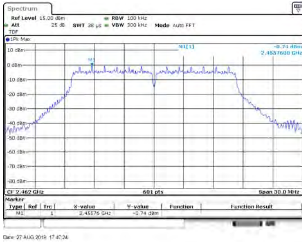
802.11g HIGH CHANNEL, Carrier level
