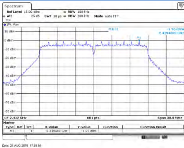
802.11n-20 MHz LOW CHANNEL, Carrier level
