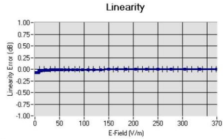
Linearity: \pm 1.64\% ( \pm 0.07\text{dB} )
