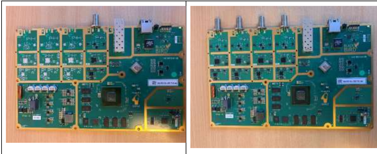
Picture 2 PCBs: C251 to the left and C254 to the right. C251 one 75 ohm coaxial port and C254 four 75 ohm coaxial ports.
