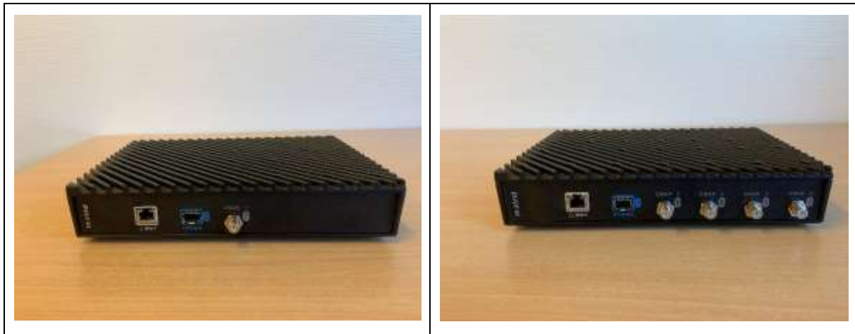
Picture 1 Units: C251 to the left and C254 to the right. C251 one 75 ohm coaxial port and C254 four 75 ohm coaxial ports.
