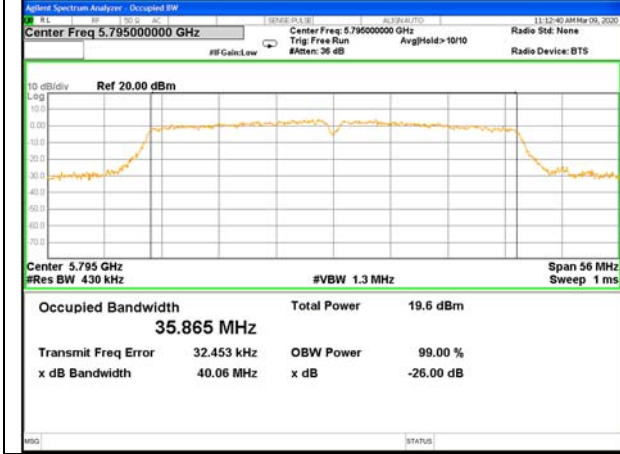
W58_11ac40_Higher_26BW and 99%
