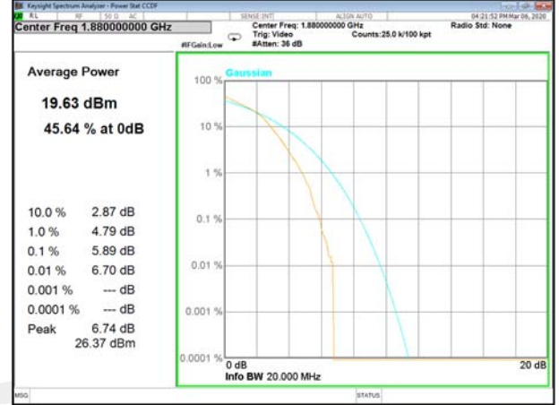
B2_100_QPSK_High
