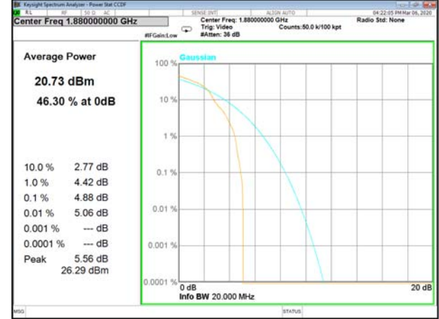
B2_1_QPSK_High
