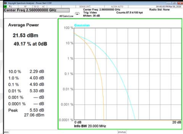
B7_100_Q16_High
