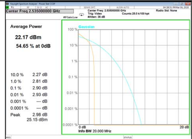
B7_1_QPSK_Middle
