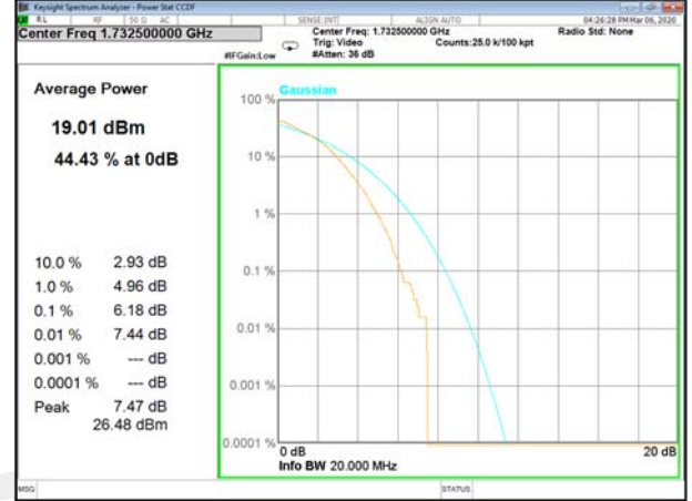
B4_100_QPSK_High
