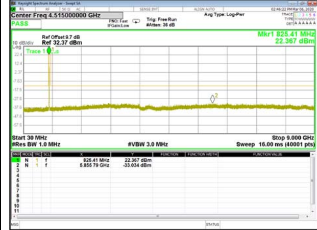
B5_QPSK_3M_Mid_CDT_Spurious
