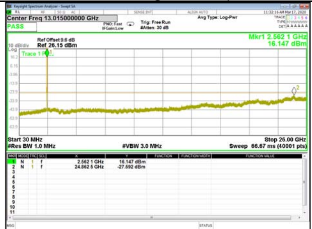
B7_Q16_10M_High_CDT_Spurious
