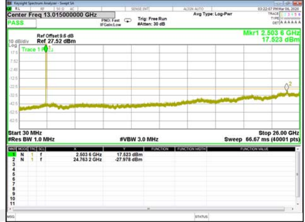
B7_Q16_5M_Mid_CDT_Spurious
