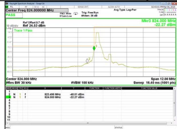
B5_Q16_1.4M_Low_1-RB_Bedge
