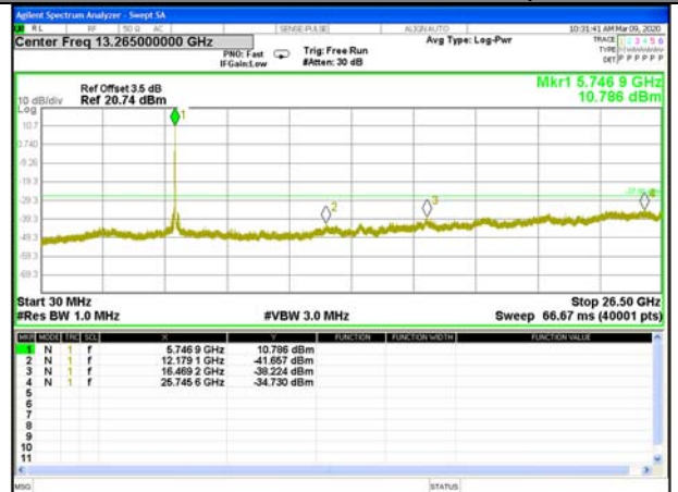
W58_11n20_Lower_Conducted Spurious
