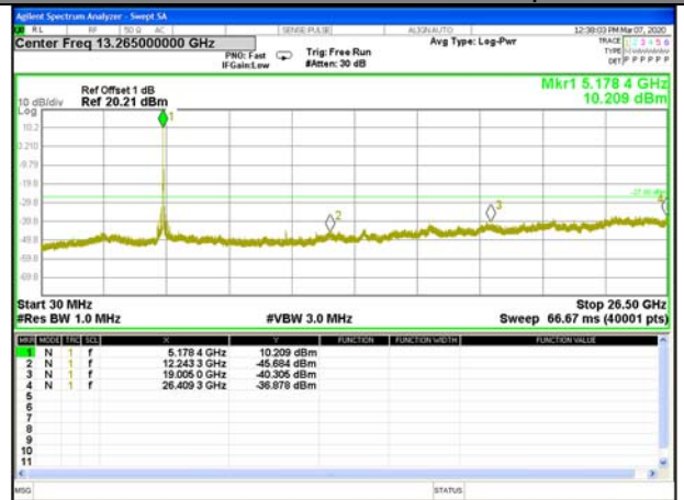
W52_11a20_Lower_Conducted Spurious
