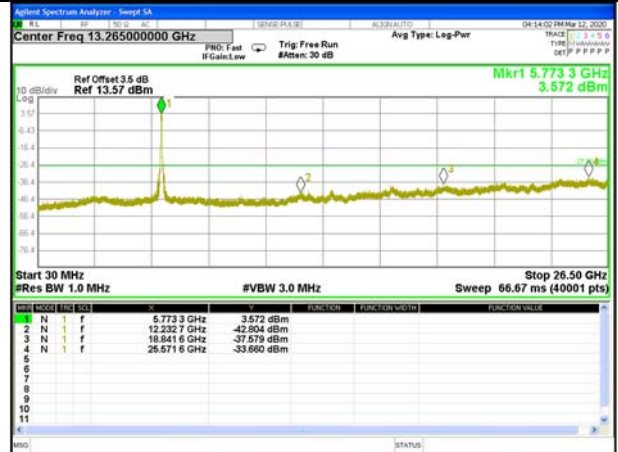
W58_11ac80_Spurious_30M26BWG_5775M
