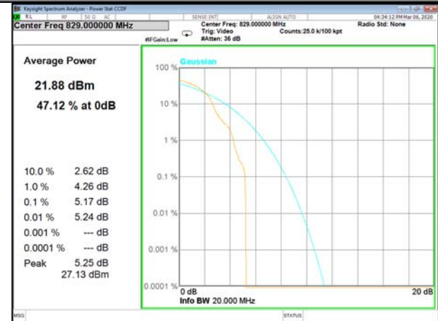
B5_1_QPSK_Middle
