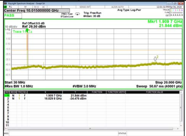
16QAM_1.4M_Higher_Conducted Spurious
