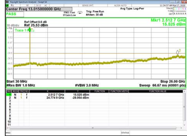
B7_QPSK_15M_Mid_CDT_Spurious
