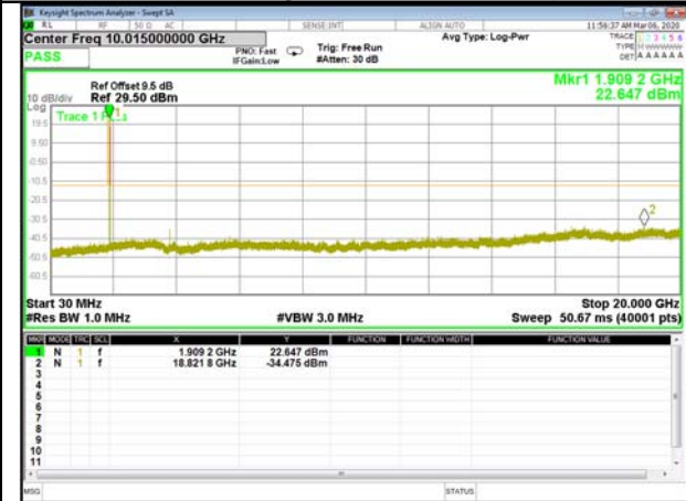
QPSK_1.4M_Higher_Conducted Spurious
