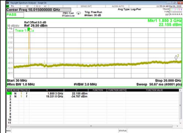
QPSK_1.4M_Middle_Conducted Spurious
