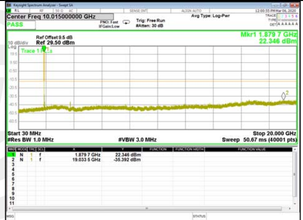
16QAM_1.4M_Higher_Conducted Spurious
