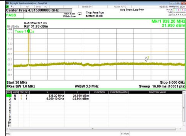
B5_QPSK_5M_High_CDT_Spurious
