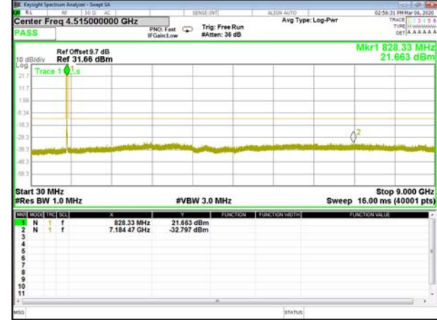
B5_QPSK_5M_Mid_CDT_Spurious
