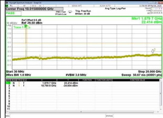
QPSK_1.4M_Higher_Conducted Spurious
