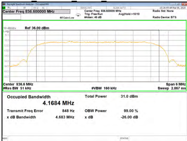
B5_WCDMA_Middle_26BW and 99%
