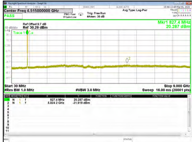
B5_HSDPA_Lower_Conducted_Spurious
