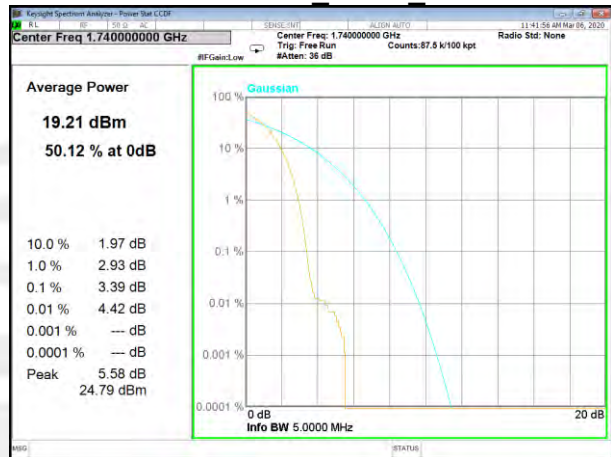
HSDPA4_Middle_
