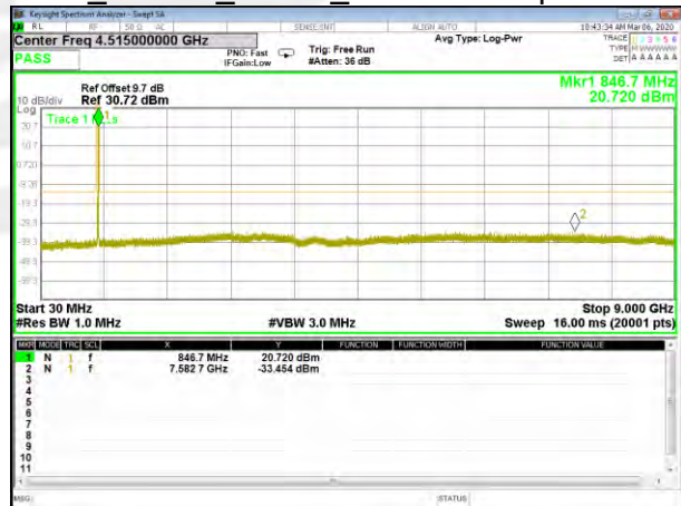
B5_HSDPA_Higher_Conducted_Spurious
