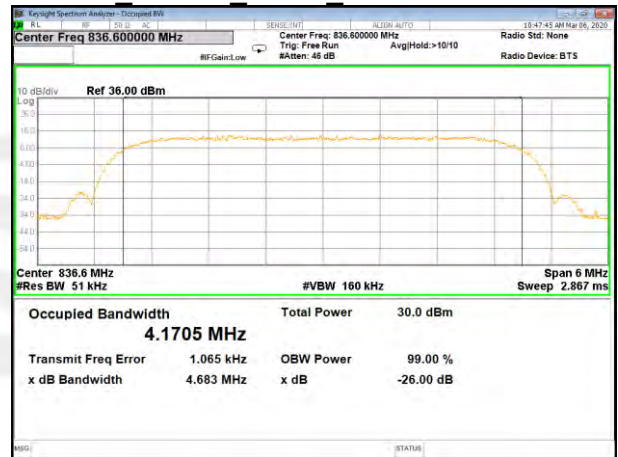
B5_HSDPA_Middle_26BW and 99%
