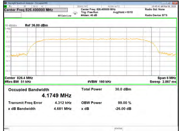
B5_HSDPA_Lower_26BW and 99%
