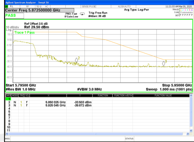
W58_11ac20_Middle_Conducted Spurious
