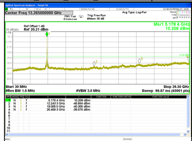
W52_11a20_Lower_Conducted Spurious
