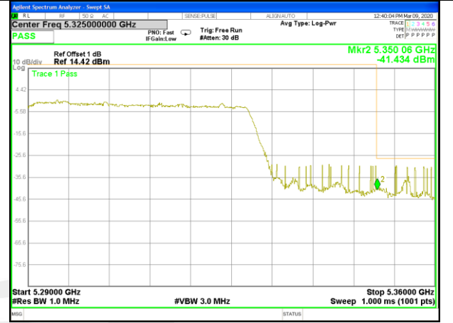
W53_11ac80_CH58(5290MHz)_Band edge_Right
