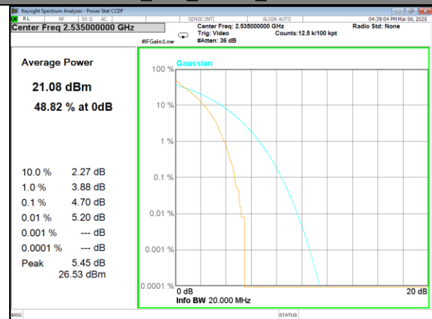
B7_100_QPSK_Middle
