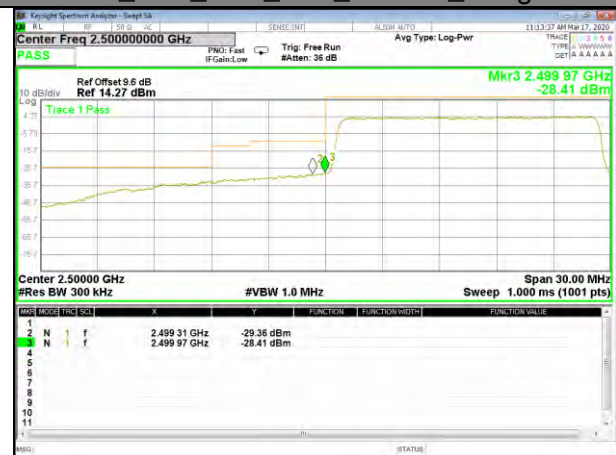
B7_Q16_15M_Low_Full-RB_Bedge
