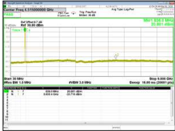
B5_HSUPA_Middle_Conducted Spurious
