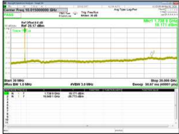
B4_HSUPA_Middle_Conducted Spurious
