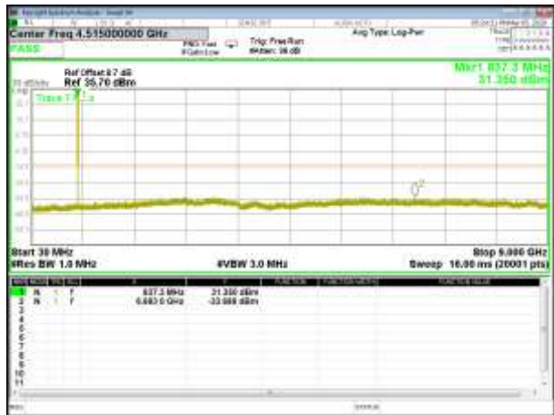
GSM_850_Middle_Conducted Spurious
