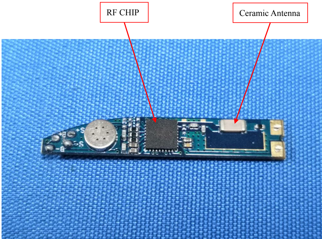
RF CHIP: Model : AC6936D Manufacturer: ZhuHai JieLi
