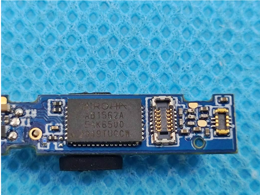
VIEW OF EUT(PORT) (Right ear bud)
