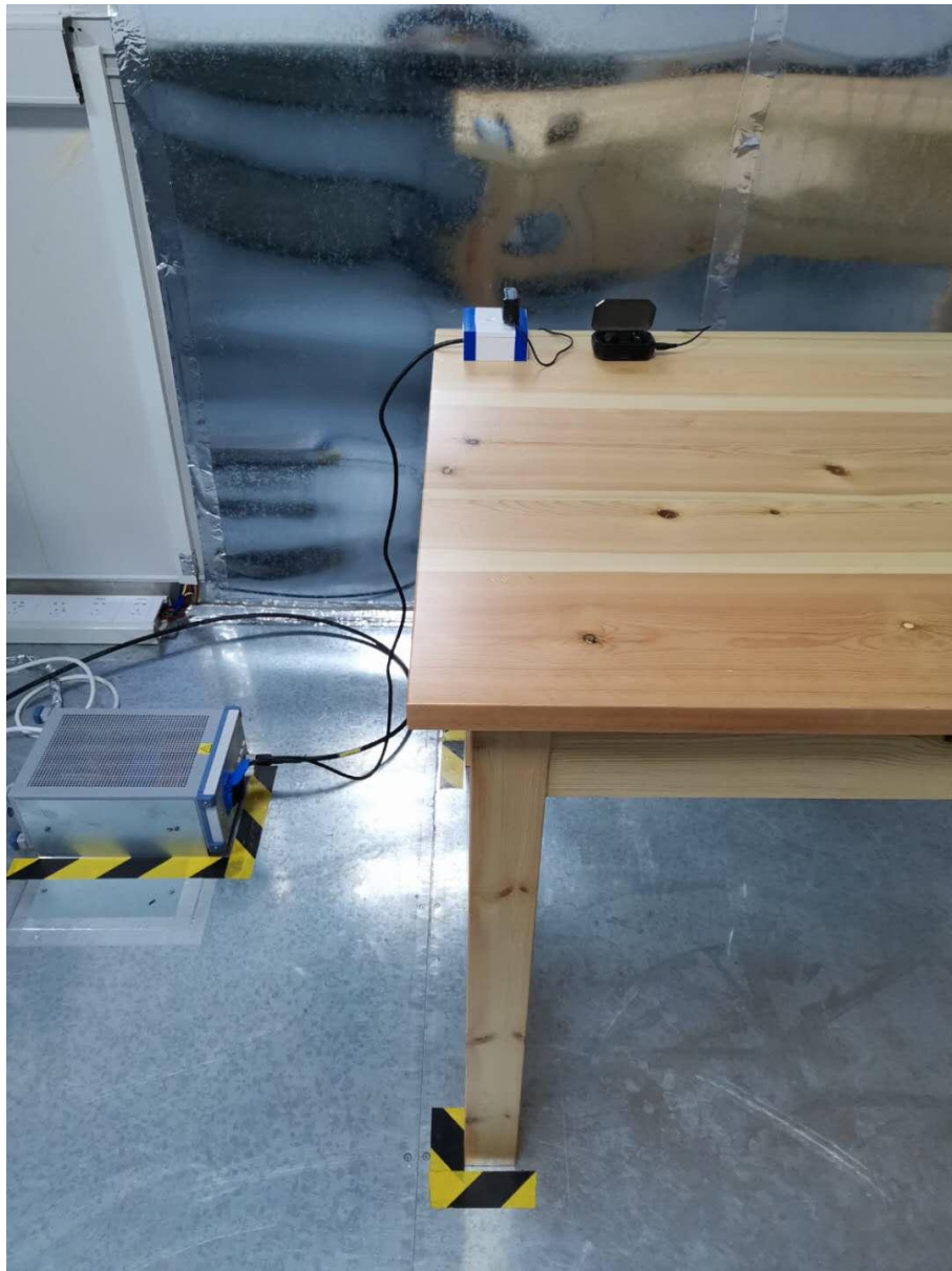
Conducted emission test setup
