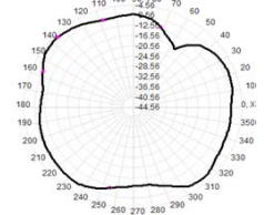
Total(H+V), Max=-6.34dBi, Crd=11.28
