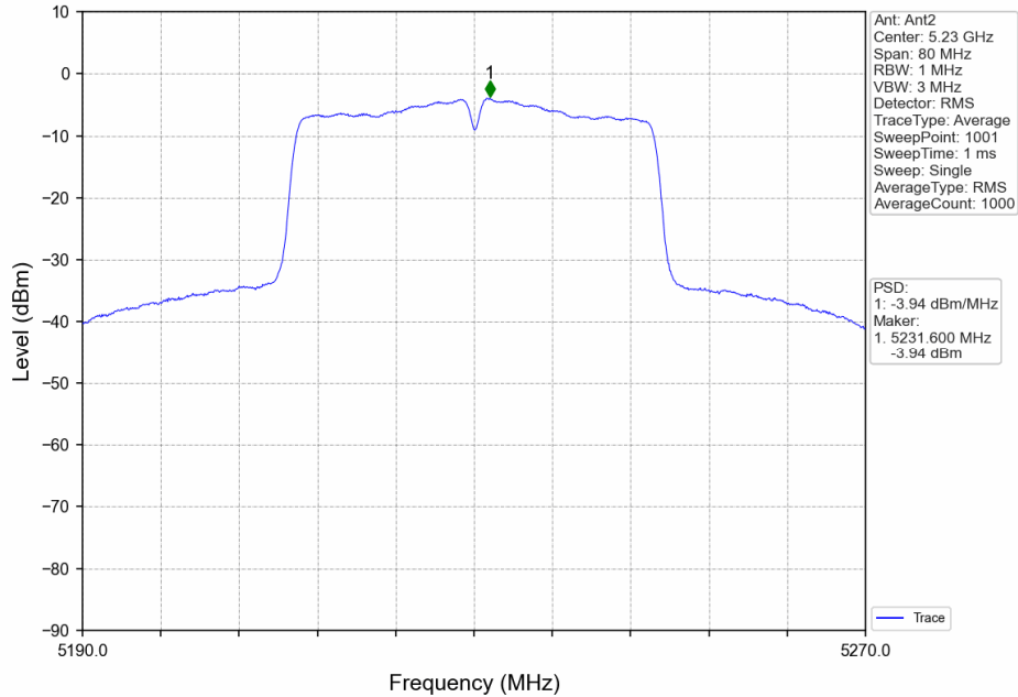
802.11ac(VHT40)_HCH_5230MHz_MIMO_NTNV
