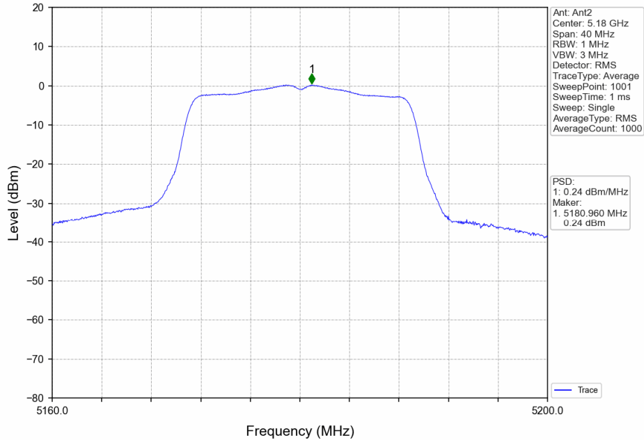
802.11ac(VHT20)_LCH_5180MHz_MIMO_NTNV
