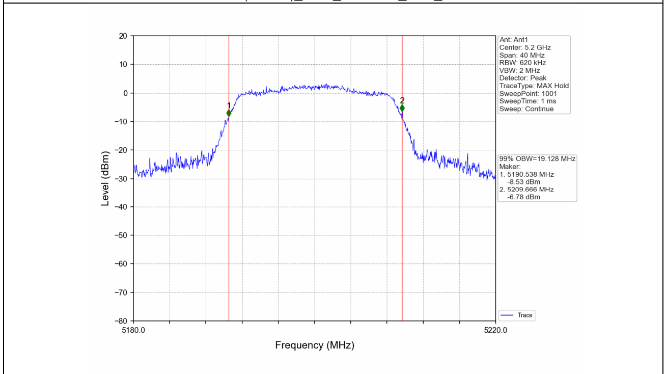
802.11ac(VHT20)_MCH_5200MHz_Ant1_NTNV
