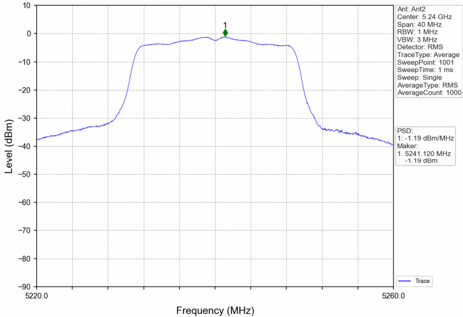
802.11ac(VHT20)_HCH_5240MHz_MIMO_NTNV
