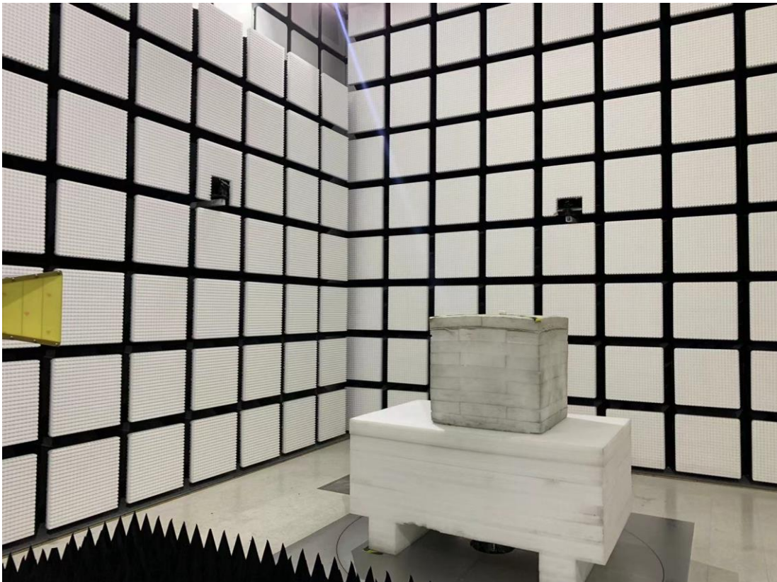
Radiated Emission Above 1-18GHz View
