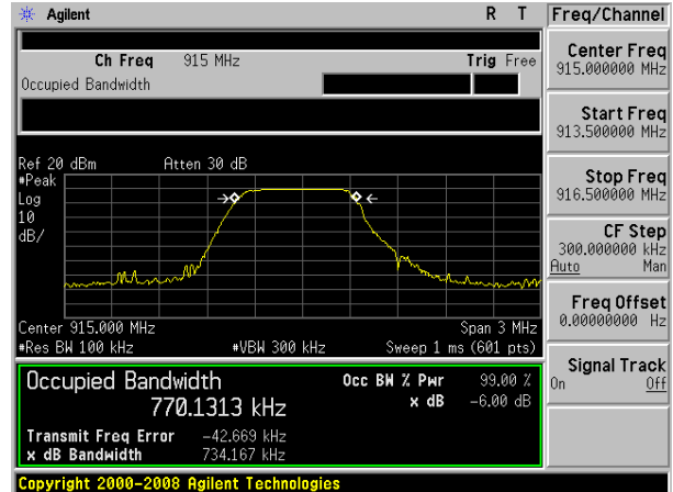
6dB Bandwidth plot on channel 13
