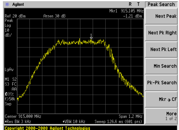
Power spectral density plot on channel 13
