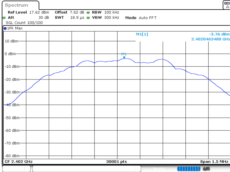
Tx. Spurious NVNT BLE-1M 2402MHz Ref
