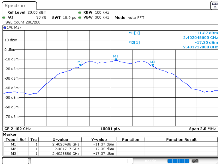
-6 dB BW NVNT BLE-1M 2402MHz 1M
