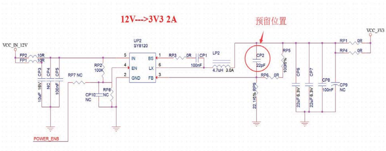
Figure 13 DC-DC step-down circuit diagram
