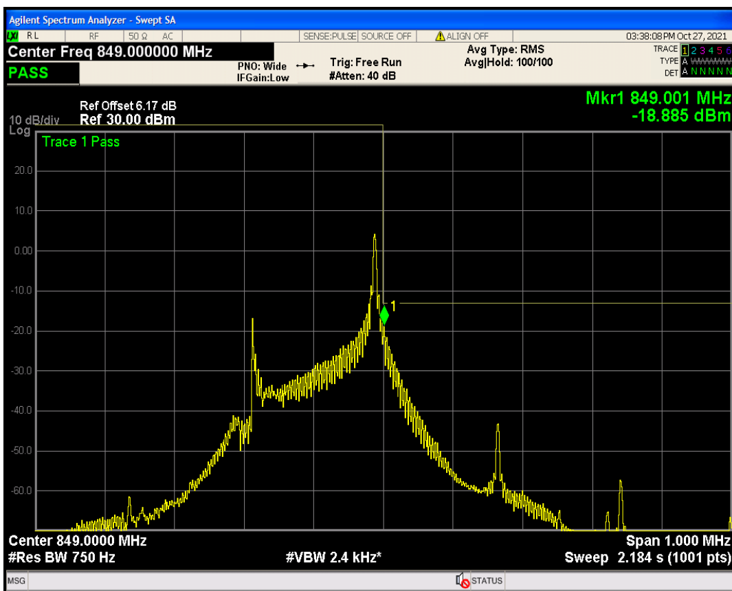
Band5 QPSK Channel=20649 nTones=1@47 Spacing=3.75kHz
