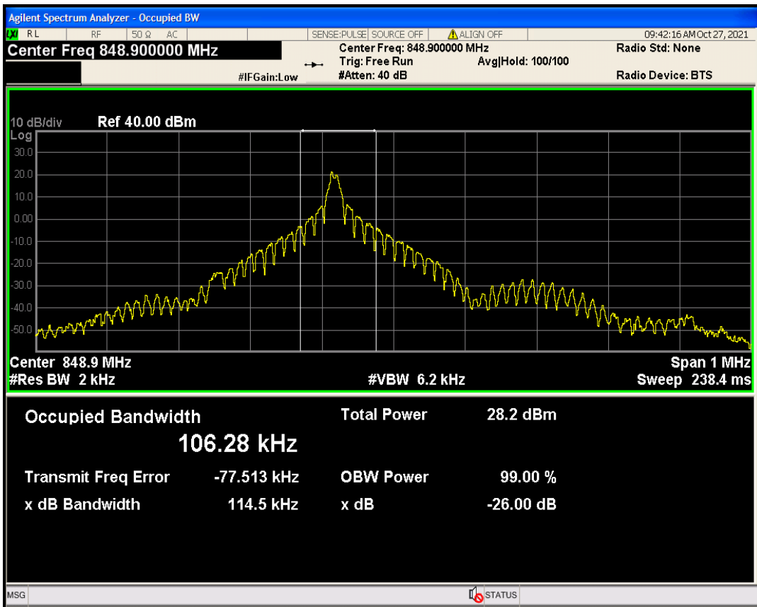
Band5 QPSK Channel=20649 nTones=12@0 Spacing=15kHz
