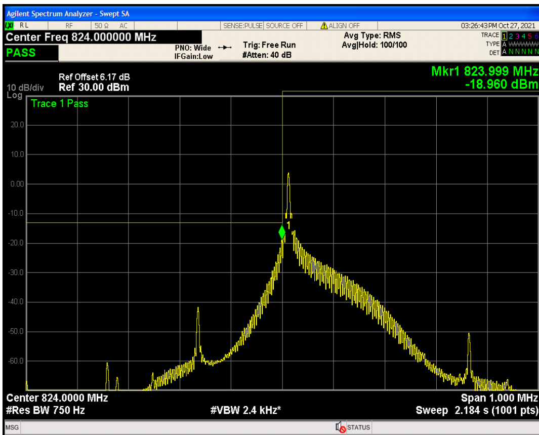
Band5 QPSK Channel=20401 nTones=1@0 Spacing=3.75kHz
