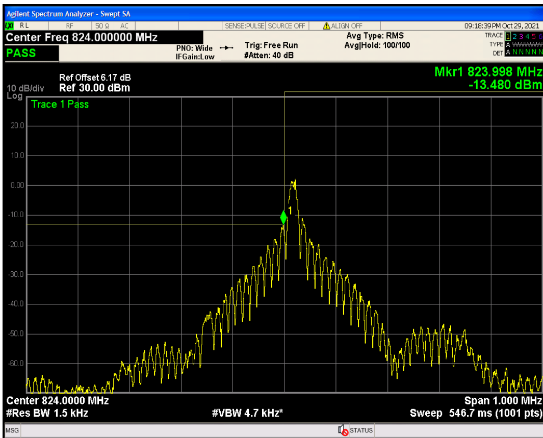
Band5 QPSK Channel=20401 nTones=1@0 Spacing=15kHz
