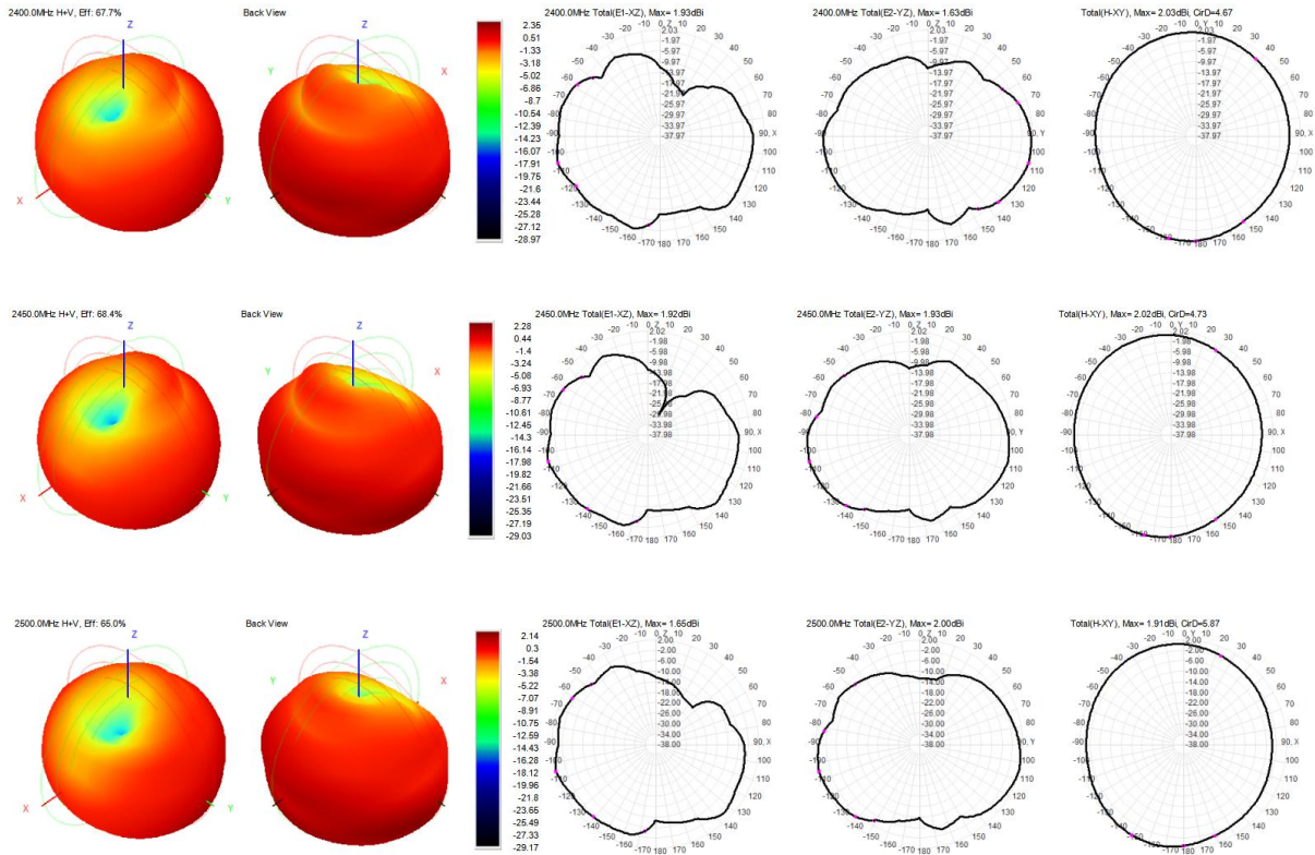
Figure 10 Antenna pattern
