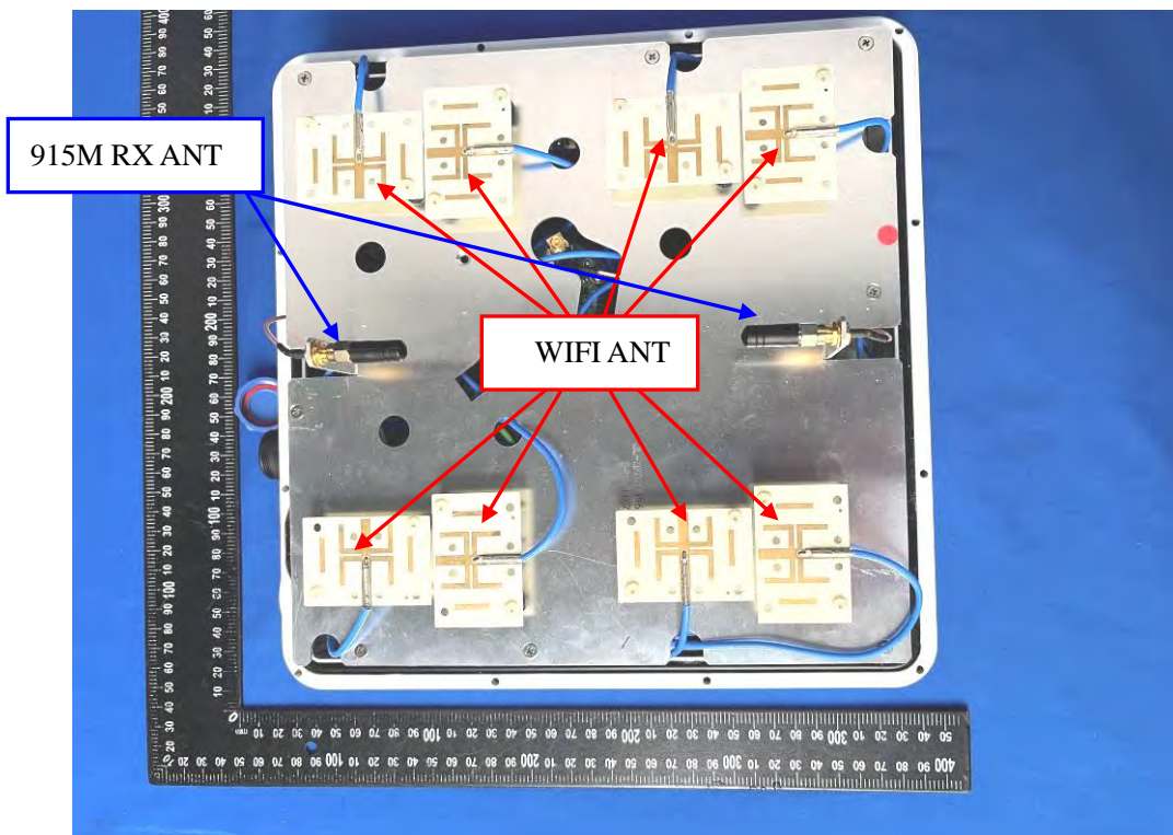
EUT View
