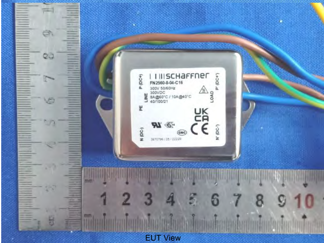
EUT View
