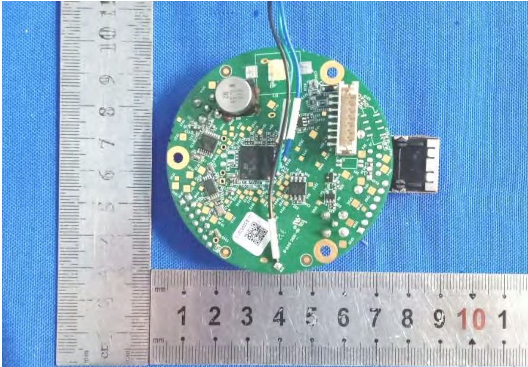
EUT View
