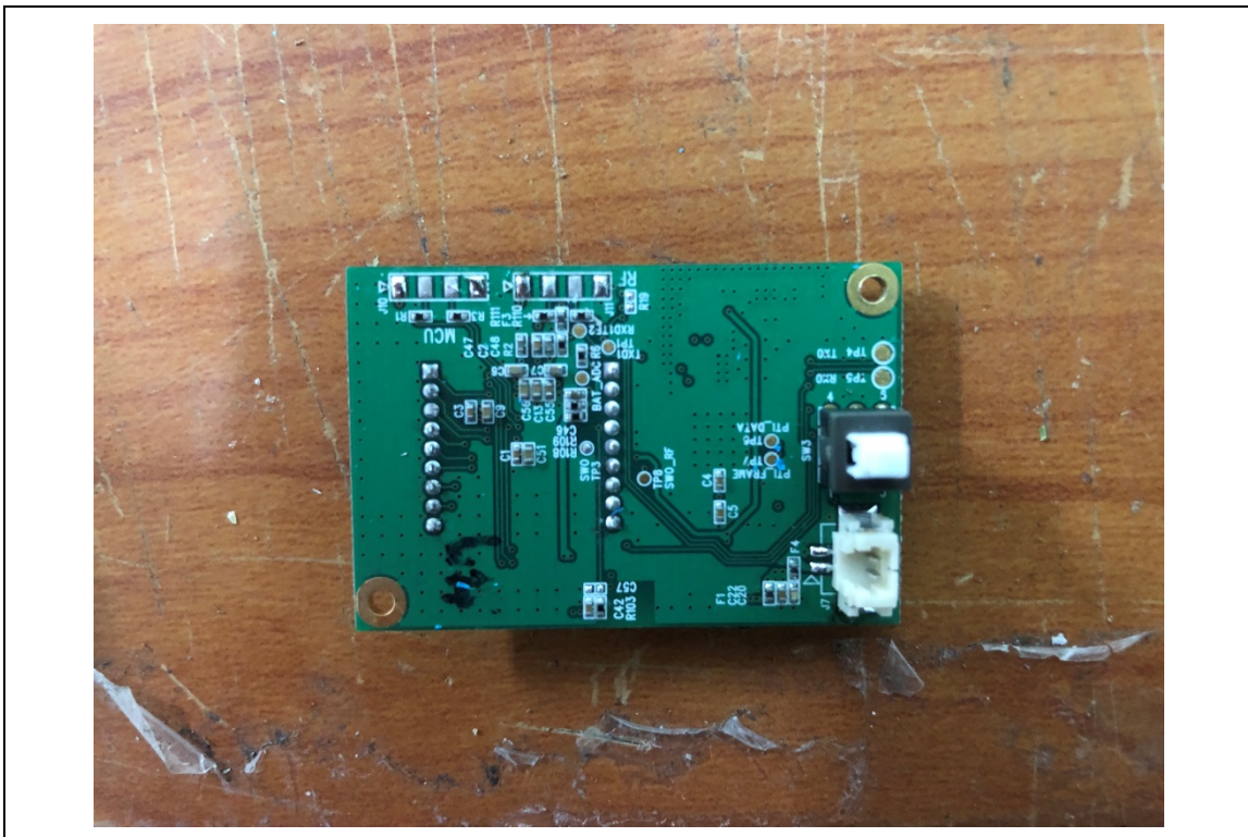
MainBoard-Rear
