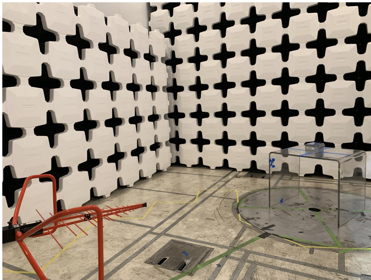
Photograph 1. Radiated Emission Test Setup – 30 MHz to 1 GHz
