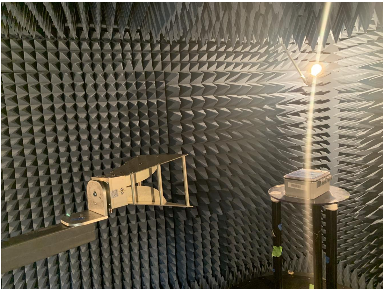
Photograph 5. Radiated Emission Test Setup - 1 GHz – 18 GHz
