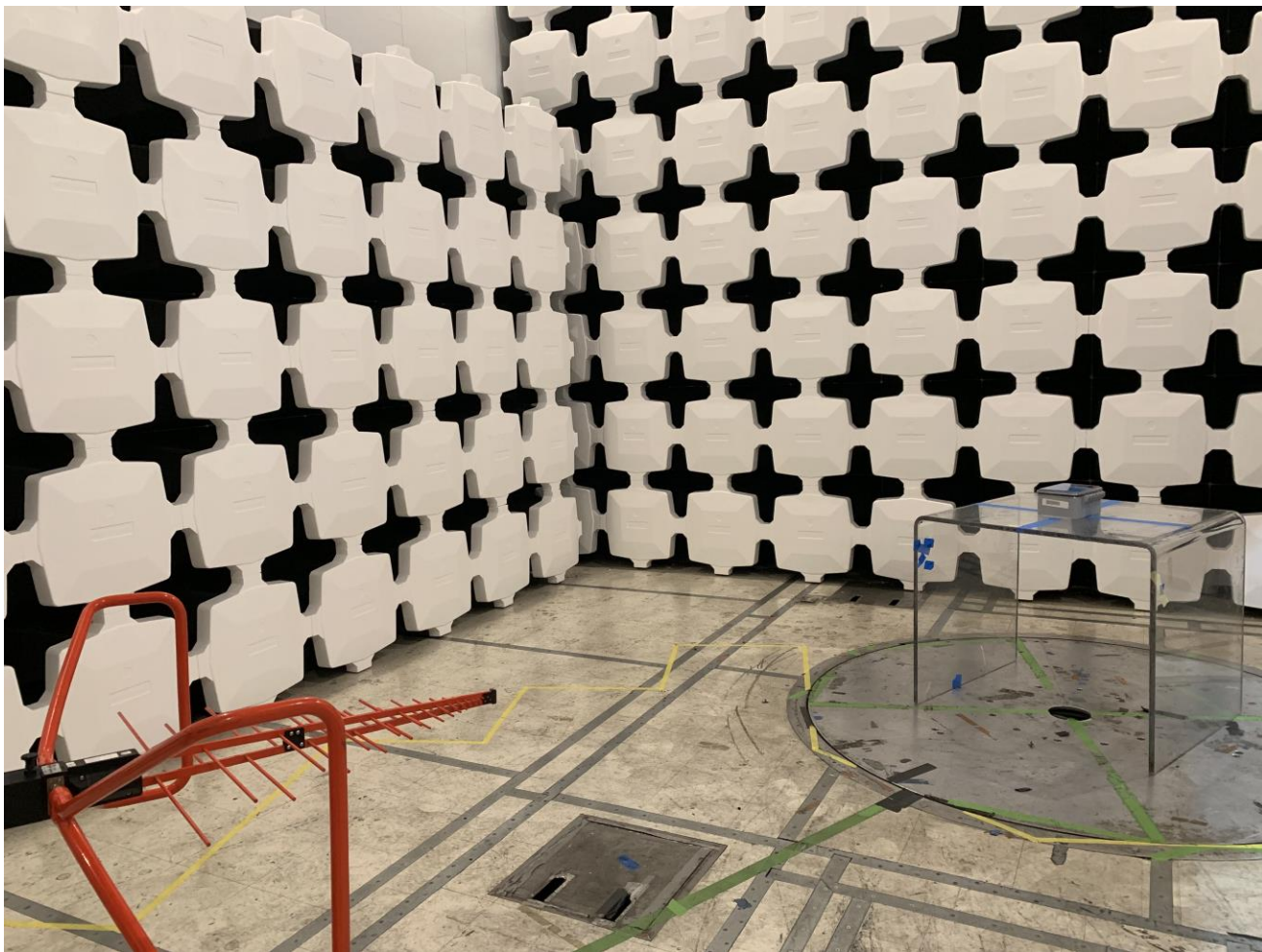
Photograph 4. Radiated Emission Test Setup – 30 MHz to 1 GHz
