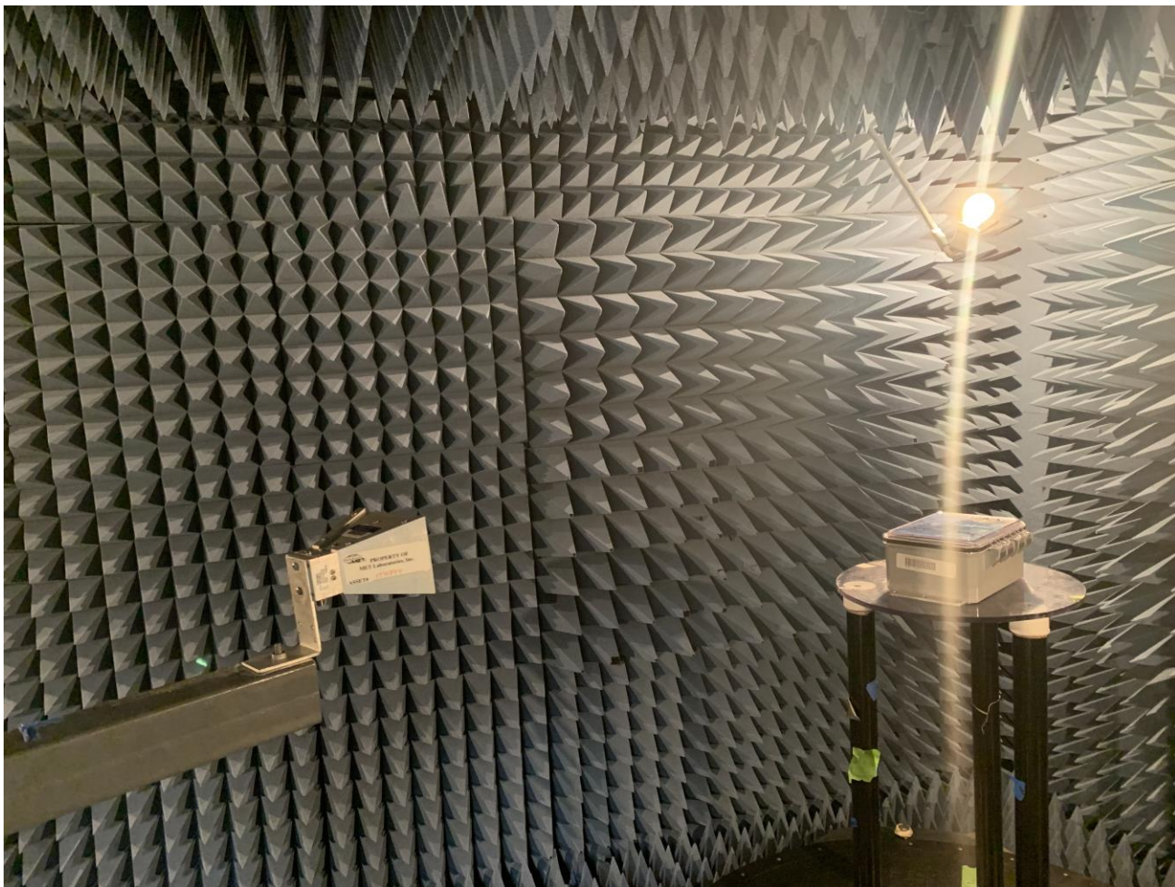
Photograph 6. Radiated Emission Test Setup - 18 GHz – 40 GHz
