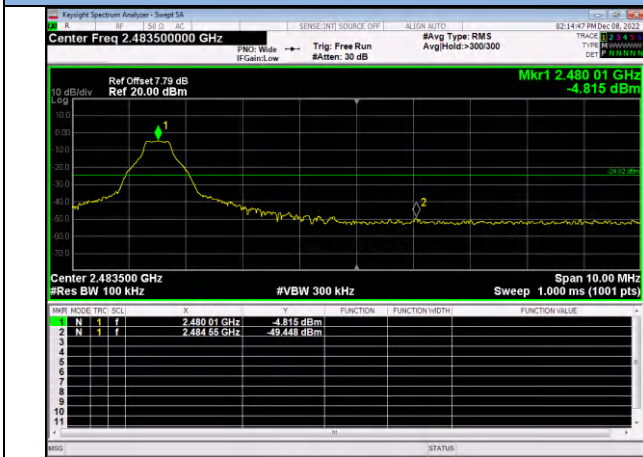
GFSK / High Channel / 2480
