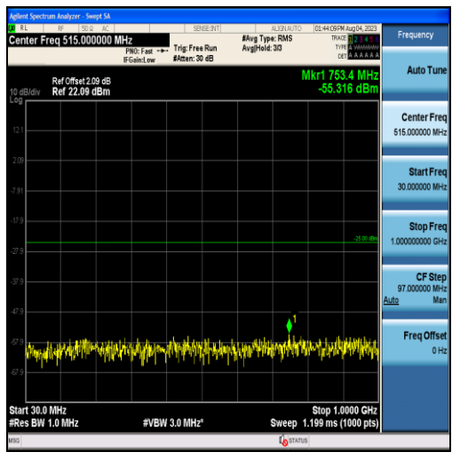
Band41-15MHz-QPSK-40620-75RB#0-Range1:30~1000MHz
