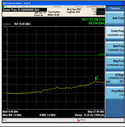
Band41-15MHz-16QAM-39725-75RB#0-Range3:6000~27000MHz
