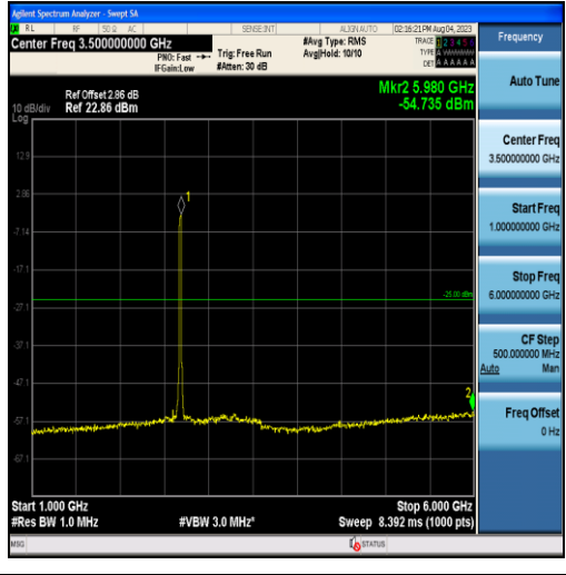
Band41-20MHz-16QAM-41490-100RB#0-Range2:1000~6000MHz
