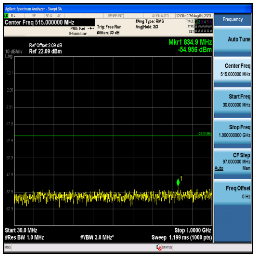
Band41-5MHz-QPSK-39675-25RB#0-Range1:30~1000MHz
