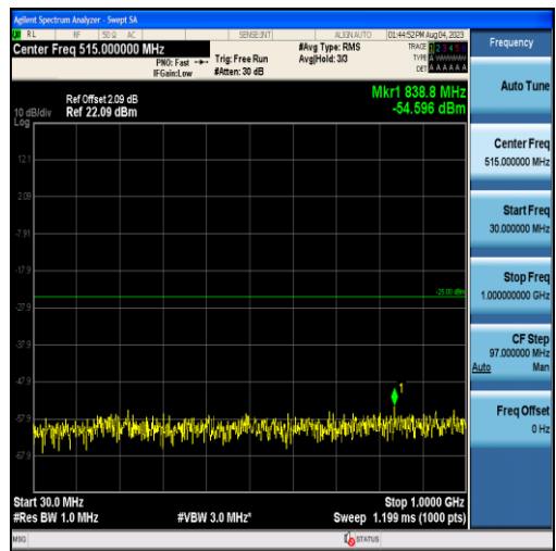
Band41-15MHz-QPSK-41515-75RB#0-Range1:30~1000MHz
