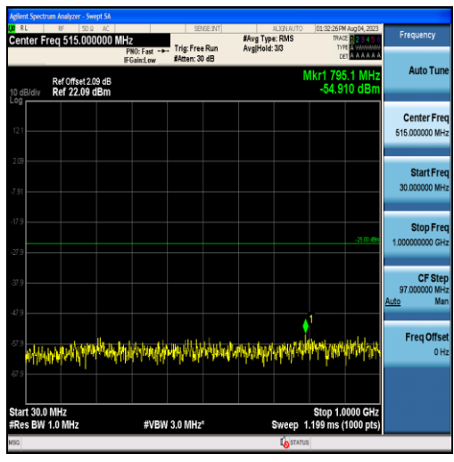
Band41-10MHz-QPSK-40620-50RB#0-Range1:30~1000MHz
