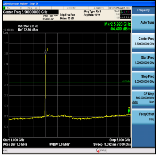
Band41-15MHz-16QAM-39725-75RB#0-Range2:1000~6000MHz
