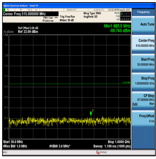
Band41-20MHz-QPSK-39750-100RB#0-Range1:30~1000MHz
