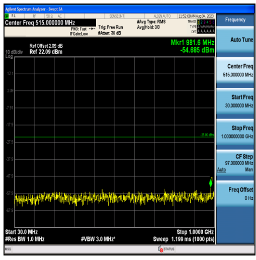
Band38-20MHz-16QAM-38000-100RB#0-Range1:30~1000MHz
