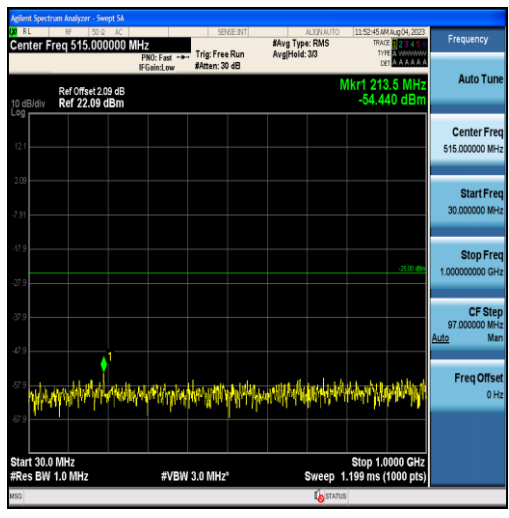
Band38-20MHz-16QAM-38150-100RB#0-Range1:30~1000MHz
