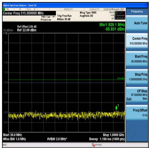
Band41-5MHz-16QAM-40620-25RB#0-Range1:30~1000MHz
