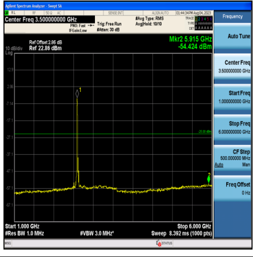
Band41-15MHz-16QAM-40620-75RB#0-Range2:1000~6000MHz
