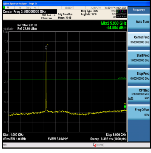
Band41-10MHz-16QAM-40620-50RB#0-Range2:1000~6000MHz
