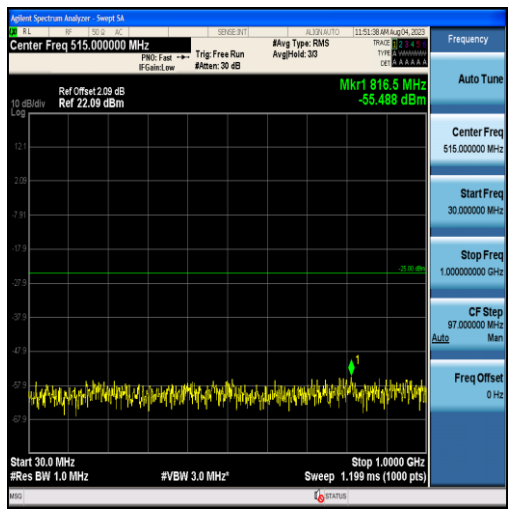
Band38-20MHz-QPSK-38000-100RB#0-Range1:30~1000MHz
