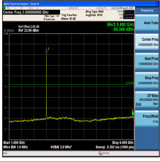
Band41-5MHz-16QAM-39675-25RB#0-Range2:1000~6000MHz
