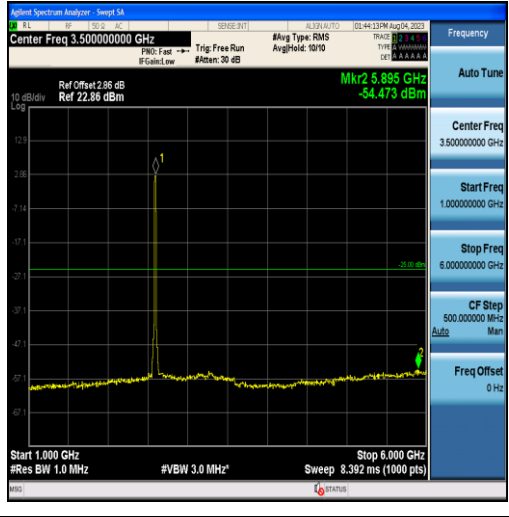
Band41-15MHz-QPSK-40620-75RB#0-Range2:1000~6000MHz
