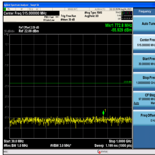
Band41-20MHz-QPSK-41490-100RB#0-Range1:30~1000MHz
