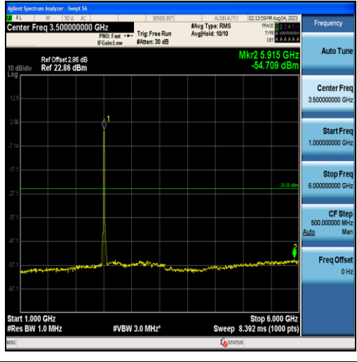
Band41-20MHz-16QAM-39750-100RB#0-Range2:1000~6000MHz
