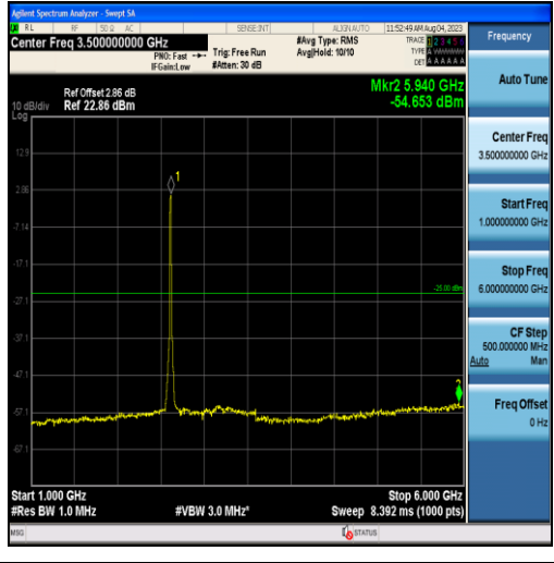
Band38-20MHz-16QAM-38150-100RB#0-Range2:1000~6000MHz
