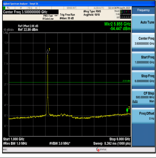
Band41-20MHz-16QAM-40620-100RB#0-Range2:1000~6000MHz
