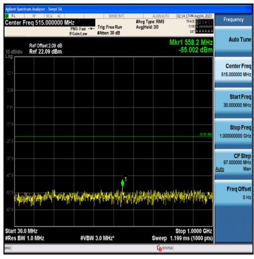
Band41-20MHz-QPSK-40620-100RB#0-Range1:30~1000MHz
