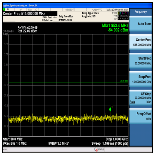
Band38-20MHz-16QAM-37850-100RB#0-Range1:30~1000MHz
