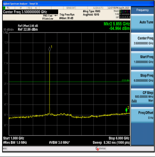
Band41-5MHz-16QAM-41565-25RB#0-Range2:1000~6000MHz
