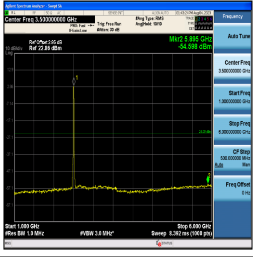
Band41-15MHz-QPSK-39725-75RB#0-Range2:1000~6000MHz
