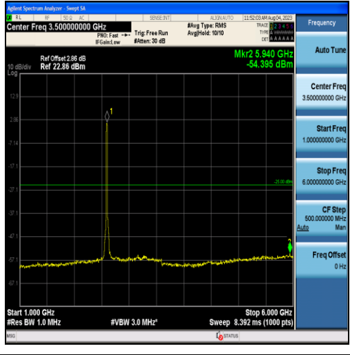
Band38-20MHz-16QAM-38000-100RB#0-Range2:1000~6000MHz
