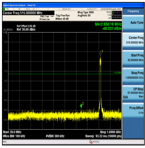
Band26-10MHz-16QAM-26740-50RB#0-Range1:30~1000MHz
