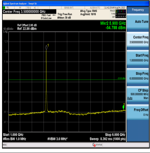
Band38-15MHz-16QAM-38175-75RB#0-Range2:1000~6000MHz
