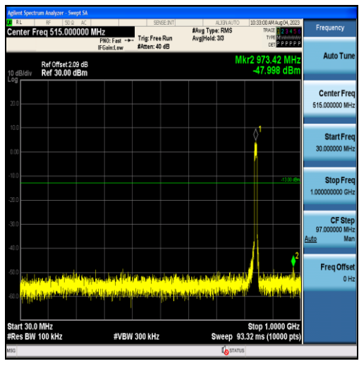
Band26-10MHz-16QAM-26990-50RB#0-Range1:30~1000MHz
