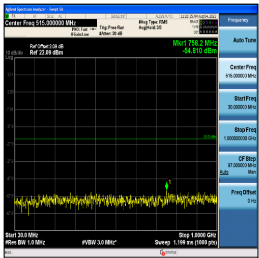
Band38-10MHz-16QAM-38000-50RB#0-Range1:30~1000MHz
