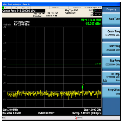
Band38-10MHz-QPSK-37800-50RB#0-Range1:30~1000MHz
