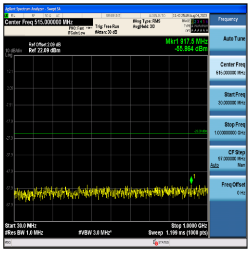
Band38-15MHz-16QAM-38175-75RB#0-Range1:30~1000MHz
