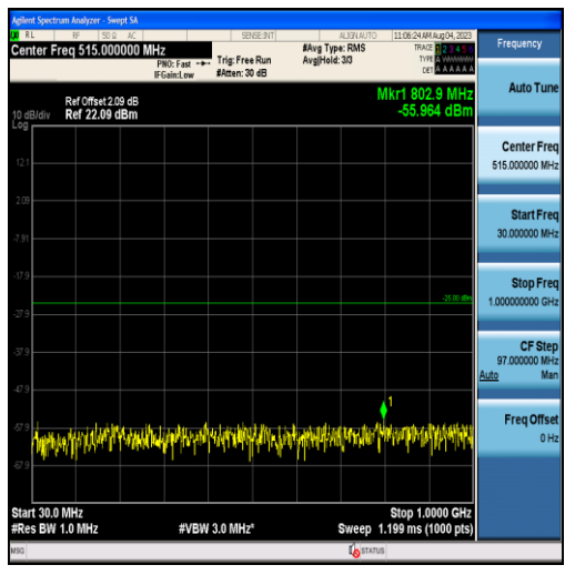
Band38-5MHz-QPSK-38000-25RB#0-Range1:30~1000MHz
