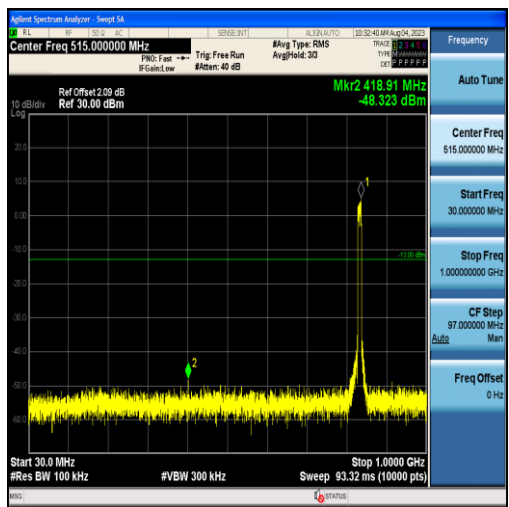
Band26-10MHz-16QAM-26915-50RB#0-Range1:30~1000MHz
