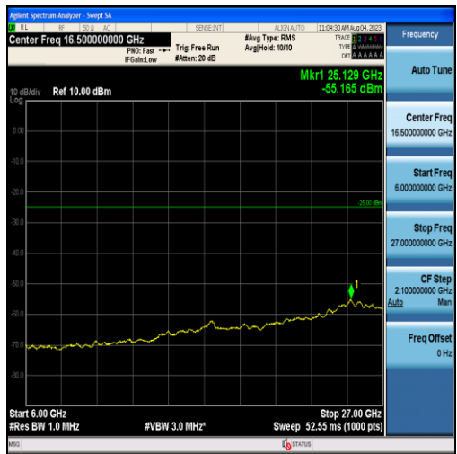
Band38-5MHz-QPSK-37775-25RB#0-Range3:6000~27000MHz
