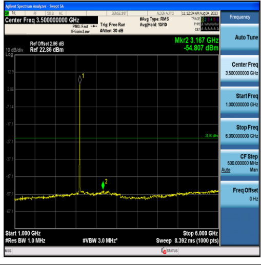
Band38-5MHz-16QAM-38000-25RB#0-Range2:1000~6000MHz
