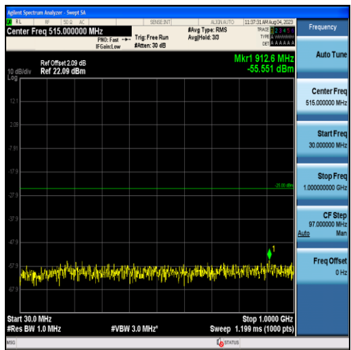
Band38-15MHz-QPSK-37825-75RB#0-Range1:30~1000MHz
