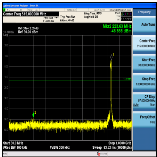
Band26-10MHz-QPSK-26915-50RB#0-Range1:30~1000MHz
