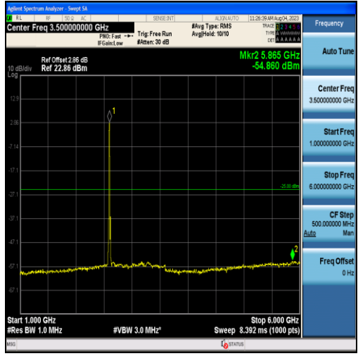
Band38-10MHz-16QAM-38000-50RB#0-Range2:1000~6000MHz
