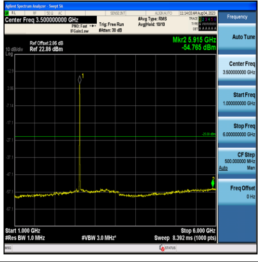
Band38-5MHz-16QAM-38225-25RB#0-Range2:1000~6000MHz
