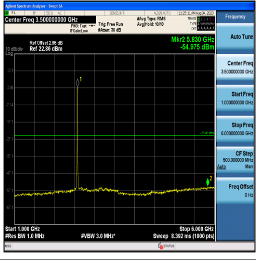
Band38-10MHz-16QAM-37800-50RB#0-Range2:1000~6000MHz
