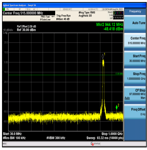
Band26-15MHz-QPSK-26865-75RB#0-Range1:30~1000MHz
