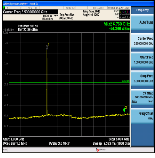
Band38-5MHz-16QAM-37775-25RB#0-Range2:1000~6000MHz
