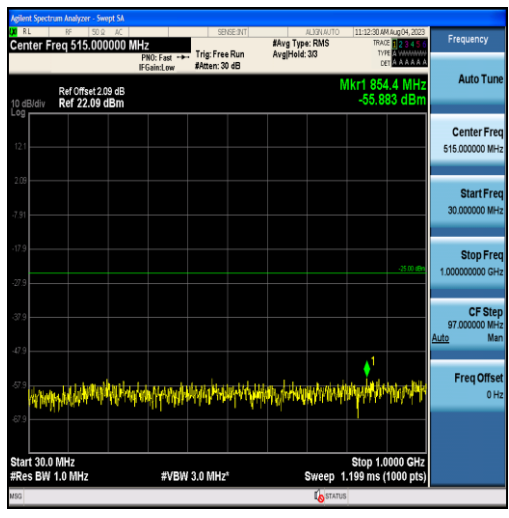
Band38-5MHz-16QAM-38000-25RB#0-Range1:30~1000MHz
