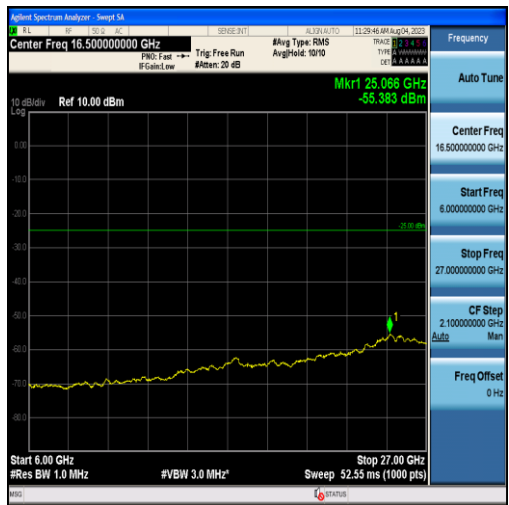
Band38-10MHz-16QAM-38200-50RB#0-Range3:6000~27000MHz
