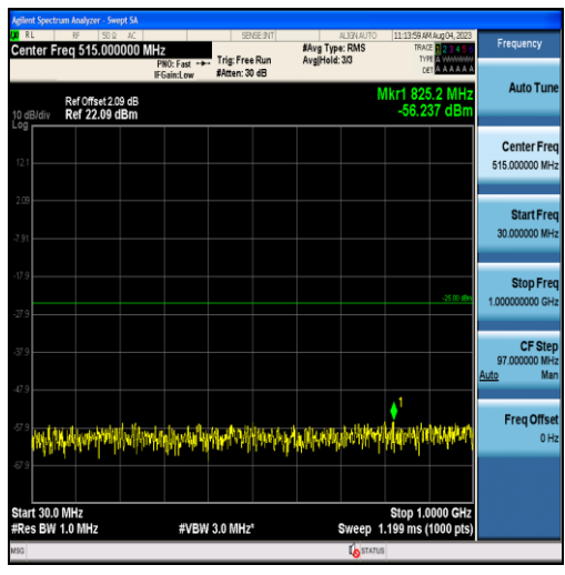
Band38-5MHz-16QAM-38225-25RB#0-Range1:30~1000MHz
