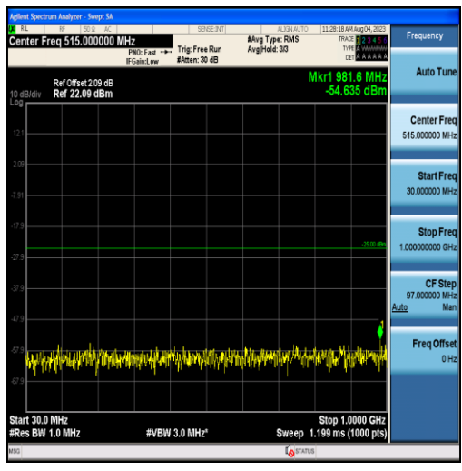
Band38-10MHz-QPSK-38200-50RB#0-Range1:30~1000MHz
