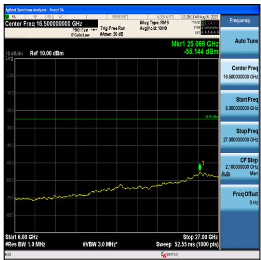
Band38-10MHz-16QAM-38000-50RB#0-Range3:6000~27000MHz
