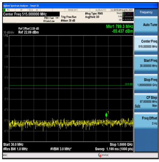
Band38-15MHz-16QAM-37825-75RB#0-Range1:30~1000MHz
