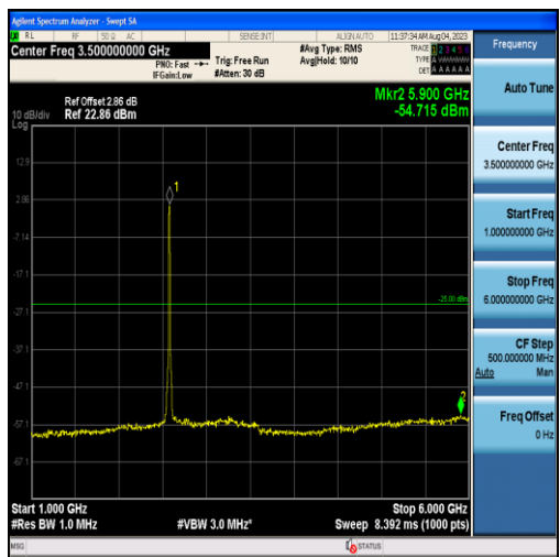
Band38-15MHz-QPSK-37825-75RB#0-Range2:1000~6000MHz
