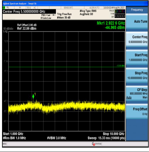
Band26-10MHz-16QAM-26740-50RB#0-Range2:1000~10000MHz
