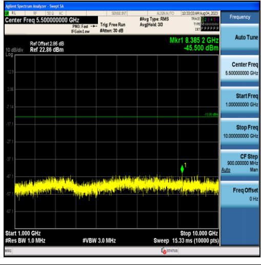
Band26-10MHz-16QAM-26990-50RB#0-Range2:1000~10000MHz
