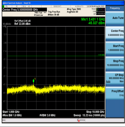
Band26-15MHz-QPSK-26865-75RB#0-Range2:1000~10000MHz
