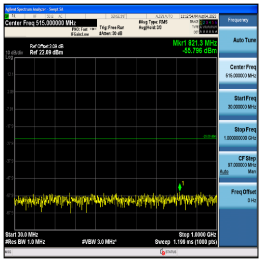
Band38-5MHz-QPSK-38225-25RB#0-Range1:30~1000MHz
