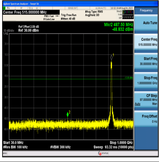
Band26-10MHz-16QAM-26840-50RB#0-Range1:30~1000MHz
