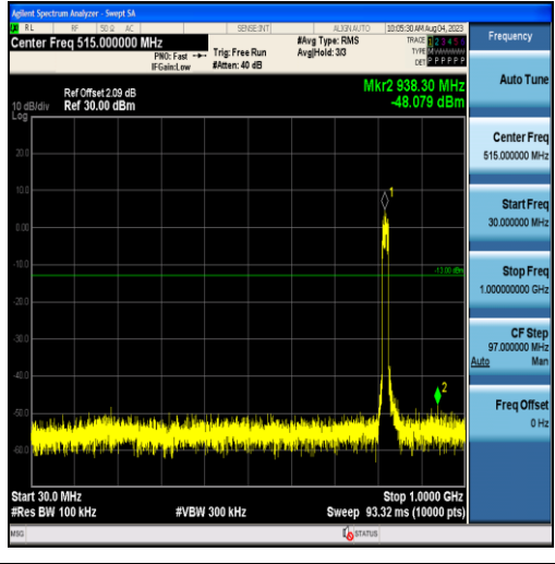
Band26-15MHz-16QAM-26765-75RB#0-Range1:30~1000MHz
