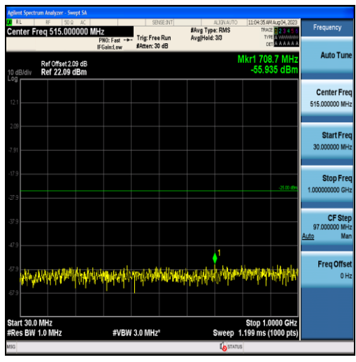
Band38-5MHz-16QAM-37775-25RB#0-Range1:30~1000MHz
