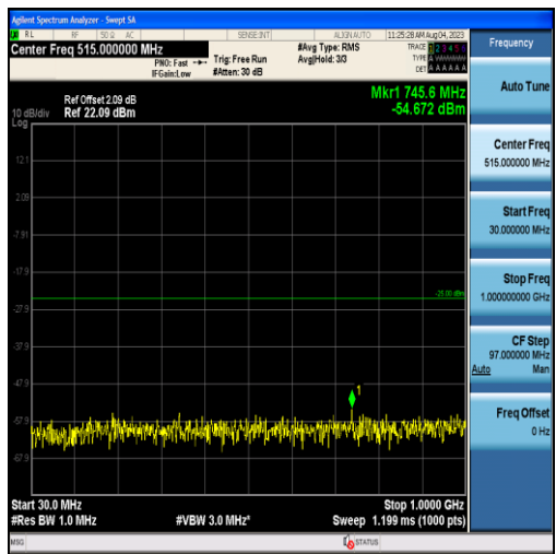
Band38-10MHz-QPSK-38000-50RB#0-Range1:30~1000MHz
