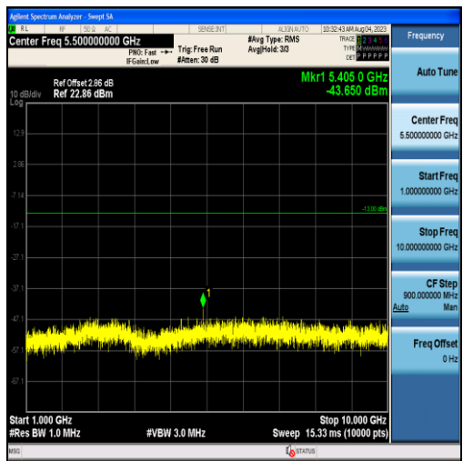
Band26-10MHz-16QAM-26915-50RB#0-Range2:1000~10000MHz
