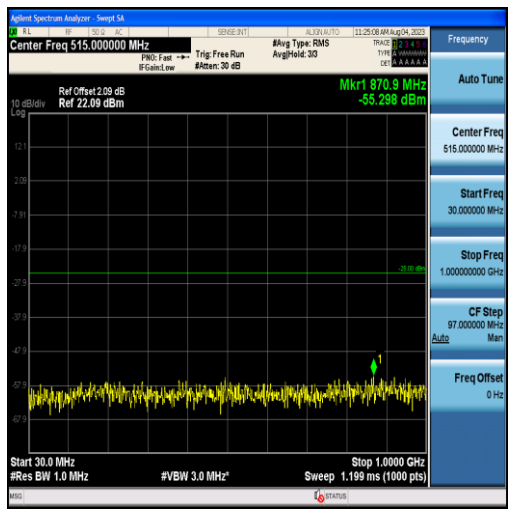
Band38-10MHz-16QAM-37800-50RB#0-Range1:30~1000MHz
