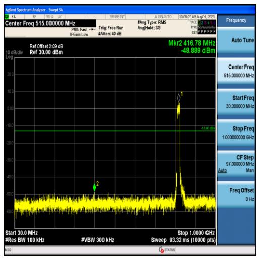
Band26-15MHz-QPSK-26765-75RB#0-Range1:30~1000MHz
