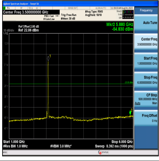
Band38-15MHz-16QAM-37825-75RB#0-Range2:1000~6000MHz
