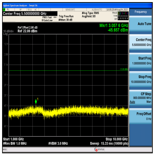
Band26-15MHz-QPSK-26765-75RB#0-Range2:1000~10000MHz
