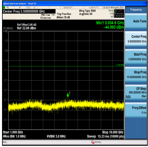
Band26-3MHz-16QAM-26805-15RB#0-Range2:1000~10000MHz
