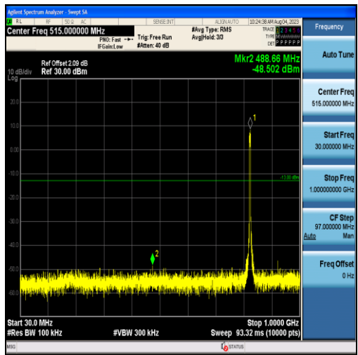
Band26-5MHz-QPSK-26815-25RB#0-Range1:30~1000MHz
