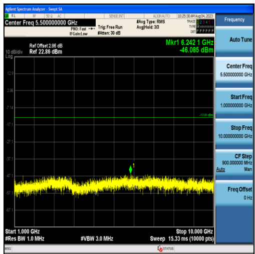
Band26-5MHz-16QAM-27015-25RB#0-Range2:1000~10000MHz
