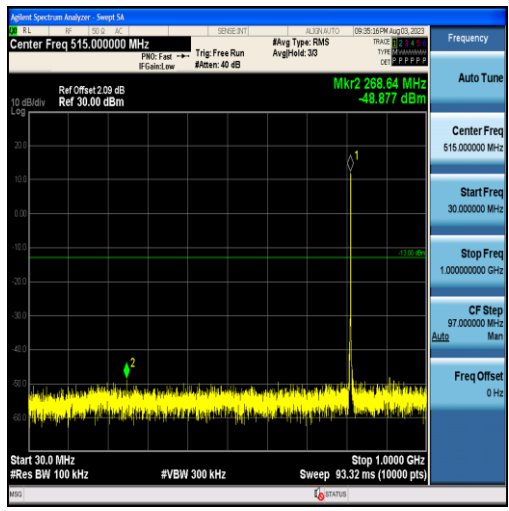
Band26-1.4MHz-QPSK-26697-6RB#0-Range1:30~1000MHz
