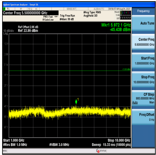
Band26-5MHz-16QAM-26715-25RB#0-Range2:1000~10000MHz
