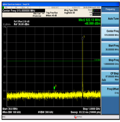
Band26-1.4MHz-16QAM-26697-6RB#0-Range1:30~1000MHz
