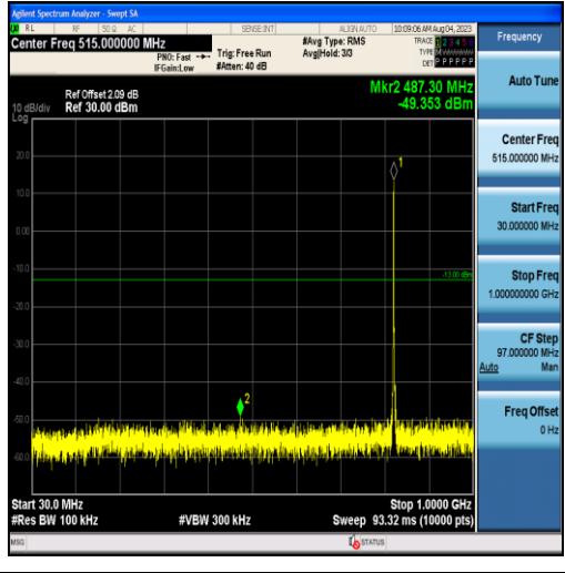
Band26-1.4MHz-QPSK-26797-6RB#0-Range1:30~1000MHz
