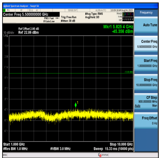
Band26-1.4MHz-16QAM-26797-6RB#0-Range2:1000~10000MHz
