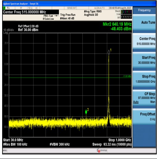
Band26-3MHz-16QAM-26740-15RB#0-Range1:30~1000MHz
