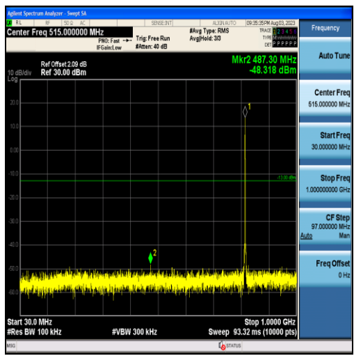
Band26-1.4MHz-QPSK-26740-6RB#0-Range1:30~1000MHz
