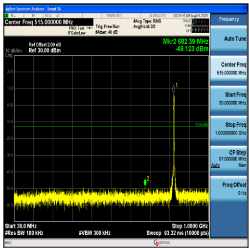
Band26-5MHz-16QAM-26815-25RB#0-Range1:30~1000MHz
