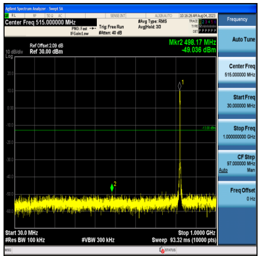
Band26-3MHz-QPSK-26805-15RB#0-Range1:30~1000MHz
