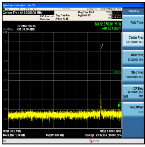
Band26-1.4MHz-QPSK-26783-6RB#0-Range 1:30~1000MHz
