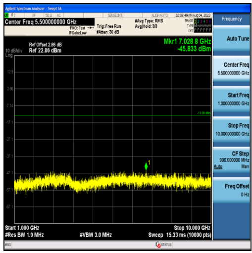
Band26-1.4MHz-QPSK-27033-6RB#0-Range2:1000~10000MHz
