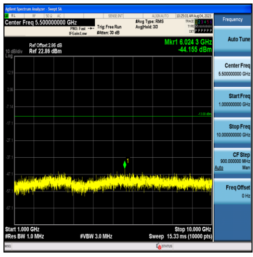
Band26-5MHz-QPSK-26915-25RB#0-Range2:1000~10000MHz
