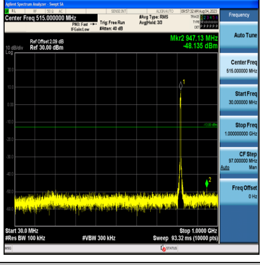
Band26-5MHz-16QAM-26765-25RB#0-Range1:30~1000MHz
