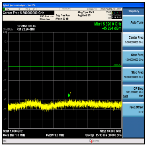
Band26-1.4MHz-16QAM-27033-6RB#0-Range2:1000~10000MHz
