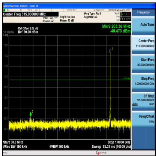
Band26-1.4MHz-QPSK-26915-6RB#0-Range1:30~1000MHz
