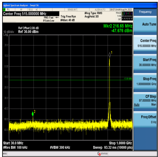
Band26-5MHz-QPSK-26740-25RB#0-Range1:30~1000MHz
