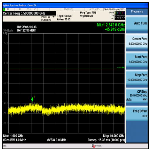
Band26-3MHz-16QAM-26775-15RB#0-Range2:1000~10000MHz
