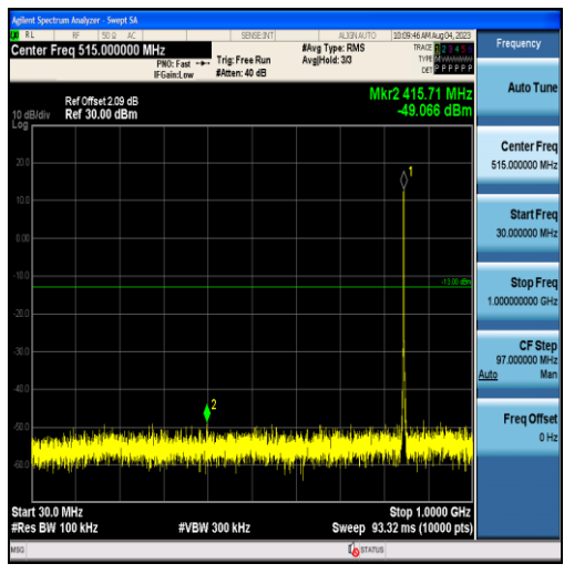
Band26-1.4MHz-QPSK-27033-6RB#0-Range 1:30~1000MHz
