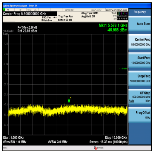
Band26-5MHz-QPSK-26815-25RB#0-Range2:1000~10000MHz
