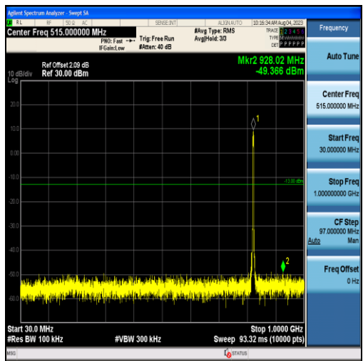
Band26-3MHz-16QAM-26805-15RB#0-Range1:30~1000MHz
