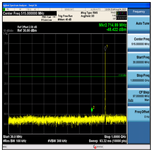
Band26-1.4MHz-16QAM-26797-6RB#0-Range1:30~1000MHz
