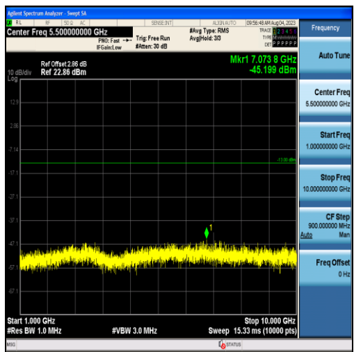
Band26-5MHz-QPSK-26715-25RB#0-Range2:1000~10000MHz
