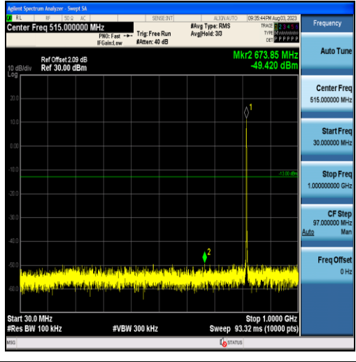
Band26-1.4MHz-16QAM-26740-6RB#0-Range1:30~1000MHz
