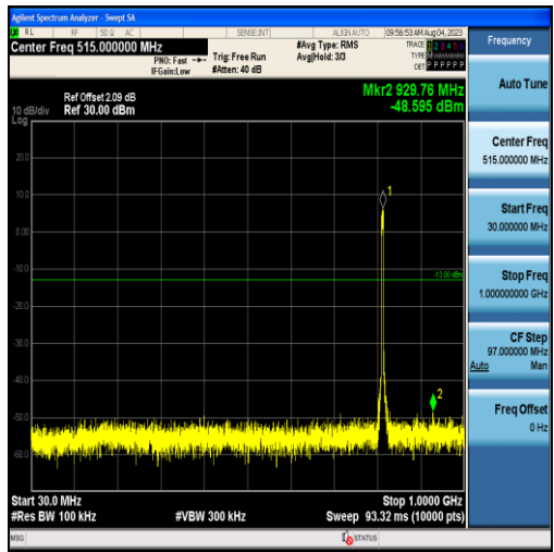
Band26-5MHz-16QAM-26715-25RB#0-Range1:30~1000MHz
