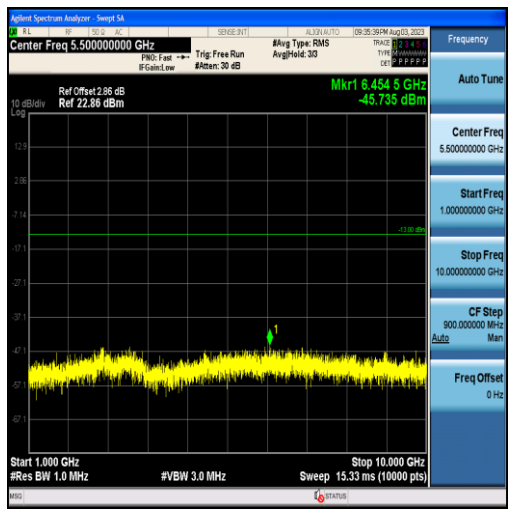
Band26-1.4MHz-QPSK-26740-6RB#0-Range2:1000~10000MHz
