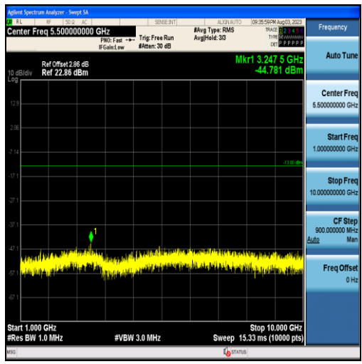
Band26-1.4MHz-QPSK-26783-6RB#0-Range2:1000~10000MHz
