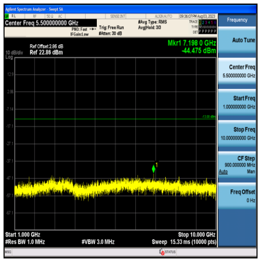
Band26-1.4MHz-16QAM-26783-6RB#0-Range2:1000~10000MHz
