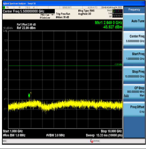
Band26-3MHz-16QAM-26705-15RB#0-Range2:1000~10000MHz
