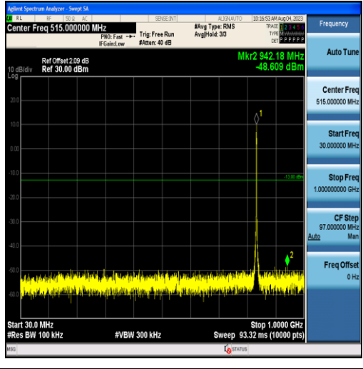
Band26-3MHz-16QAM-26915-15RB#0-Range1:30~1000MHz
