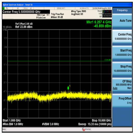
Band26-1.4MHz-QPSK-26915-6RB#0-Range2:1000~10000MHz
