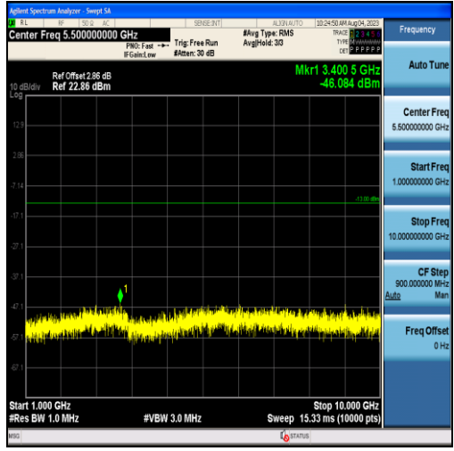
Band26-5MHz-16QAM-26815-25RB#0-Range2:1000~10000MHz
