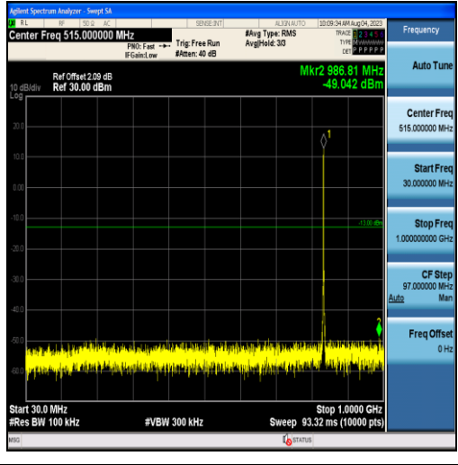
Band26-1.4MHz-16QAM-26915-6RB#0-Range1:30~1000MHz
