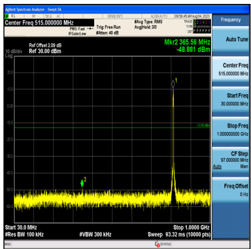
Band26-5MHz-QPSK-26715-25RB#0-Range1:30~1000MHz
