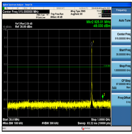
Band26-3MHz-QPSK-26775-15RB#0-Range1:30~1000MHz
