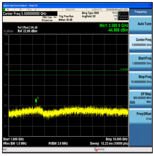
Band26-3MHz-QPSK-26740-15RB#0-Range2:1000~10000MHz
