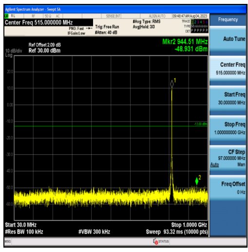
Band26-3MHz-QPSK-26740-15RB#0-Range1:30~1000MHz
