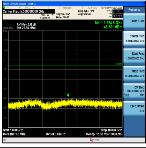
Band26-3MHz-16QAM-26740-15RB#0-Range2:1000~10000MHz
