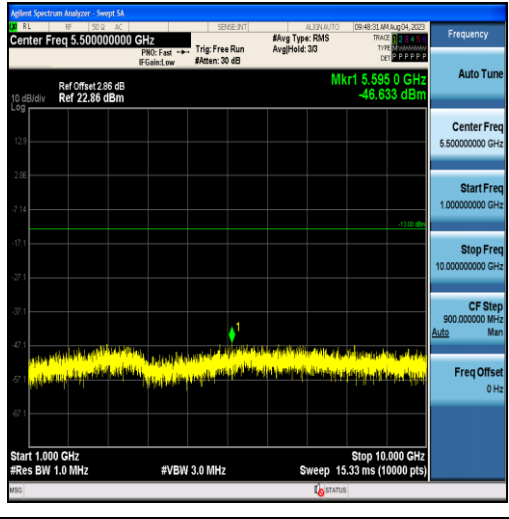
Band26-3MHz-QPSK-26705-15RB#0-Range2:1000~10000MHz
