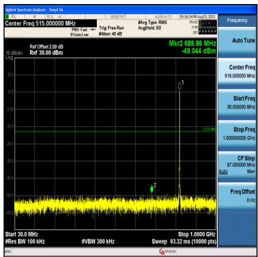
Band26-1.4MHz-16QAM-26783-6RB#0-Range1:30~1000MHz
