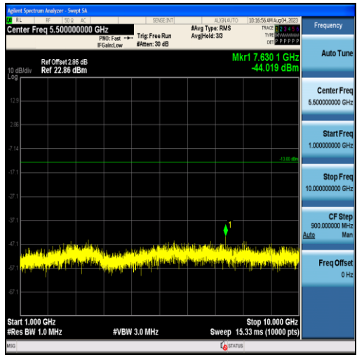
Band26-3MHz-16QAM-26915-15RB#0-Range2:1000~10000MHz
