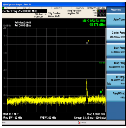
Band26-3MHz-16QAM-26705-15RB#0-Range1:30~1000MHz
