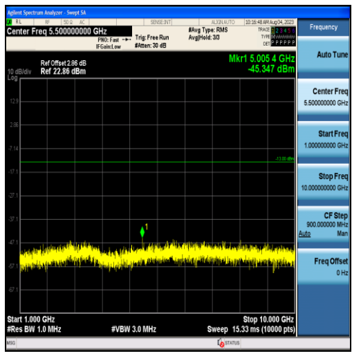
Band26-3MHz-QPSK-26915-15RB#0-Range2:1000~10000MHz
