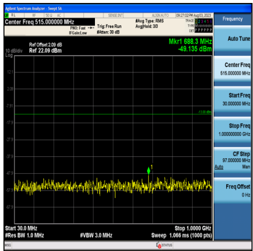
Band25-20MHz-16QAM-26365-100RB#0-Range1:30~1000MHz
