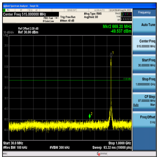
Band26-5MHz-QPSK-26915-25RB#0-Range1:30~1000MHz
