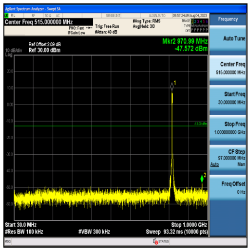
Band26-5MHz-QPSK-26765-25RB#0-Range1:30~1000MHz
