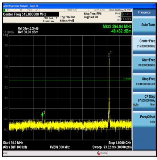
Band26-3MHz-16QAM-26775-15RB#0-Range1:30~1000MHz
