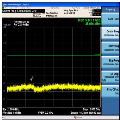
Band26-3MHz-QPSK-26805-15RB#0-Range2:1000~10000MHz
