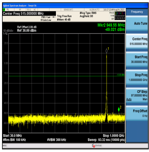
Band26-3MHz-16QAM-27025-15RB#0-Range1:30~1000MHz
