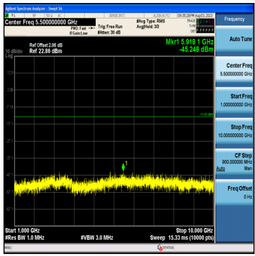
Band26-1.4MHz-16QAM-26697-6RB#0-Range2:1000~10000MHz
