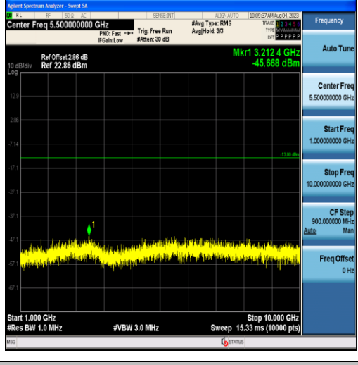
Band26-1.4MHz-16QAM-26915-6RB#0-Range2:1000~10000MHz
