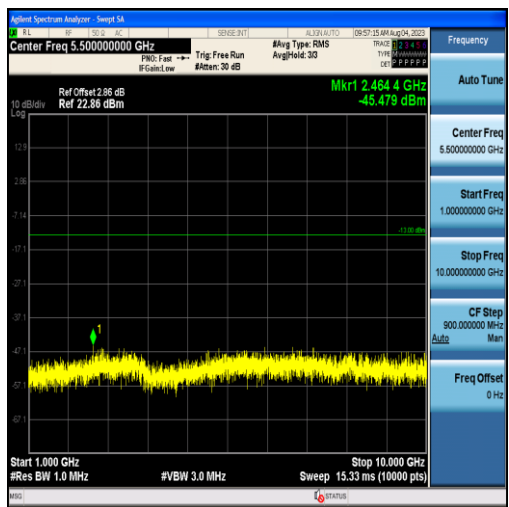
Band26-5MHz-16QAM-26740-25RB#0-Range2:1000~10000MHz
