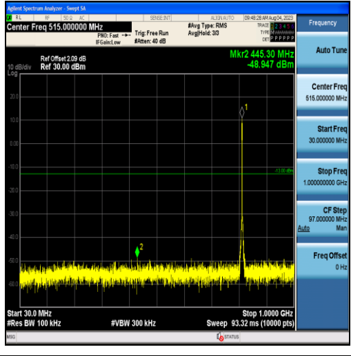
Band26-3MHz-QPSK-26705-15RB#0-Range1:30~1000MHz
