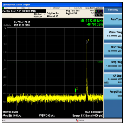
Band26-3MHz-QPSK-26915-15RB#0-Range1:30~1000MHz
