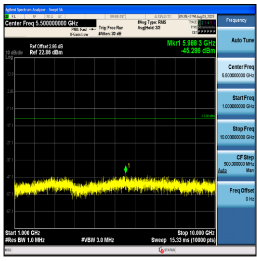
Band26-1.4MHz-16QAM-26740-6RB#0-Range2:1000~10000MHz
