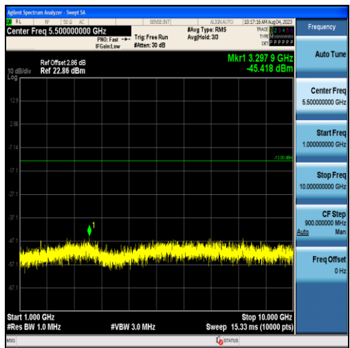
Band26-3MHz-16QAM-27025-15RB#0-Range2:1000~10000MHz
