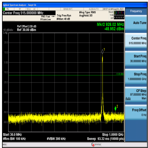
Band26-5MHz-16QAM-26740-25RB#0-Range1:30~1000MHz
