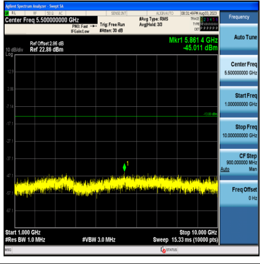
Band13-5MHz-16QAM-23230-25RB#0-Range2:1000~10000MHz
