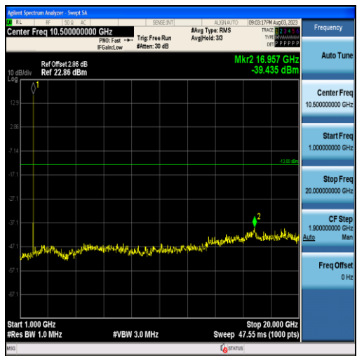
Band25-5MHz-16QAM-26665-25RB#0-Range2:1000~20000MHz
