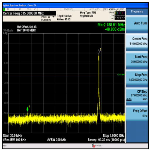
Band13-5MHz-16QAM-23230-25RB#0-Range1:30~1000MHz
