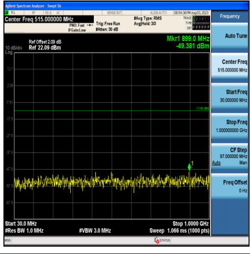
Band25-3MHz-16QAM-26365-15RB#0-Range1:30~1000MHz
