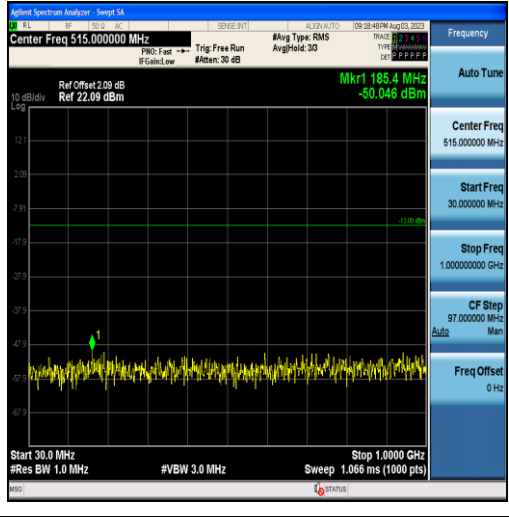
Band25-15MHz-16QAM-26365-75RB#0-Range1:30~1000MHz
