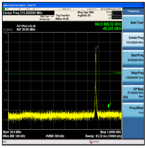
Band13-5MHz-QPSK-23205-25RB#0-Range1:30~1000MHz
