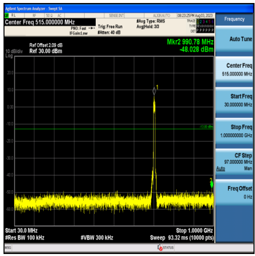
Band12-10MHz-16QAM-23130-50RB#0-Range1:30~1000MHz
