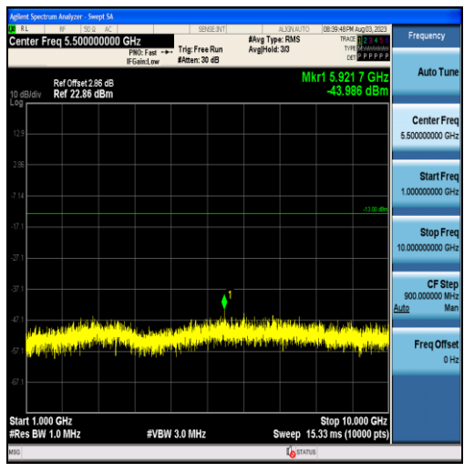
Band13-10MHz-16QAM-23230-50RB#0-Range2:1000~10000MHz
