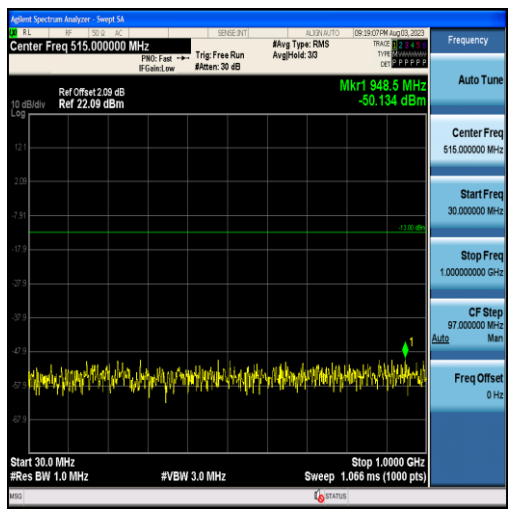
Band25-15MHz-16QAM-26615-75RB#0-Range1:30~1000MHz
