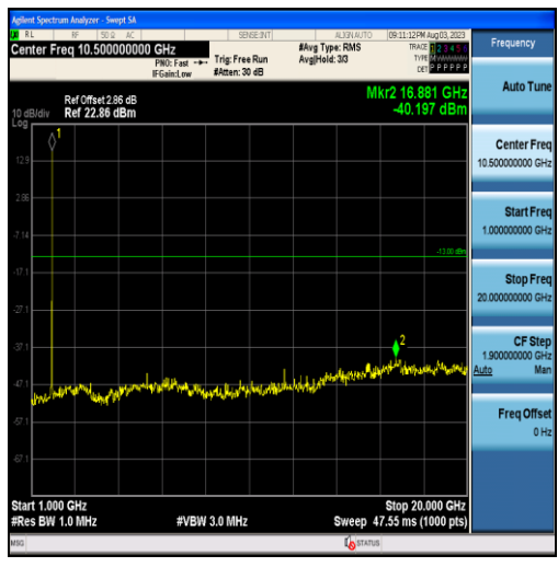
Band25-10MHz-16QAM-26640-50RB#0-Range2:1000~20000MHz
