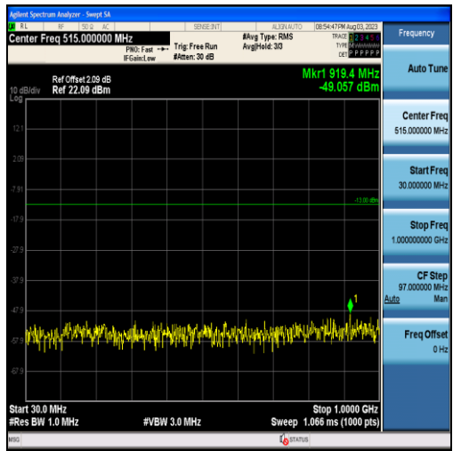
Band25-3MHz-QPSK-26675-15RB#0-Range1:30~1000MHz
