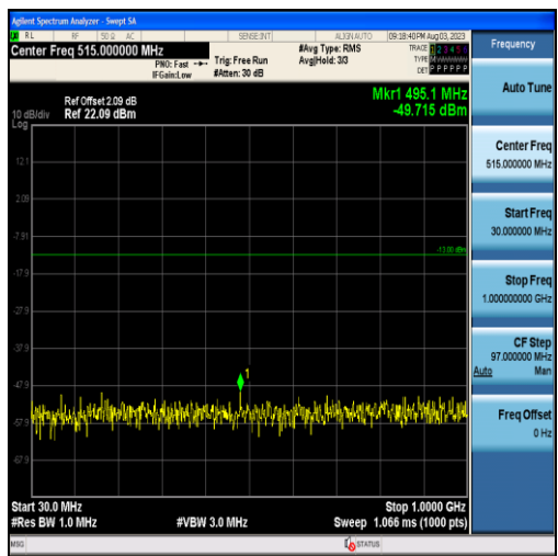
Band25-15MHz-QPSK-26365-75RB#0-Range1:30~1000MHz
