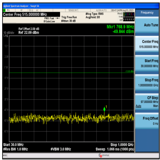
Band25-1.4MHz-16QAM-26683-6RB#0-Range1:30~1000MHz
