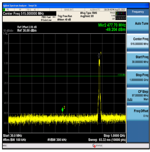
Band13-10MHz-16QAM-23230-50RB#0-Range1:30~1000MHz
