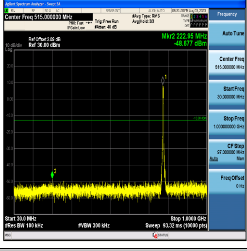
Band13-5MHz-16QAM-23205-25RB#0-Range1:30~1000MHz
