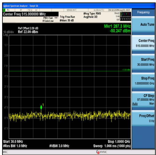
Band25-10MHz-QPSK-26090-50RB#0-Range1:30~1000MHz
