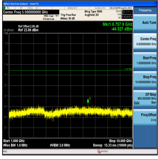
Band12-10MHz-16QAM-23095-50RB#0-Range2:1000~10000MHz
