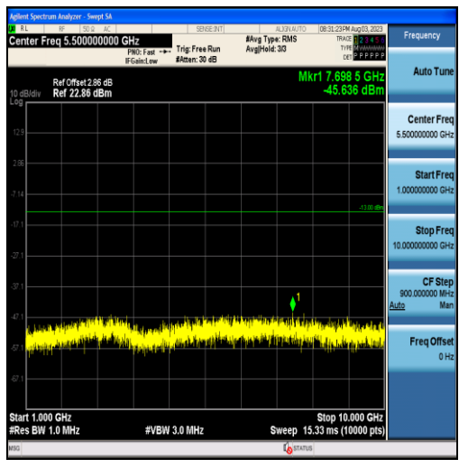
Band13-5MHz-16QAM-23205-25RB#0-Range2:1000~10000MHz
