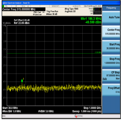
Band25-1.4MHz-16QAM-26365-6RB#0-Range1:30~1000MHz
