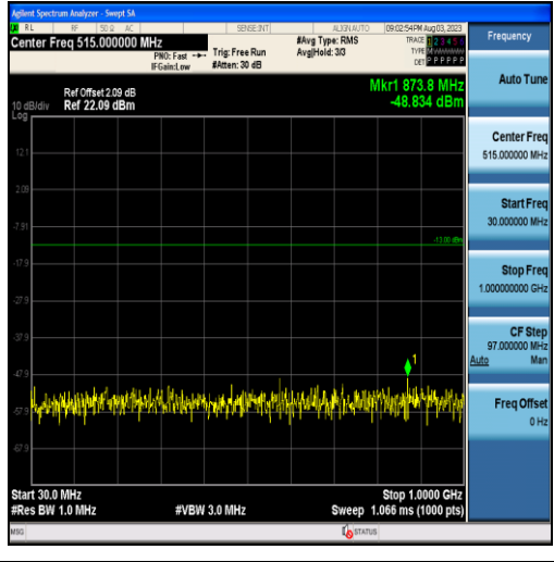
Band25-5MHz-16QAM-26365-25RB#0-Range1:30~1000MHz
