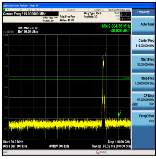
Band13-10MHz-QPSK-23230-50RB#0-Range1:30~1000MHz
