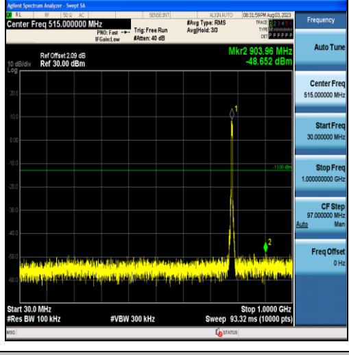
Band13-5MHz-QPSK-23255-25RB#0-Range1:30~1000MHz
