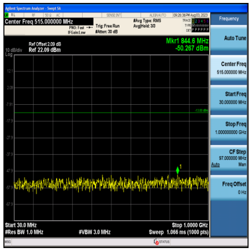
Band25-20MHz-QPSK-26140-100RB#0-Range1:30~1000MHz
