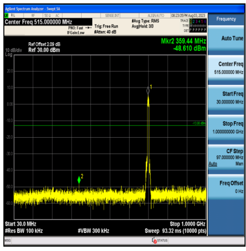
Band12-10MHz-16QAM-23095-50RB#0-Range1:30~1000MHz
