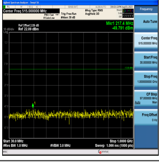
Band25-5MHz-16QAM-26665-25RB#0-Range1:30~1000MHz
