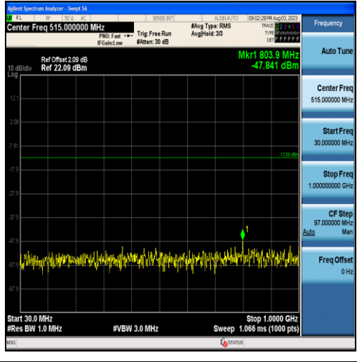
Band25-5MHz-QPSK-26065-25RB#0-Range1:30~1000MHz
