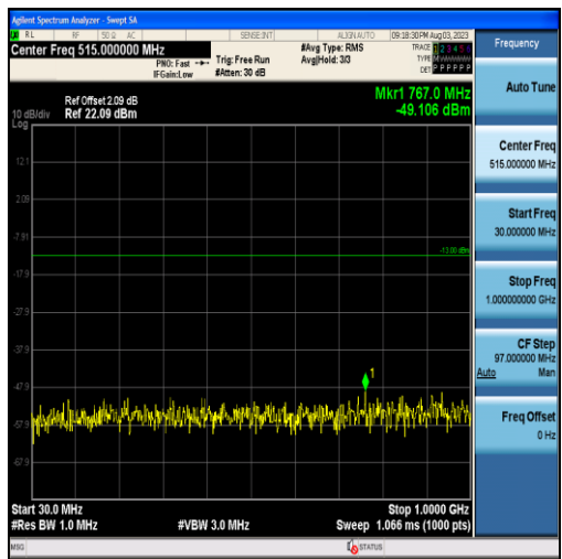
Band25-15MHz-16QAM-26115-75RB#0-Range1:30~1000MHz
