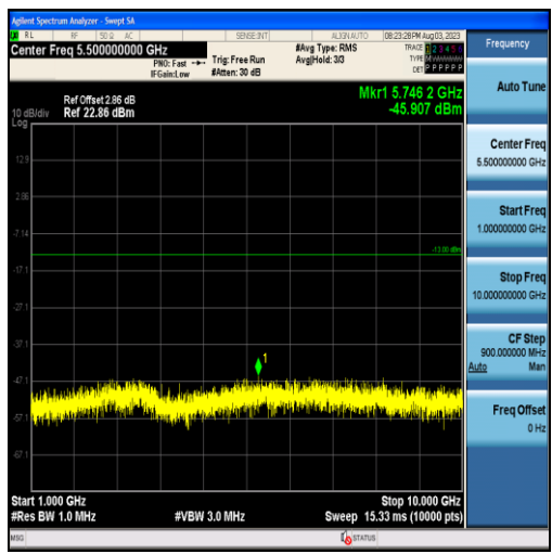
Band12-10MHz-16QAM-23130-50RB#0-Range2:1000~10000MHz
