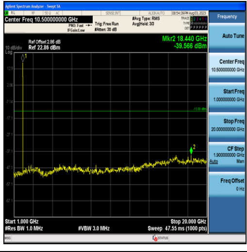
Band25-3MHz-16QAM-26365-15RB#0-Range2:1000~20000MHz
