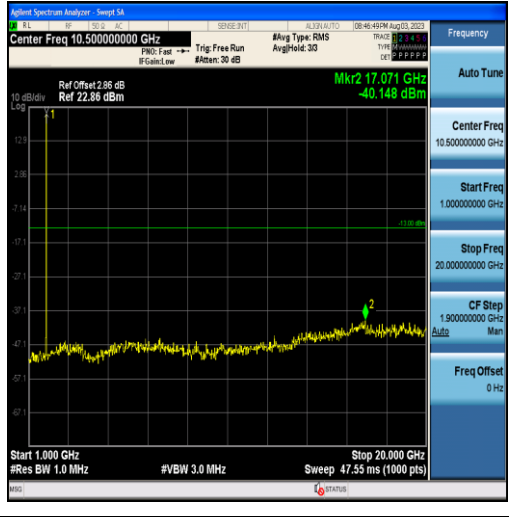
Band25-1.4MHz-16QAM-26047-6RB#0-Range2:1000~20000MHz
