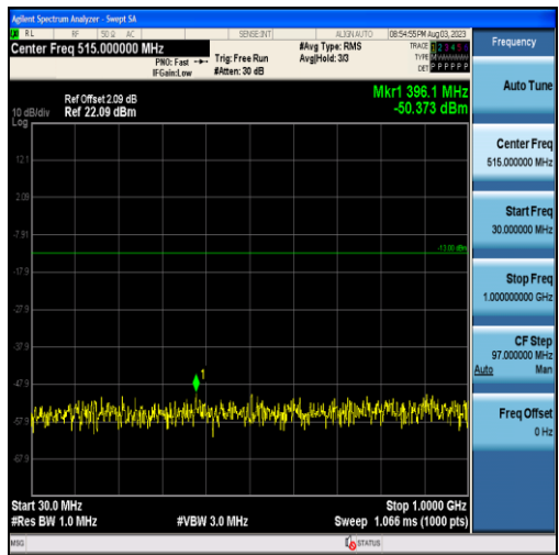
Band25-3MHz-16QAM-26675-15RB#0-Range1:30~1000MHz
