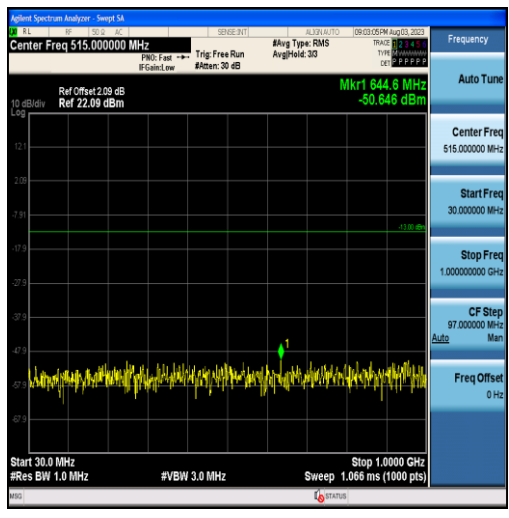
Band25-5MHz-QPSK-26665-25RB#0-Range1:30~1000MHz
