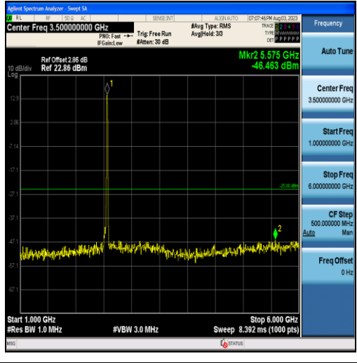
Band7-15MHz-QPSK-21375-75RB#0-Range2:1000~6000MHz
