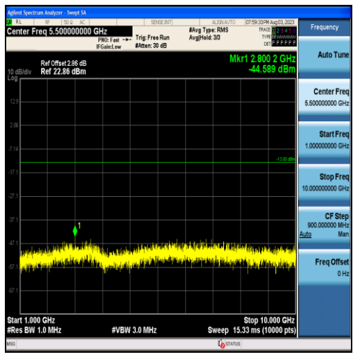
Band12-1.4MHz-16QAM-23017-6RB#0-Range2:1000~10000MHz
