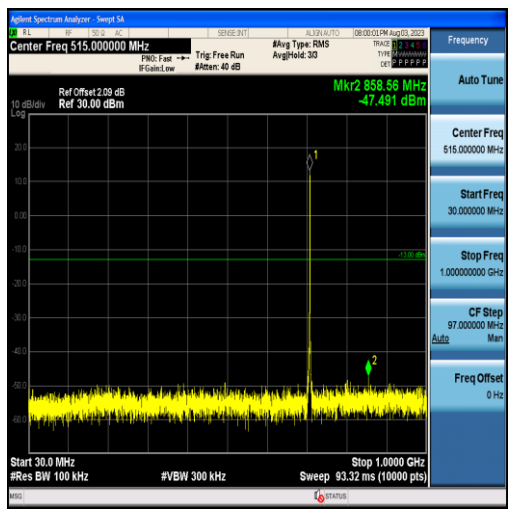
Band12-1.4MHz-QPSK-23173-6RB#0-Range1:30~1000MHz
