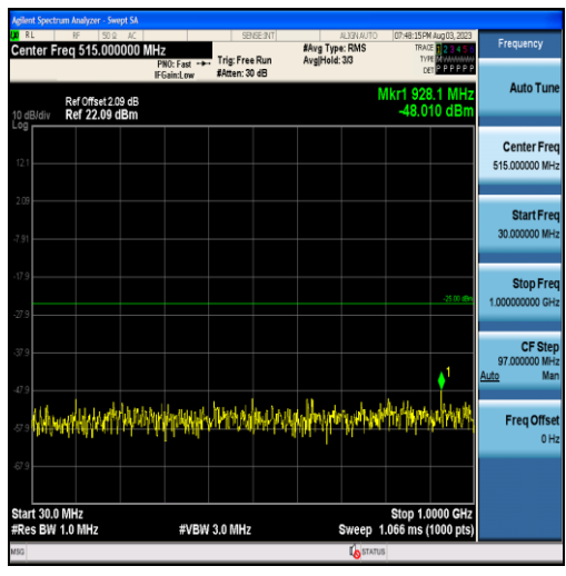
Band7-20MHz-QPSK-21100-100RB#0-Range1:30~1000MHz
