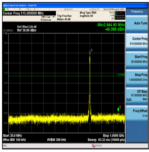
Band12-5MHz-16QAM-23095-25RB#0-Range1:30~1000MHz
