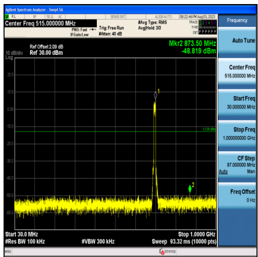
Band12-10MHz-16QAM-23060-50RB#0-Range1:30~1000MHz
