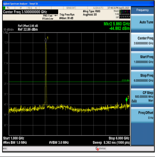
Band7-20MHz-16QAM-21100-100RB#0-Range2:1000~6000MHz
