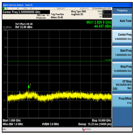
Band12-1.4MHz-QPSK-23095-6RB#0-Range2:1000~10000MHz
