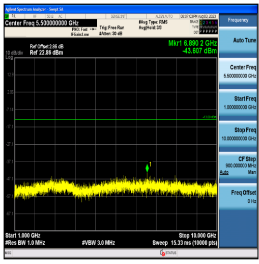
Band12-3MHz-16QAM-23025-15RB#0-Range2:1000~10000MHz
