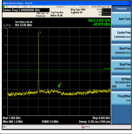
Band7-15MHz-16QAM-20825-75RB#0-Range2:1000~6000MHz
