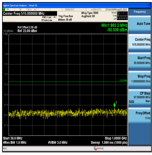
Band7-15MHz-16QAM-20825-75RB#0-Range1:30~1000MHz
