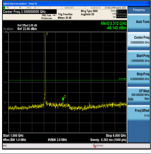
Band7-15MHz-16QAM-21375-75RB#0-Range2:1000~6000MHz
