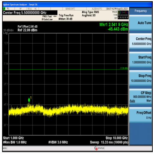
Band12-3MHz-16QAM-23165-15RB#0-Range2:1000~10000MHz
