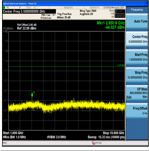
Band12-1.4MHz-16QAM-23095-6RB#0-Range2:1000~10000MHz
