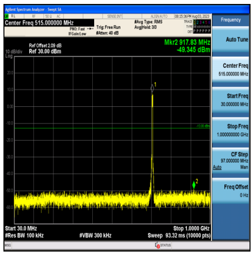
Band12-5MHz-QPSK-23155-25RB#0-Range1:30~1000MHz
