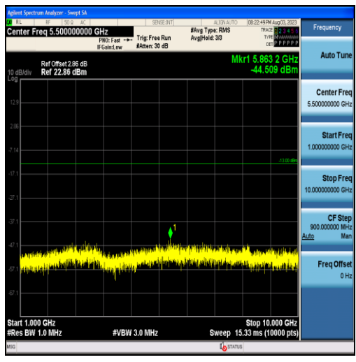
Band12-10MHz-16QAM-23060-50RB#0-Range2:1000~10000MHz
