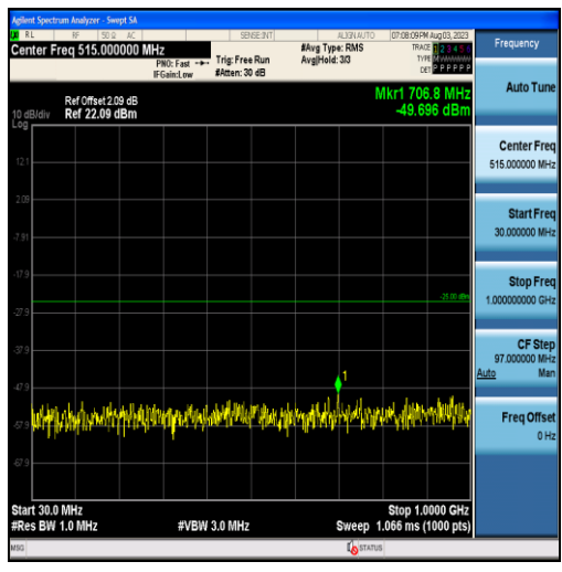
Band7-15MHz-16QAM-21375-75RB#0-Range1:30~1000MHz
