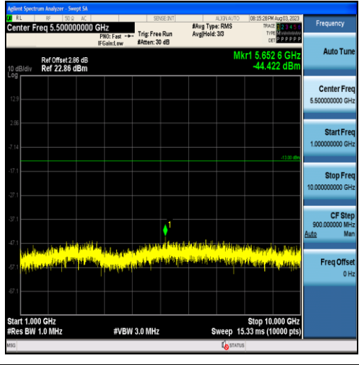
Band12-5MHz-16QAM-23095-25RB#0-Range2:1000~10000MHz
