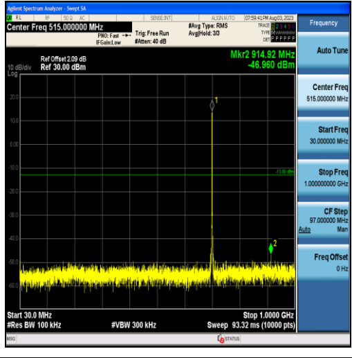
Band12-1.4MHz-QPSK-23095-6RB#0-Range1:30~1000MHz
