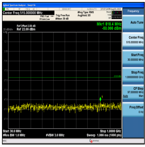
Band7-15MHz-16QAM-21100-75RB#0-Range1:30~1000MHz
