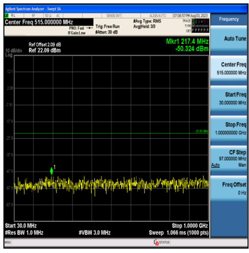
Band7-15MHz-QPSK-21100-75RB#0-Range1:30~1000MHz
