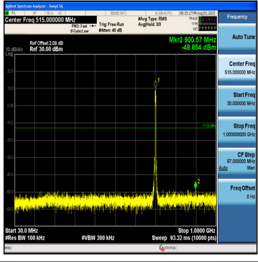
Band12-5MHz-QPSK-23095-25RB#0-Range1:30~1000MHz
