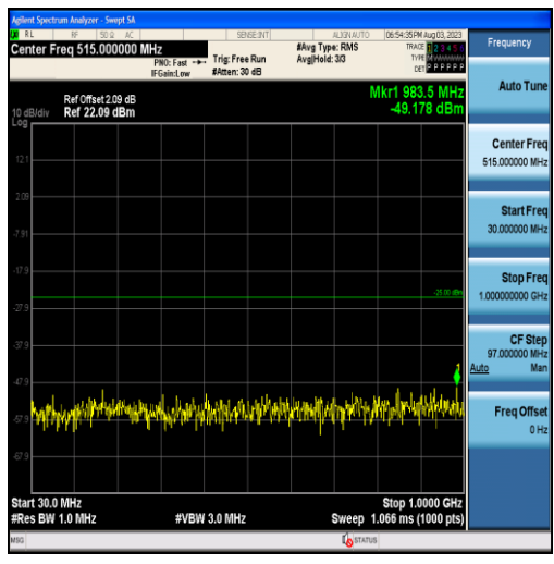
Band7-10MHz-16QAM-21400-50RB#0-Range1:30~1000MHz
