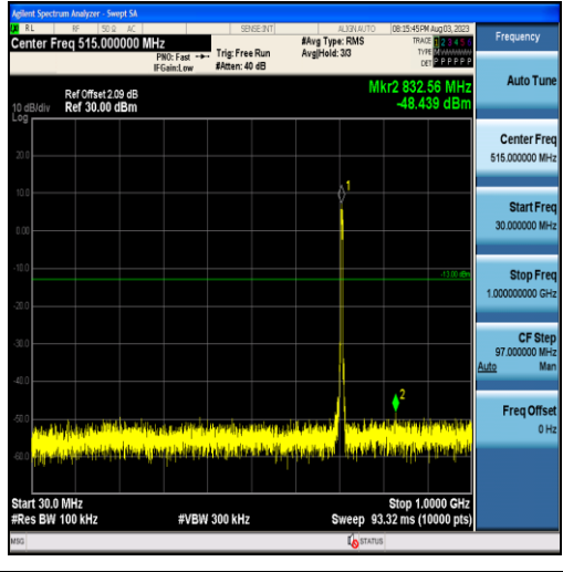
Band12-5MHz-16QAM-23155-25RB#0-Range1:30~1000MHz
