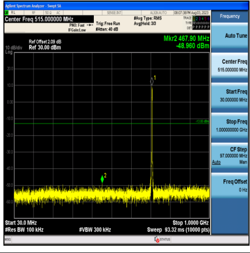
Band12-3MHz-16QAM-23165-15RB#0-Range1:30~1000MHz
