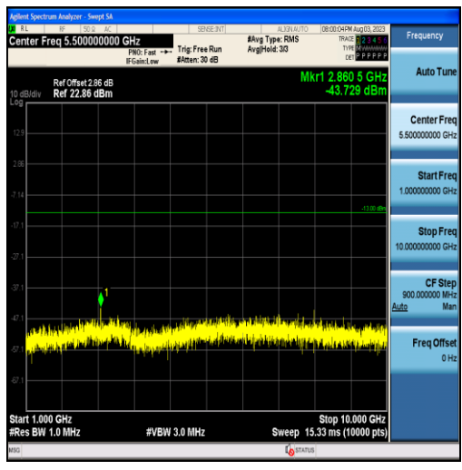
Band12-1.4MHz-QPSK-23173-6RB#0-Range2:1000~10000MHz
