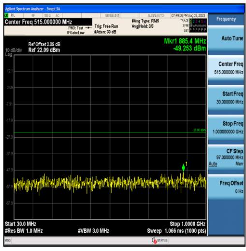
Band7-20MHz-16QAM-21350-100RB#0-Range1:30~1000MHz
