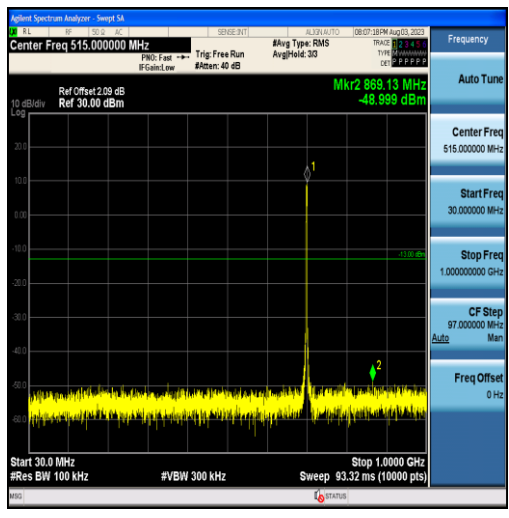
Band12-3MHz-16QAM-23095-15RB#0-Range1:30~1000MHz
