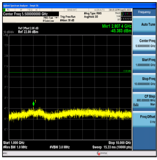
Band12-5MHz-16QAM-23035-25RB#0-Range2:1000~10000MHz
