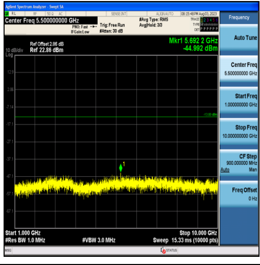
Band12-5MHz-16QAM-23155-25RB#0-Range2:1000~10000MHz
