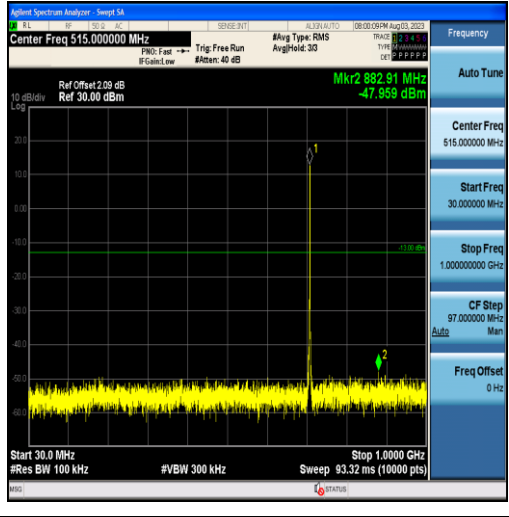
Band12-1.4MHz-16QAM-23173-6RB#0-Range1:30~1000MHz
