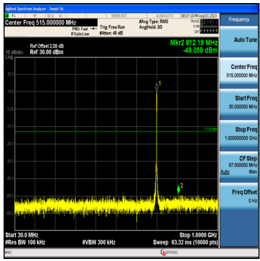
Band12-3MHz-QPSK-23095-15RB#0-Range1:30~1000MHz
