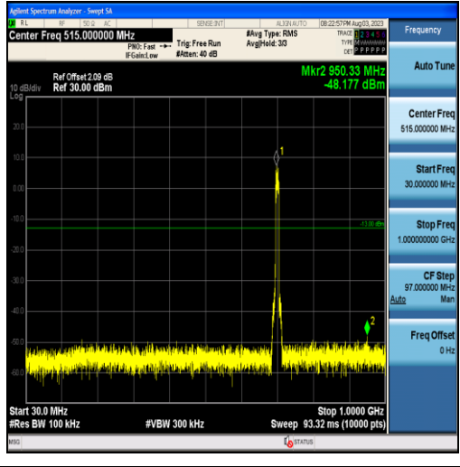
Band12-10MHz-QPSK-23095-50RB#0-Range1:30~1000MHz
