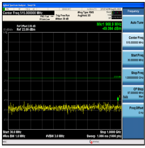
Band7-15MHz-QPSK-21375-75RB#0-Range1:30~1000MHz
