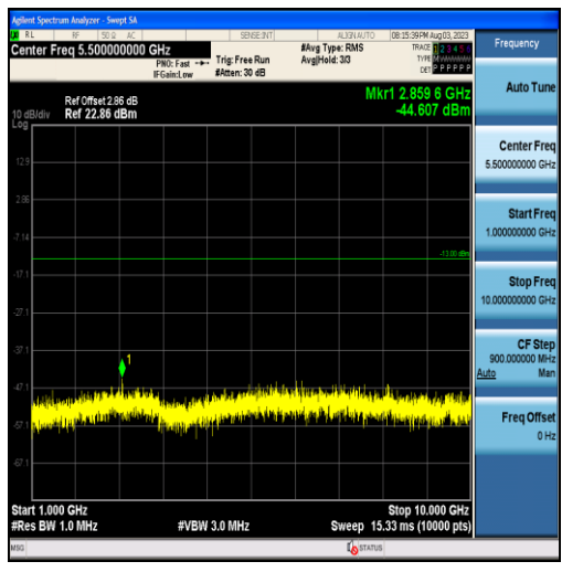
Band12-5MHz-QPSK-23155-25RB#0-Range2:1000~10000MHz
