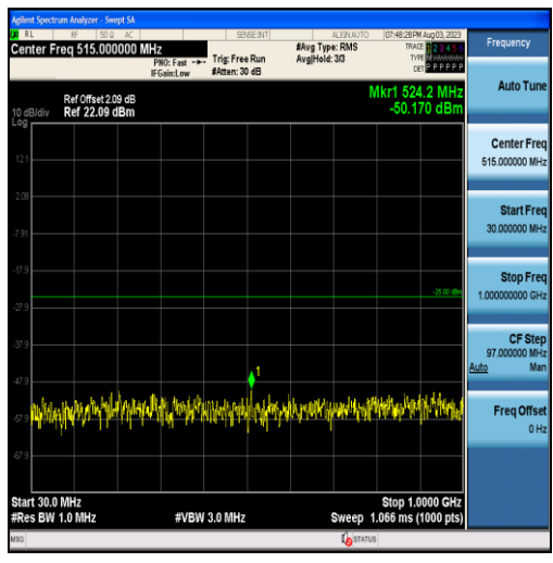
Band7-20MHz-16QAM-21100-100RB#0-Range1:30~1000MHz
