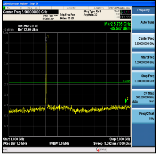
Band7-15MHz-QPSK-21100-75RB#0-Range2:1000~6000MHz
