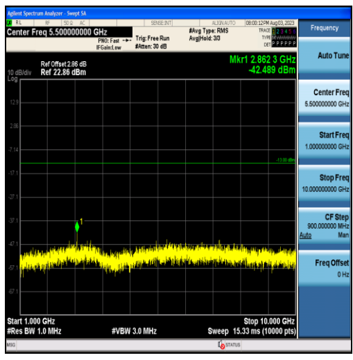
Band12-1.4MHz-16QAM-23173-6RB#0-Range2:1000~10000MHz
