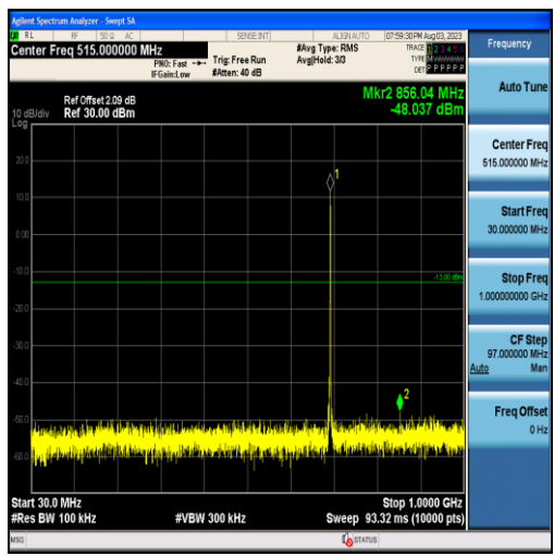
Band12-1.4MHz-16QAM-23017-6RB#0-Range1:30~1000MHz
