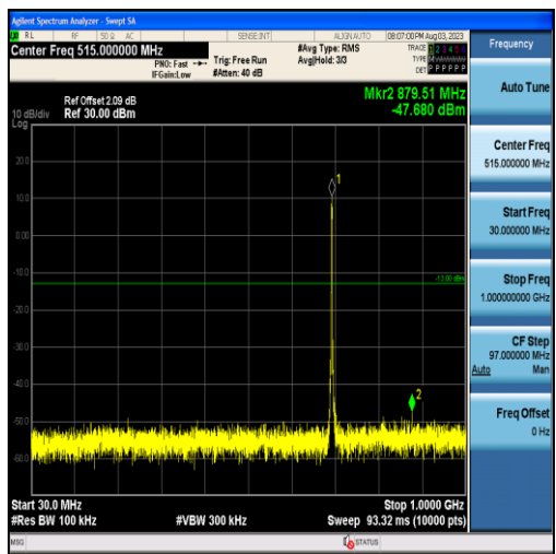
Band12-3MHz-16QAM-23025-15RB#0-Range1:30~1000MHz
