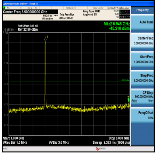
Band7-15MHz-QPSK-20825-75RB#0-Range2:1000~6000MHz
