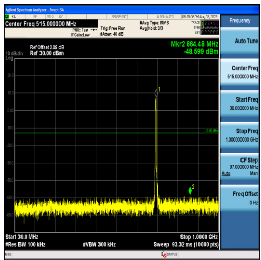
Band12-5MHz-16QAM-23035-25RB#0-Range1:30~1000MHz
