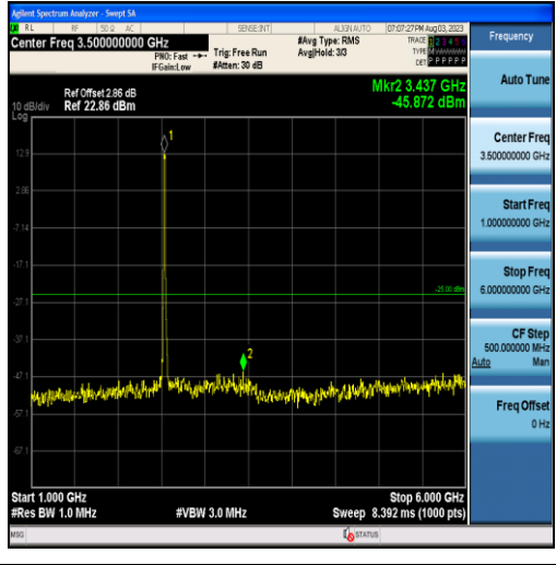
Band7-15MHz-16QAM-21100-75RB#0-Range2:1000~6000MHz
