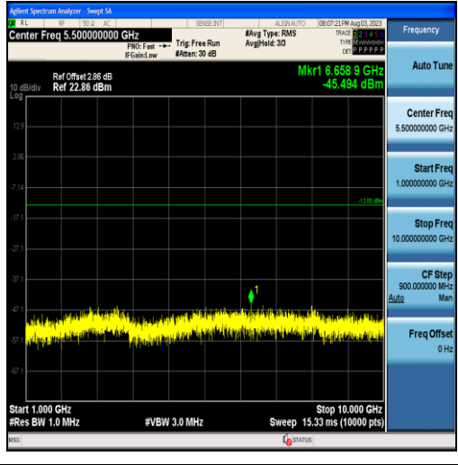
Band12-3MHz-16QAM-23095-15RB#0-Range2:1000~10000MHz
