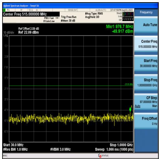
Band7-20MHz-16QAM-20850-100RB#0-Range1:30~1000MHz
