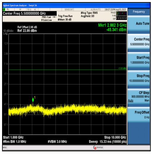
Band12-3MHz-QPSK-23165-15RB#0-Range2:1000~10000MHz
