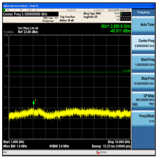
Band12-10MHz-QPSK-23095-50RB#0-Range2:1000~10000MHz
