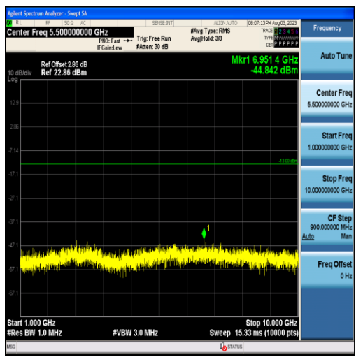
Band12-3MHz-QPSK-23095-15RB#0-Range2:1000~10000MHz
