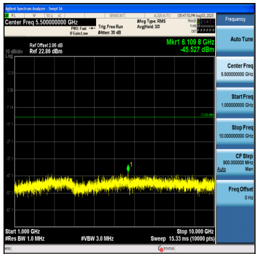
Band5-1.4MHz-QPSK-20525-6RB#0-Range2:1000~10000MHz
