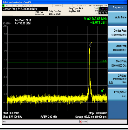
Band5-10MHz-16QAM-20450-50RB#0-Range1:30~1000MHz
