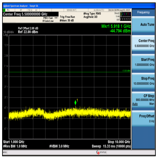
Band5-5MHz-QPSK-20525-25RB#0-Range2:1000~10000MHz
