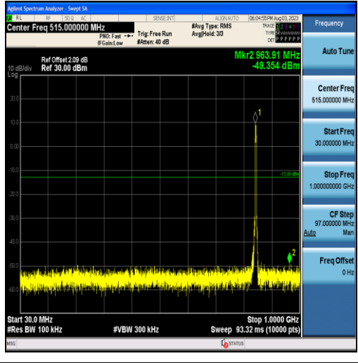
Band5-5MHz-16QAM-20625-25RB#0-Range1:30~1000MHz
