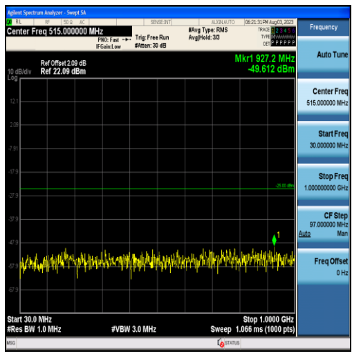
Band7-5MHz-QPSK-21100-25RB#0-Range1:30~1000MHz
