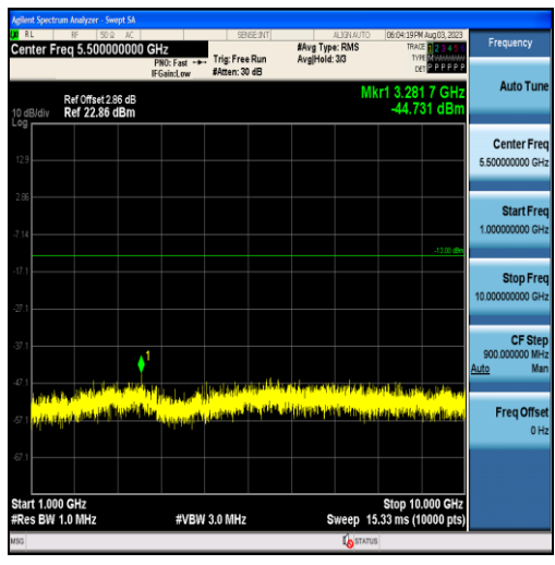
Band5-5MHz-16QAM-20425-25RB#0-Range2:1000~10000MHz
