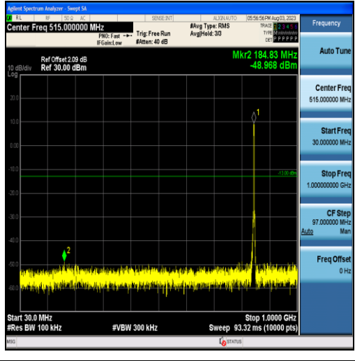
Band5-3MHz-16QAM-20635-15RB#0-Range1:30~1000MHz
