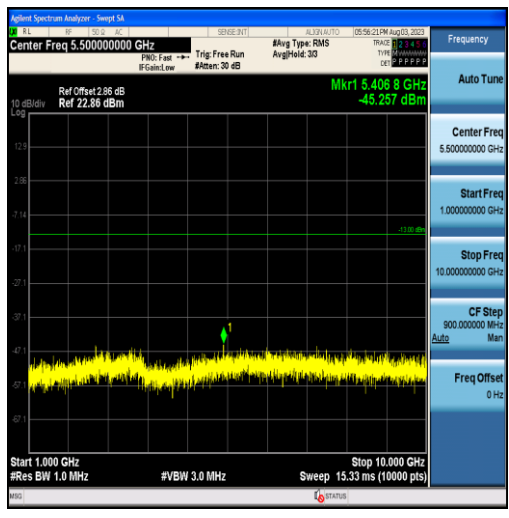
Band5-3MHz-16QAM-20415-15RB#0-Range2:1000~10000MHz
