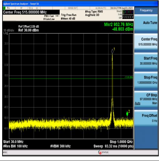
Band5-5MHz-QPSK-20525-25RB#0-Range1:30~1000MHz
