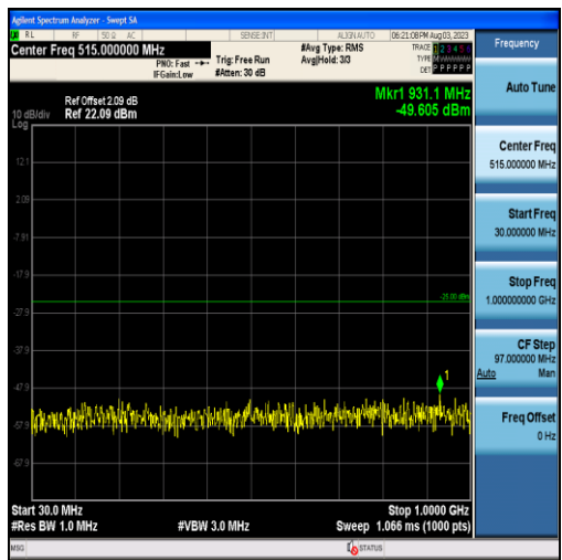
Band7-5MHz-16QAM-20775-25RB#0-Range1:30~1000MHz
