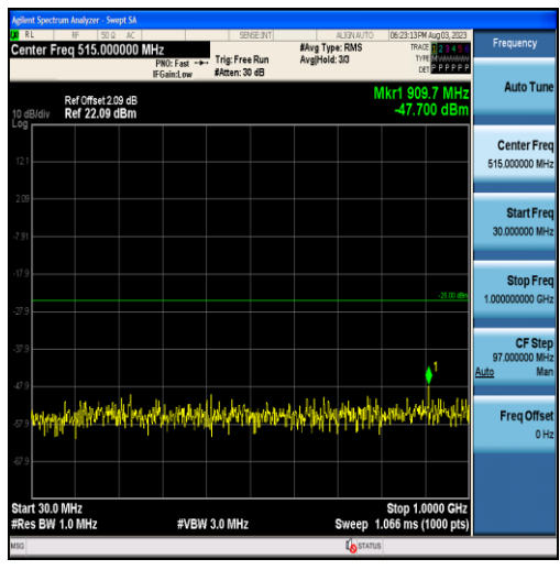
Band7-5MHz-16QAM-21425-25RB#0-Range1:30~1000MHz
