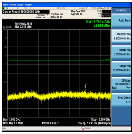
Band5-10MHz-16QAM-20450-50RB#0-Range2:1000~10000MHz
