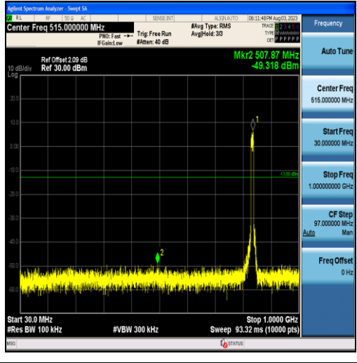
Band5-10MHz-QPSK-20525-50RB#0-Range1:30~1000MHz
