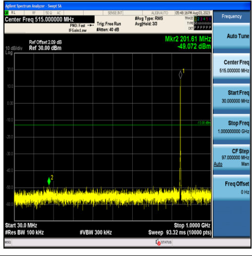
Band5-1.4MHz-16QAM-20643-6RB#0-Range1:30~1000MHz
