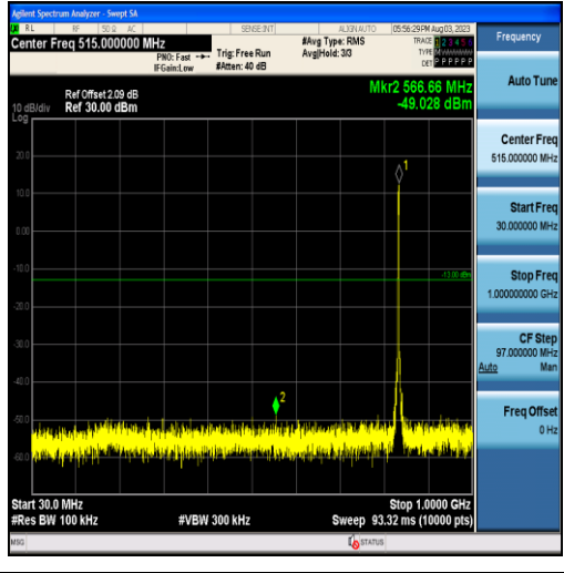
Band5-3MHz-QPSK-20525-15RB#0-Range1:30~1000MHz
