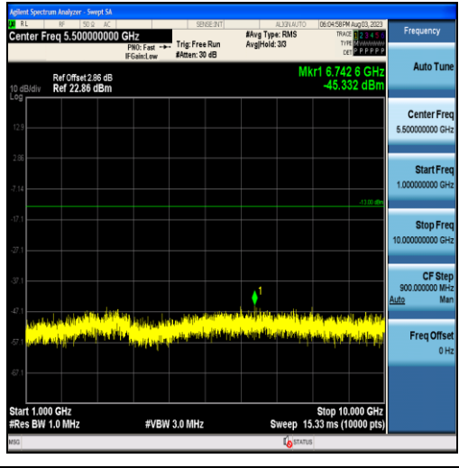
Band5-5MHz-16QAM-20625-25RB#0-Range2:1000~10000MHz
