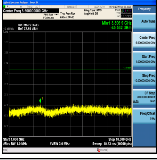
Band5-1.4MHz-16QAM-20643-6RB#0-Range2:1000~10000MHz
