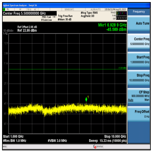
Band5-3MHz-QPSK-20635-15RB#0-Range2:1000~10000MHz
