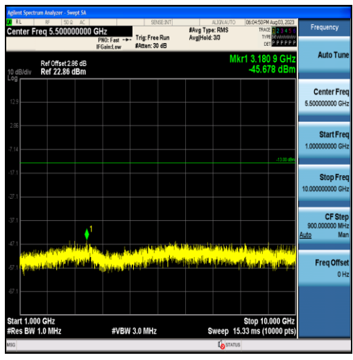
Band5-5MHz-QPSK-20625-25RB#0-Range2:1000~10000MHz
