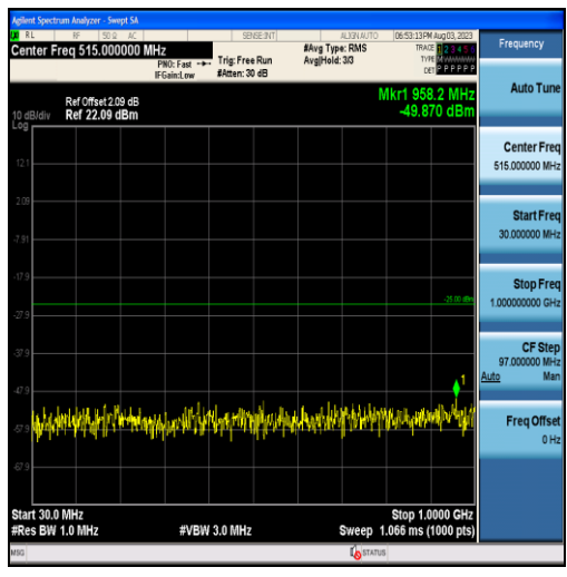
Band7-10MHz-16QAM-20800-50RB#0-Range1:30~1000MHz
