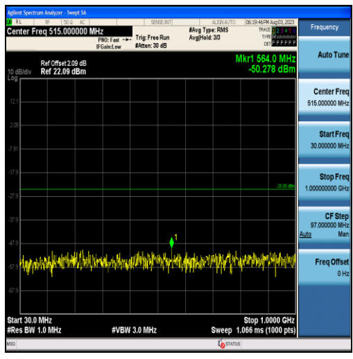
Band7-5MHz-QPSK-20775-25RB#0-Range1:30~1000MHz
