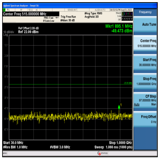
Band7-10MHz-16QAM-21100-50RB#0-Range1:30~1000MHz
