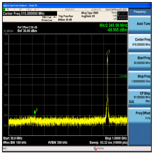
Band5-5MHz-16QAM-20525-25RB#0-Range1:30~1000MHz
