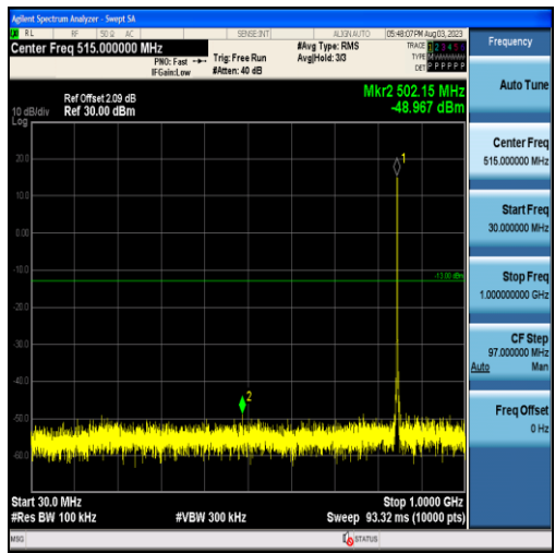
Band5-1.4MHz-QPSK-20643-6RB#0-Range1:30~1000MHz
