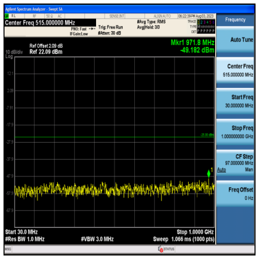
Band7-5MHz-QPSK-21425-25RB#0-Range1:30~1000MHz
