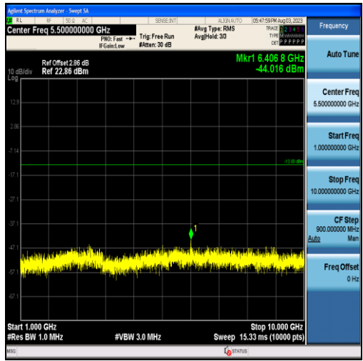
Band5-1.4MHz-16QAM-20525-6RB#0-Range2:1000~10000MHz
