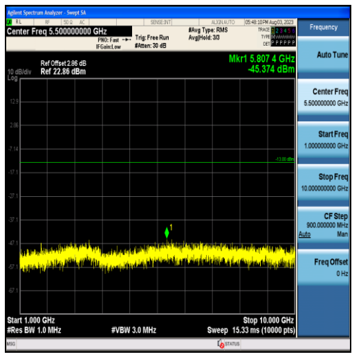
Band5-1.4MHz-QPSK-20643-6RB#0-Range2:1000~10000MHz
