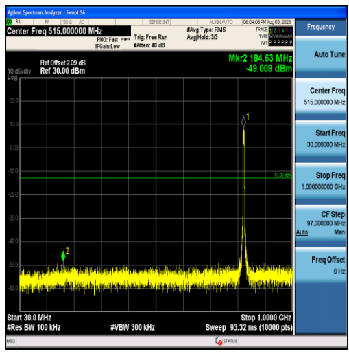
Band5-5MHz-QPSK-20425-25RB#0-Range1:30~1000MHz
