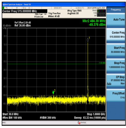
Band5-1.4MHz-QPSK-20407-6RB#0-Range1:30~1000MHz
