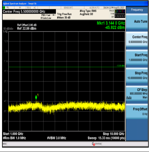
Band5-5MHz-QPSK-20425-25RB#0-Range2:1000~10000MHz
