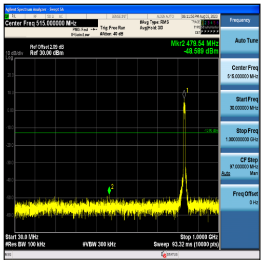
Band5-10MHz-16QAM-20525-50RB#0-Range1:30~1000MHz
