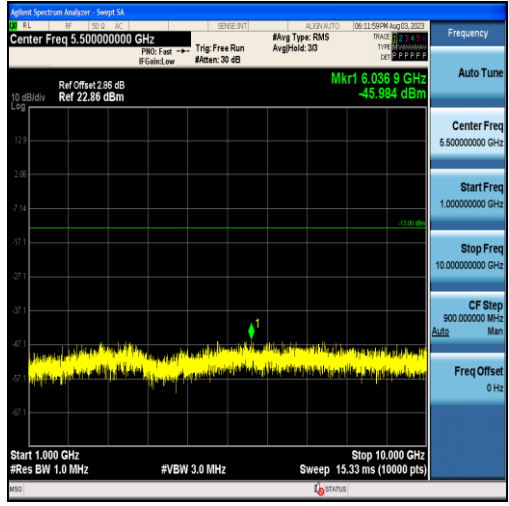
Band5-10MHz-16QAM-20525-50RB#0-Range2:1000~10000MHz
