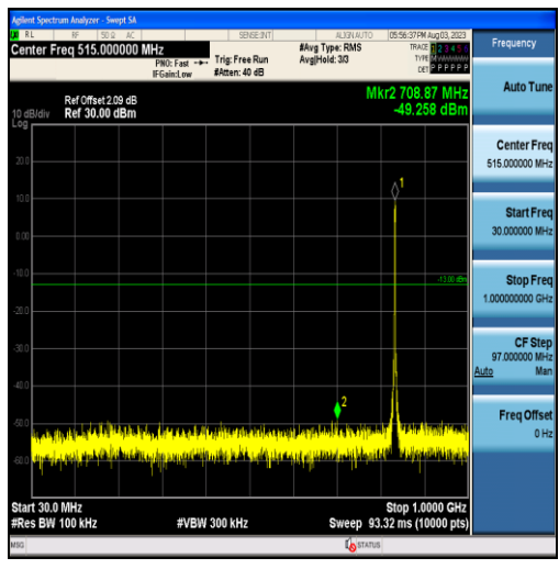
Band5-3MHz-16QAM-20525-15RB#0-Range1:30~1000MHz
