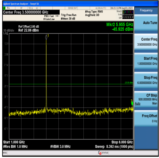
Band7-5MHz-16QAM-20775-25RB#0-Range2:1000~6000MHz
