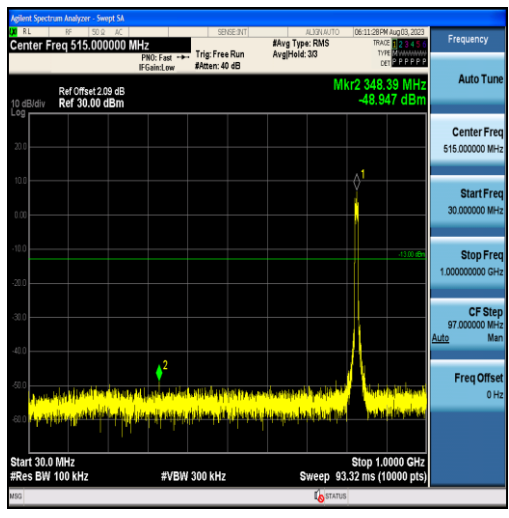
Band5-10MHz-QPSK-20450-50RB#0-Range1:30~1000MHz
