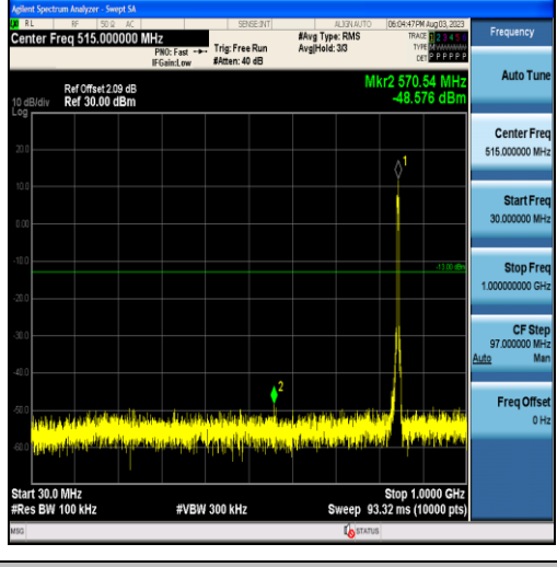
Band5-5MHz-QPSK-20625-25RB#0-Range1:30~1000MHz
