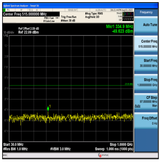
Band7-5MHz-16QAM-21100-25RB#0-Range1:30~1000MHz
