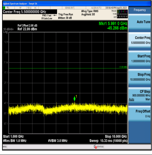
Band5-3MHz-16QAM-20525-15RB#0-Range2:1000~10000MHz
