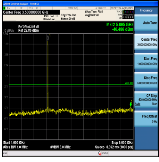
Band7-5MHz-16QAM-21425-25RB#0-Range2:1000~6000MHz
