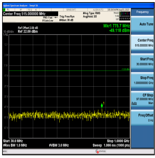
Band4-20MHz-16QAM-20175-100RB#0-Range1:30~1000MHz
