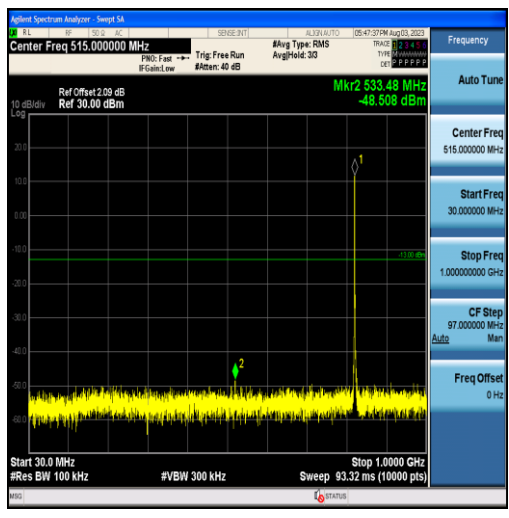
Band5-1.4MHz-16QAM-20407-6RB#0-Range1:30~1000MHz
