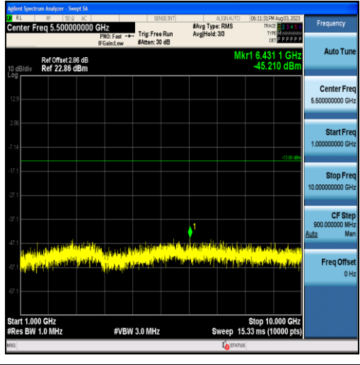
Band5-10MHz-QPSK-20450-50RB#0-Range2:1000~10000MHz
