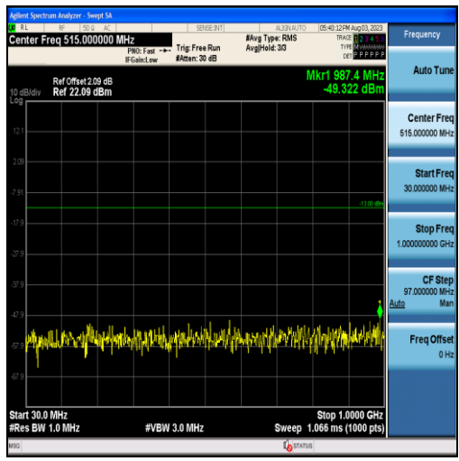
Band4-20MHz-16QAM-20300-100RB#0-Range1:30~1000MHz
