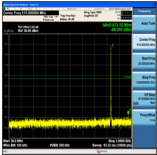
Band5-1.4MHz-QPSK-20525-6RB#0-Range1:30~1000MHz
