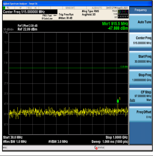
Band2-20MHz-QPSK-18900-100RB#0-Range1:30~1000MHz
