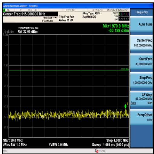
Band4-20MHz-16QAM-20050-100RB#0-Range1:30~1000MHz
