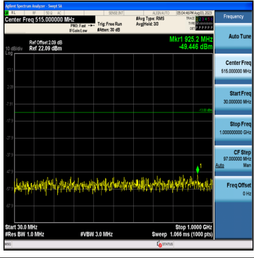
Band4-1.4MHz-QPSK-20175-6RB#0-Range1:30~1000MHz
