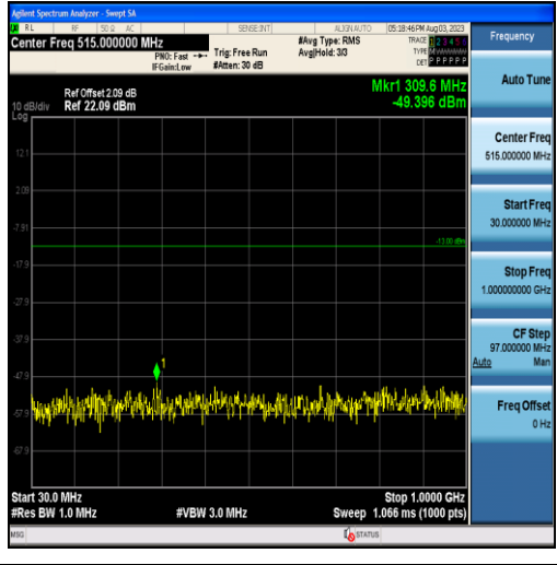
Band4-5MHz-QPSK-20175-25RB#0-Range1:30~1000MHz
