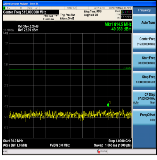
Band2-15MHz-16QAM-19125-75RB#0-Range1:30~1000MHz
