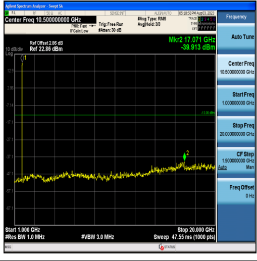
Band4-5MHz-16QAM-20175-25RB#0-Range2:1000~20000MHz
