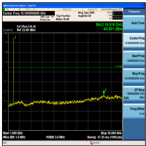
Band2-20MHz-16QAM-19100-100RB#0-Range2:1000~20000MHz
