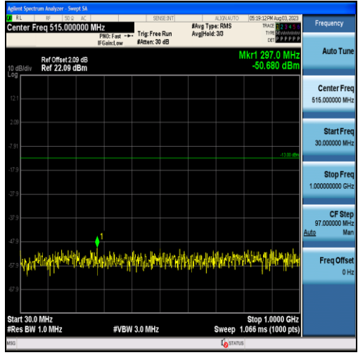
Band4-5MHz-16QAM-20375-25RB#0-Range1:30~1000MHz
