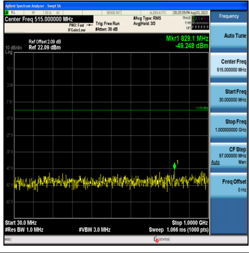
Band4-10MHz-16QAM-20350-50RB#0-Range1:30~1000MHz
