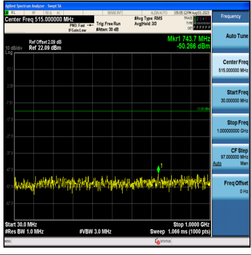
Band4-1.4MHz-16QAM-20393-6RB#0-Range1:30~1000MHz
