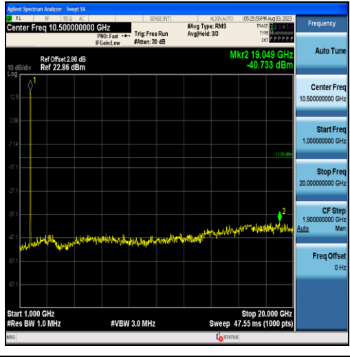
Band4-10MHz-16QAM-20350-50RB#0-Range2:1000~20000MHz
