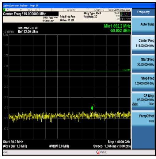
Band4-5MHz-QPSK-19975-25RB#0-Range1:30~1000MHz
