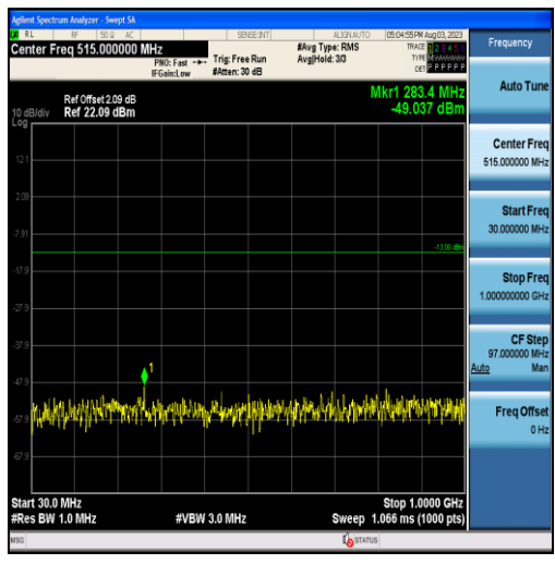
Band4-1.4MHz-16QAM-20175-6RB#0-Range1:30~1000MHz
