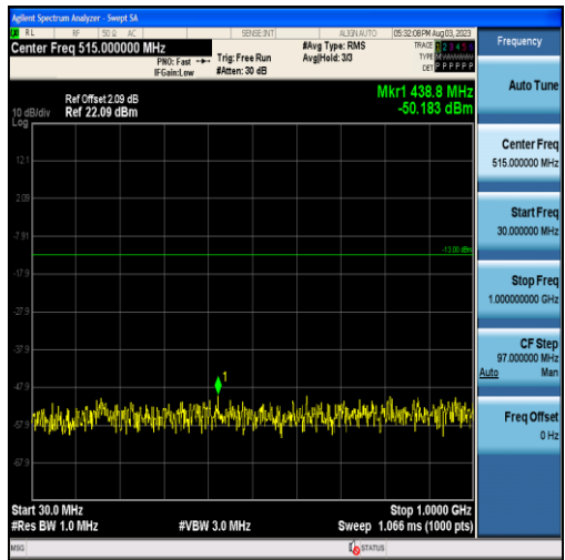
Band4-15MHz-QPSK-20025-75RB#0-Range1:30~1000MHz
