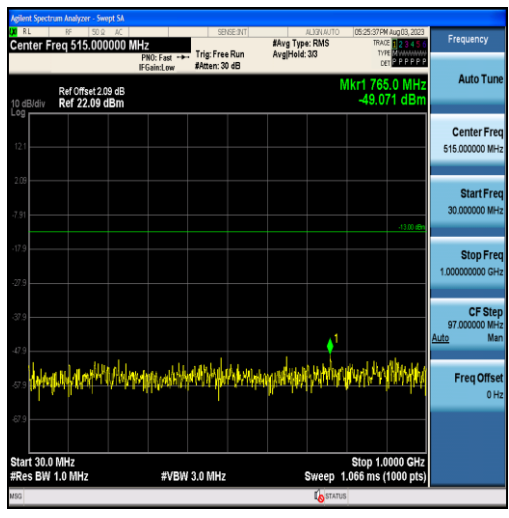
Band4-10MHz-16QAM-20175-50RB#0-Range1:30~1000MHz
