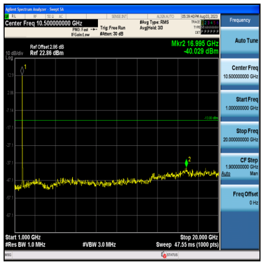
Band4-20MHz-16QAM-20050-100RB#0-Range2:1000~20000MHz
