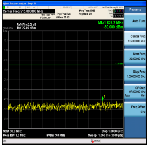
Band2-15MHz-QPSK-18900-75RB#0-Range1:30~1000MHz
