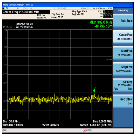
Band2-15MHz-16QAM-18900-75RB#0-Range1:30~1000MHz
