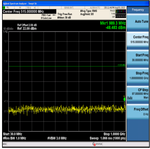
Band4-3MHz-16QAM-20385-15RB#0-Range1:30~1000MHz
