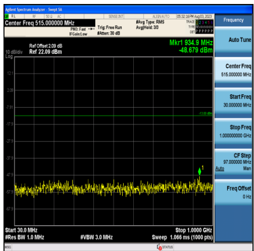
Band4-15MHz-16QAM-20025-75RB#0-Range1:30~1000MHz
