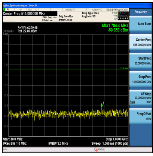
Band4-5MHz-16QAM-20175-25RB#0-Range1:30~1000MHz
