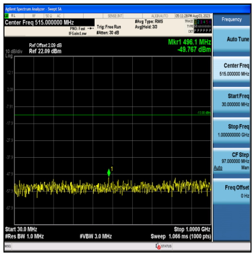
Band4-3MHz-16QAM-20175-15RB#0-Range1:30~1000MHz
