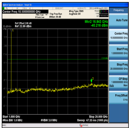
Band4-3MHz-16QAM-20385-15RB#0-Range2:1000~20000MHz
