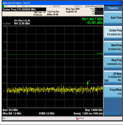
Band4-20MHz-QPSK-20175-100RB#0-Range1:30~1000MHz
