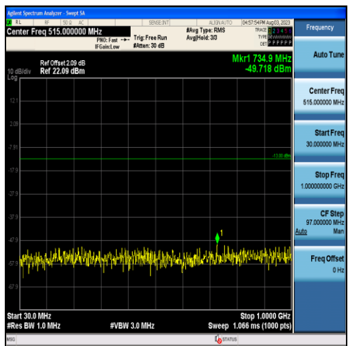
Band2-20MHz-16QAM-19100-100RB#0-Range1:30~1000MHz
