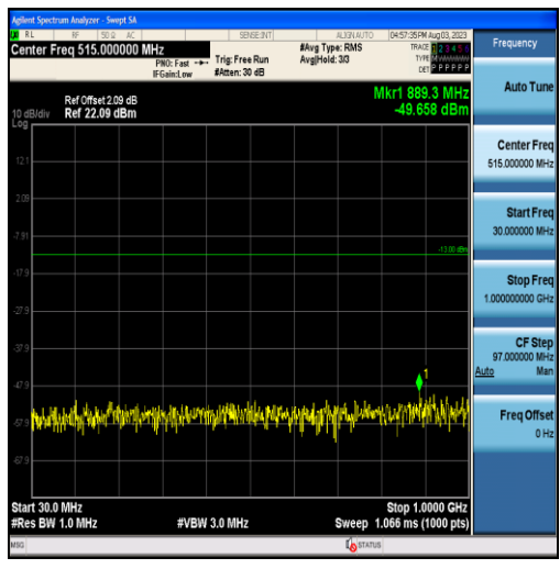
Band2-20MHz-16QAM-18900-100RB#0-Range1:30~1000MHz
