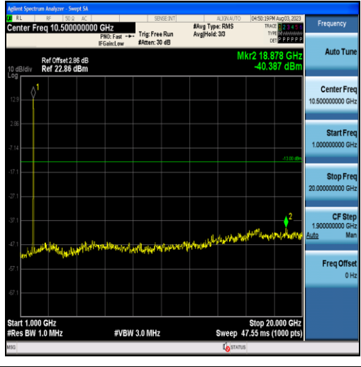
Band2-15MHz-16QAM-18900-75RB#0-Range2:1000~20000MHz
