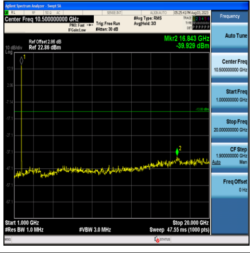
Band4-10MHz-16QAM-20175-50RB#0-Range2:1000~20000MHz
