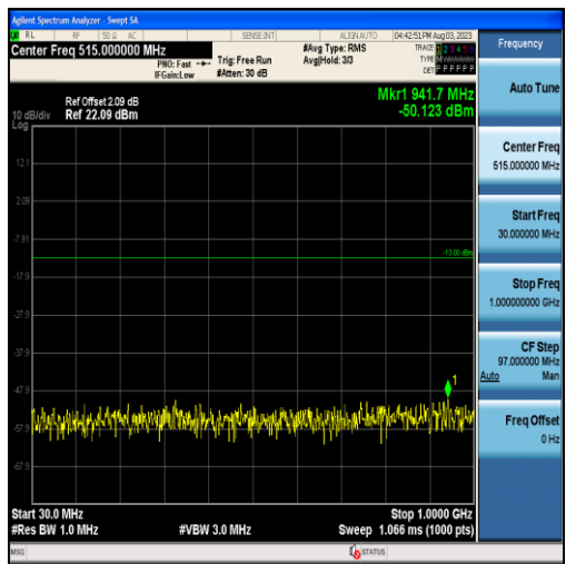
Band2-10MHz-QPSK-18650-50RB#0-Range1:30~1000MHz
