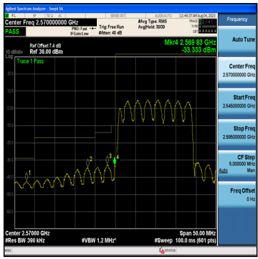
Band38-20MHz-16QAM-37850-100RB#0
