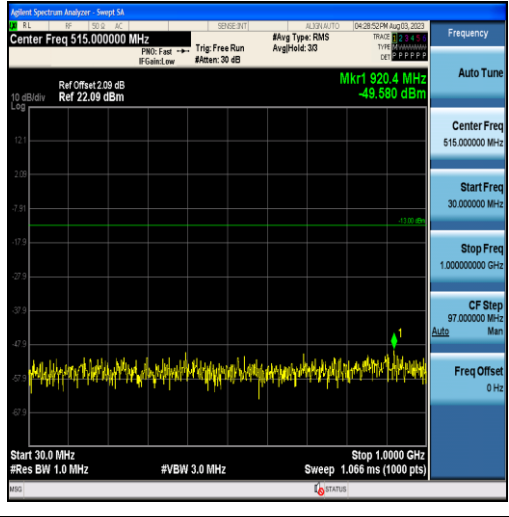
Band2-3MHz-QPSK-18900-15RB#0-Range1:30~1000MHz
