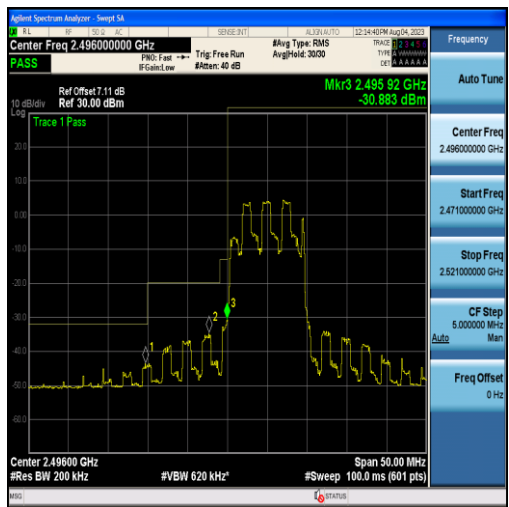
Band41-10MHz-16QAM-39700-50RB#0
