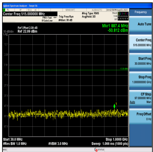
Band2-10MHz-16QAM-18650-50RB#0-Range1:30~1000MHz
