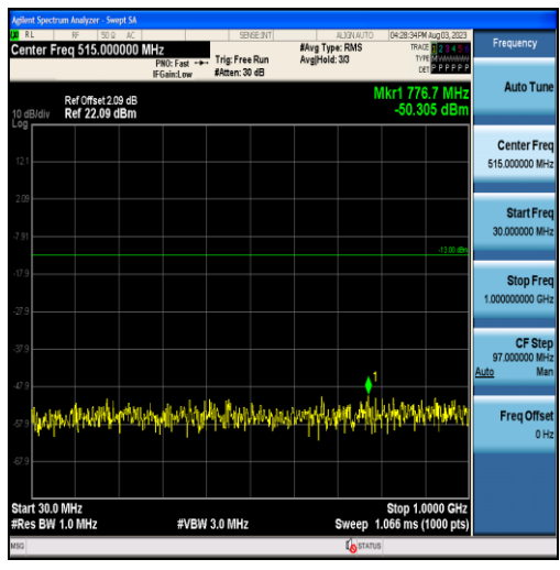
Band2-3MHz-QPSK-18615-15RB#0-Range1:30~1000MHz
