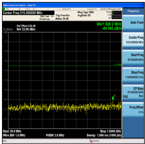
Band2-10MHz-16QAM-18900-50RB#0-Range1:30~1000MHz
