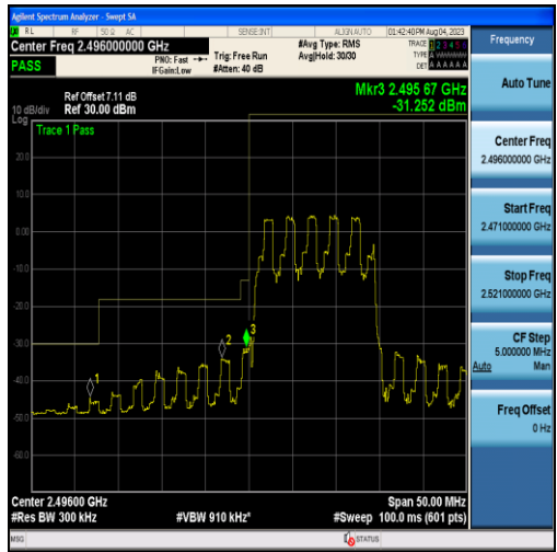
Band41-15MHz-16QAM-39725-75RB#0
