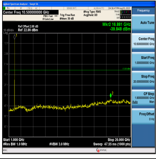
Band2-5MHz-16QAM-19175-25RB#0-Range2:1000~20000MHz
