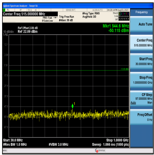
Band2-1.4MHz-QPSK-19193-6RB#0-Range1:30~1000MHz
