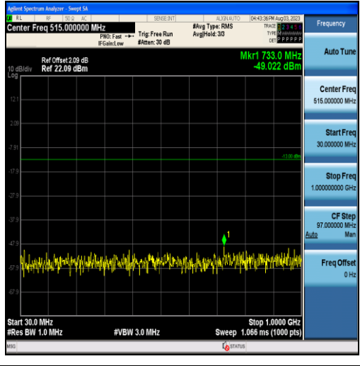
Band2-10MHz-16QAM-19150-50RB#0-Range1:30~1000MHz
