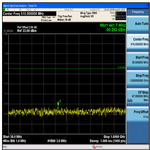
Band2-10MHz-QPSK-19150-50RB#0-Range1:30~1000MHz
