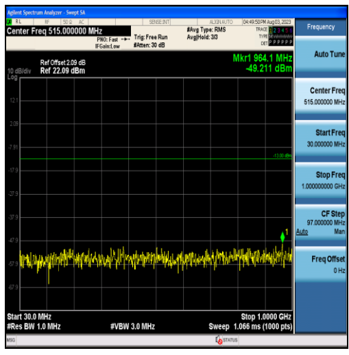
Band2-15MHz-QPSK-18675-75RB#0-Range1:30~1000MHz
