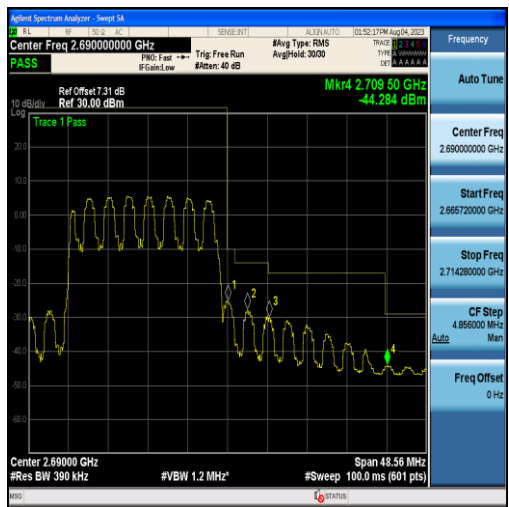
Band41-20MHz-QPSK-41490-100RB#0
