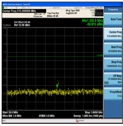
Band2-5MHz-16QAM-18900-25RB#0-Range1:30~1000MHz
