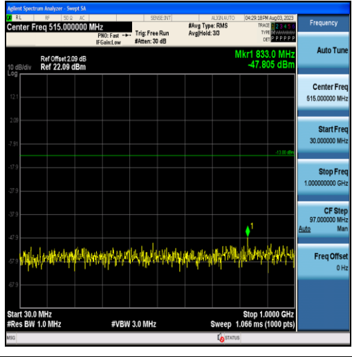
Band2-3MHz-16QAM-19185-15RB#0-Range1:30~1000MHz
