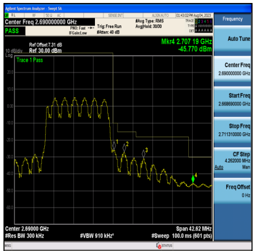
Band41-15MHz-QPSK-41515-75RB#0
