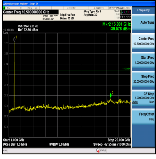
Band2-15MHz-QPSK-18675-75RB#0-Range2:1000~20000MHz
