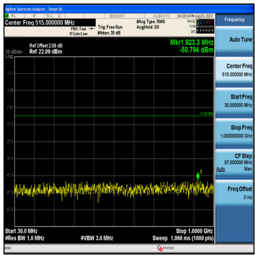
Band2-1.4MHz-16QAM-18900-6RB#0-Range1:30~1000MHz
