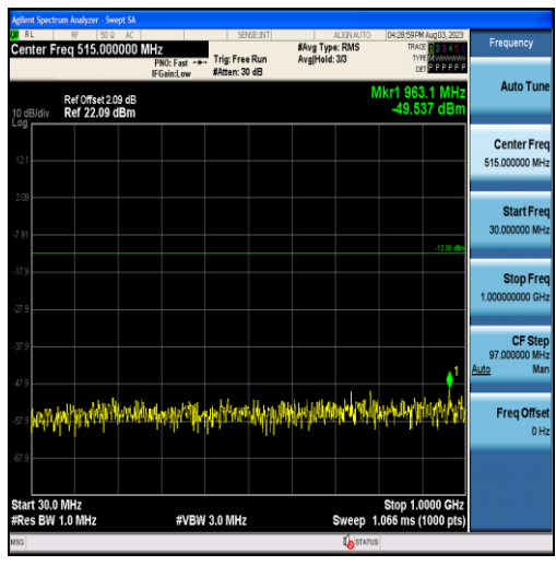
Band2-3MHz-16QAM-18900-15RB#0-Range1:30~1000MHz
