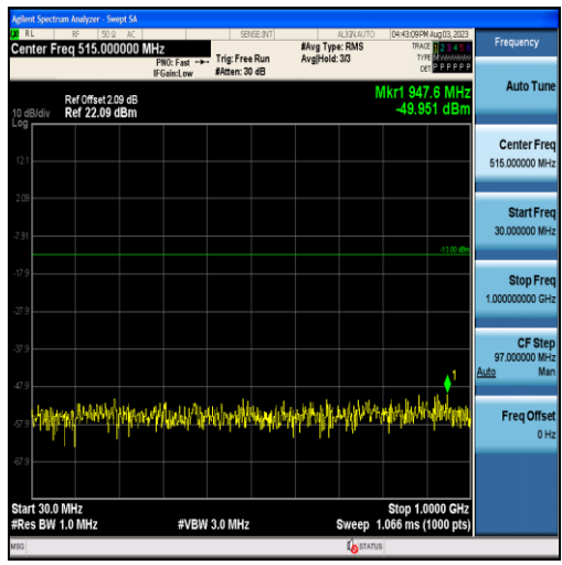
Band2-10MHz-QPSK-18900-50RB#0-Range1:30~1000MHz
