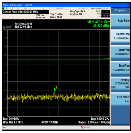
Band2-15MHz-16QAM-18675-75RB#0-Range1:30~1000MHz
