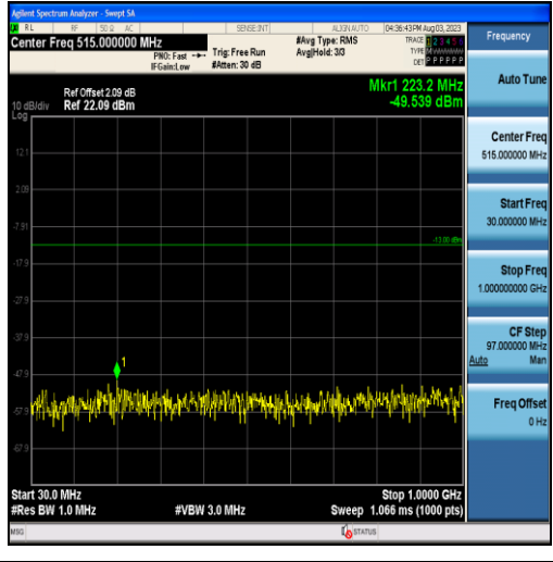
Band2-5MHz-16QAM-19175-25RB#0-Range1:30~1000MHz
