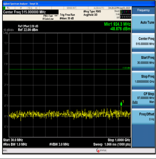
Band2-1.4MHz-16QAM-19193-6RB#0-Range1:30~1000MHz
