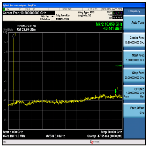
Band2-5MHz-16QAM-18625-25RB#0-Range2:1000~20000MHz
