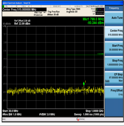
Band2-1.4MHz-QPSK-18900-6RB#0-Range1:30~1000MHz
