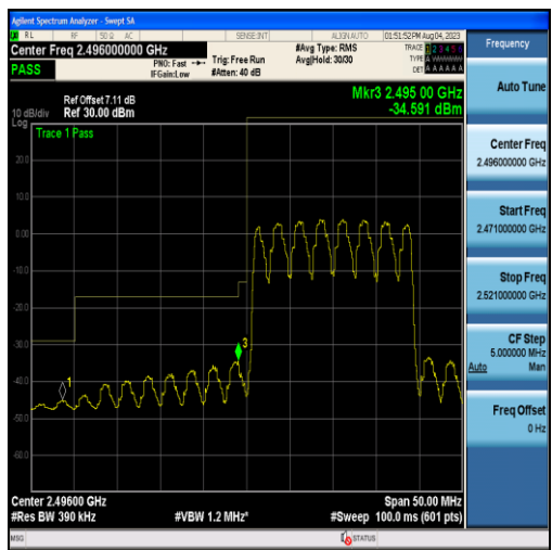
Band41-20MHz-16QAM-39750-100RB#0
