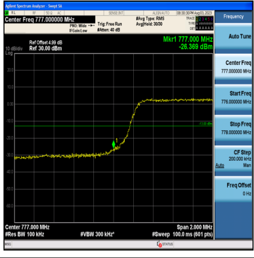
Band13-5MHz-16QAM-23205-25RB#0
