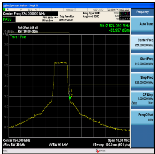
Band26-1.4MHz-16QAM-26783-6RB#0
