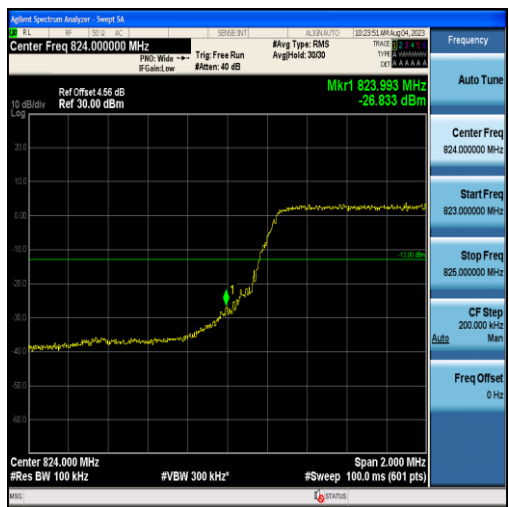
Band26-5MHz-QPSK-26815-25RB#0
