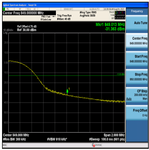
Band26-15MHz-QPSK-26965-75RB#0
