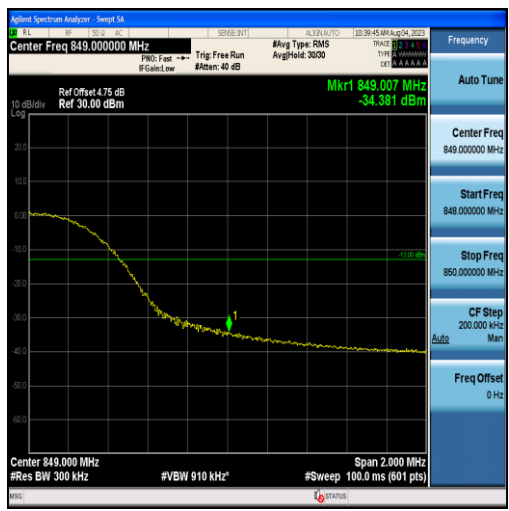
Band26-15MHz-16QAM-26965-75RB#0
