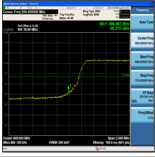
Band12-5MHz-QPSK-23035-25RB#0
