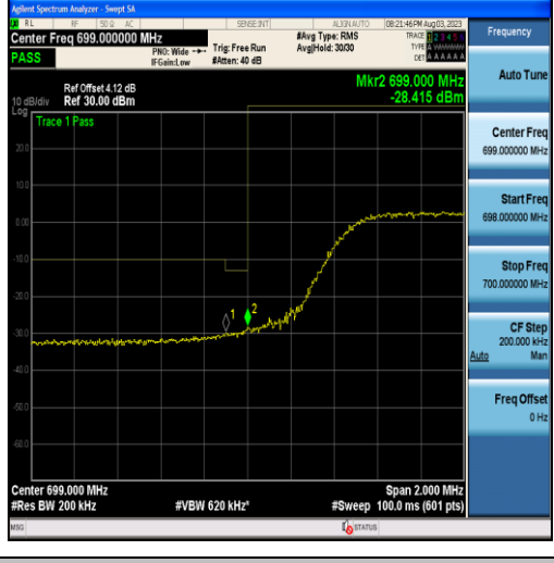
Band12-10MHz-QPSK-23060-50RB#0
