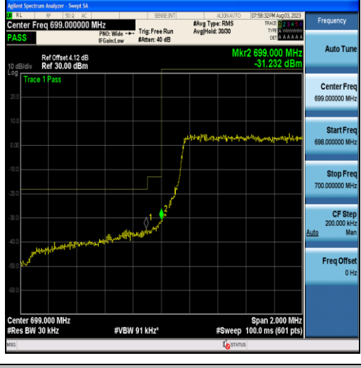
Band12-1.4MHz-QPSK-23017-6RB#0
