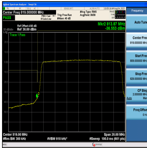
Band26-15MHz-16QAM-26765-75RB#0
