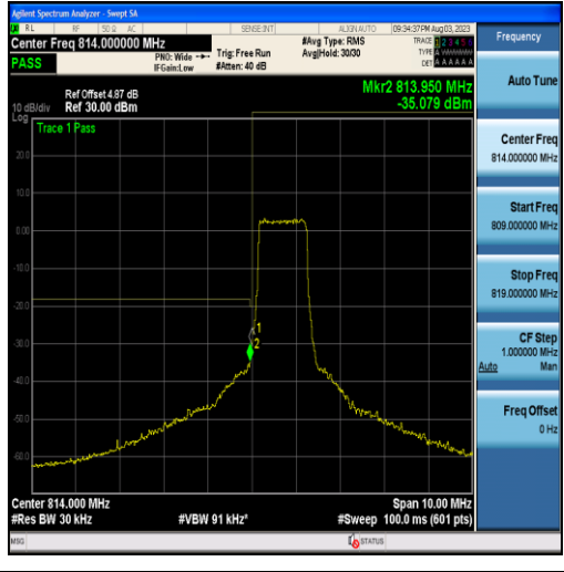
Band26-1.4MHz-16QAM-26697-6RB#0
