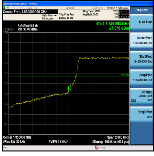
Band25-1.4MHz-16QAM-26047-6RB#0
