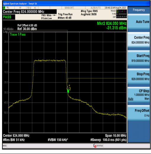
Band26-3MHz-QPSK-26775-15RB#0
