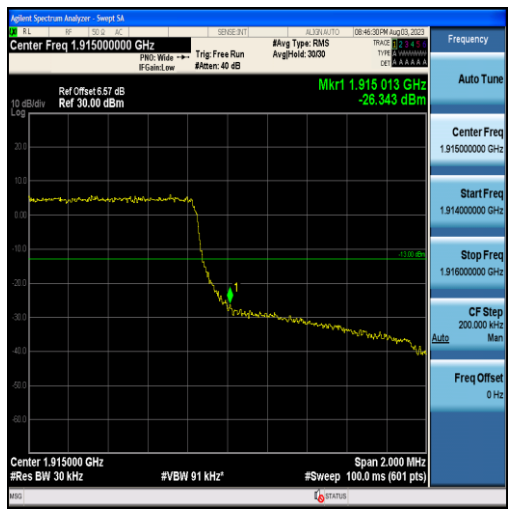
Band25-1.4MHz-16QAM-26683-6RB#0
