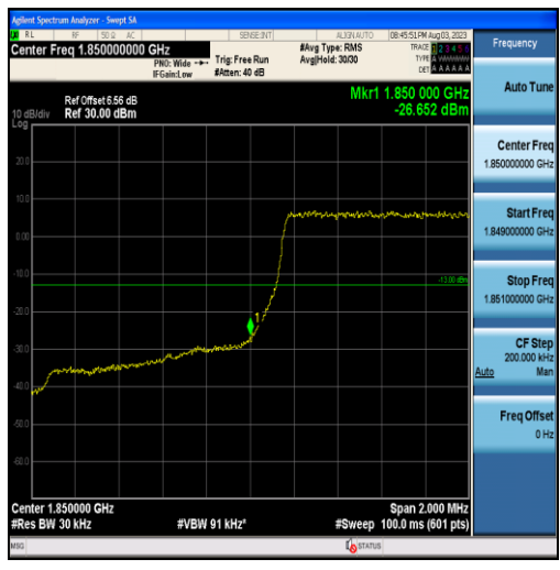
Band25-1.4MHz-QPSK-26047-6RB#0
