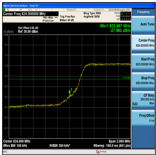
Band26-5MHz-16QAM-26815-25RB#0
