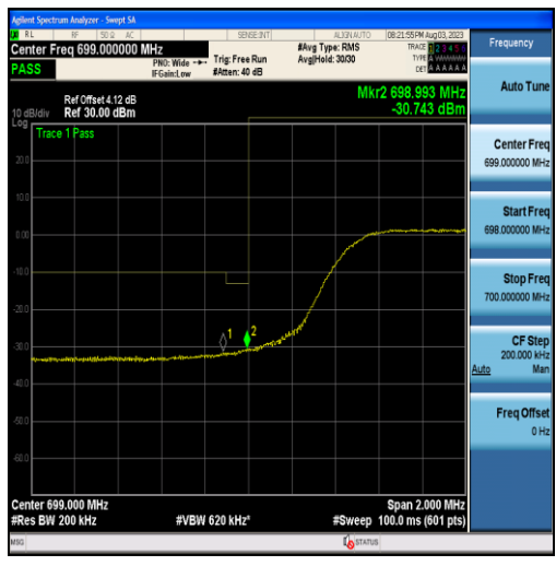
Band12-10MHz-16QAM-23060-50RB#0
