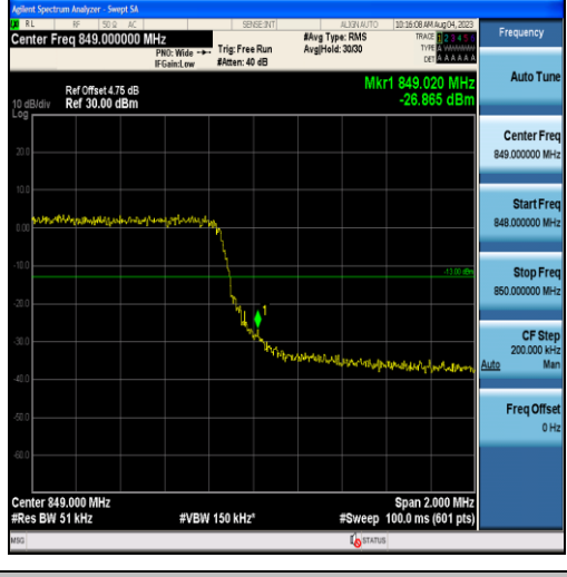
Band26-3MHz-QPSK-27025-15RB#0
