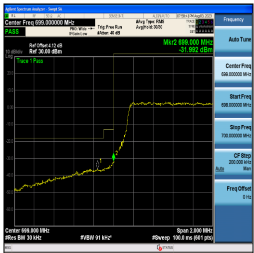
Band12-1.4MHz-16QAM-23017-6RB#0
