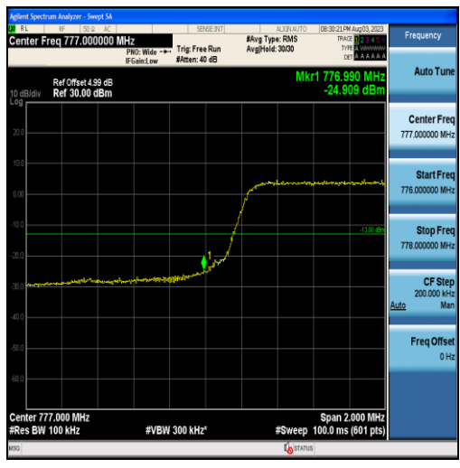
Band13-5MHz-QPSK-23205-25RB#0
