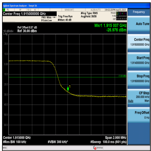
Band25-5MHz-16QAM-26665-25RB#0
