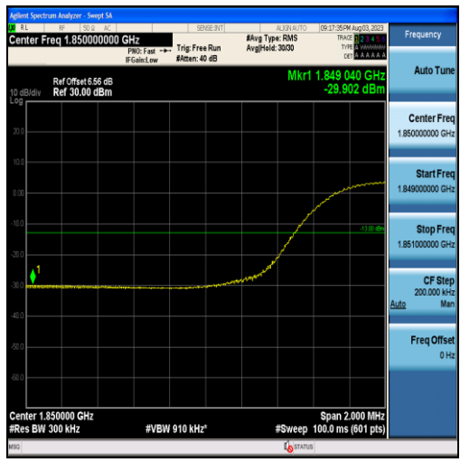
Band25-15MHz-QPSK-26115-75RB#0
