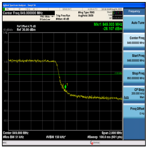
Band26-3MHz-16QAM-27025-15RB#0
