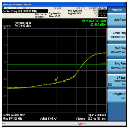
Band26-15MHz-16QAM-26865-75RB#0
