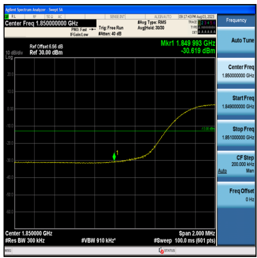
Band25-15MHz-16QAM-26115-75RB#0
