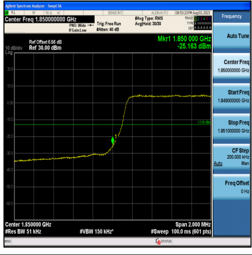
Band25-3MHz-QPSK-26055-15RB#0
