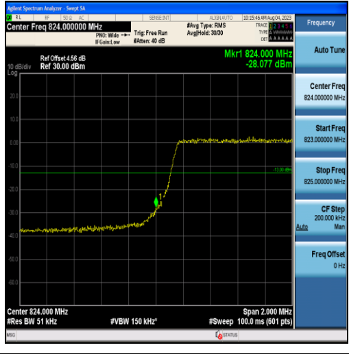
Band26-3MHz-16QAM-26805-15RB#0
