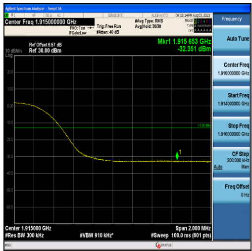
Band25-15MHz-16QAM-26615-75RB#0
