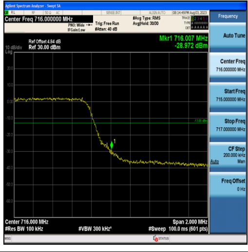
Band12-5MHz-16QAM-23155-25RB#0
