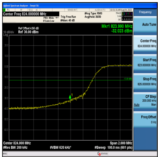
Band26-10MHz-16QAM-26840-50RB#0
