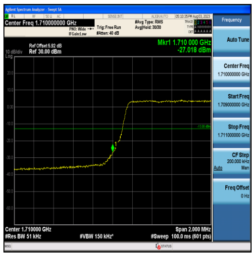
Band4-3MHz-16QAM-19965-15RB#0
