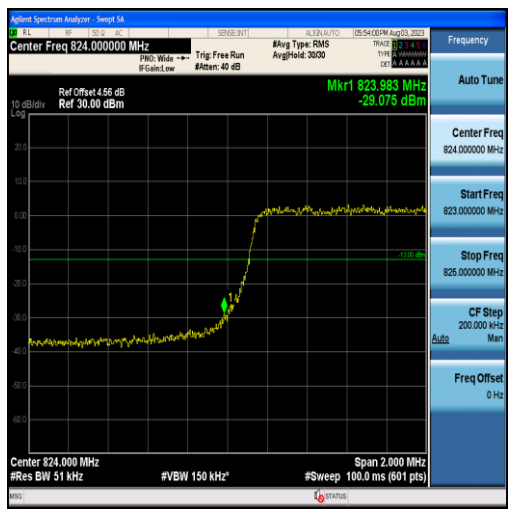
Band5-3MHz-16QAM-20415-15RB#0
