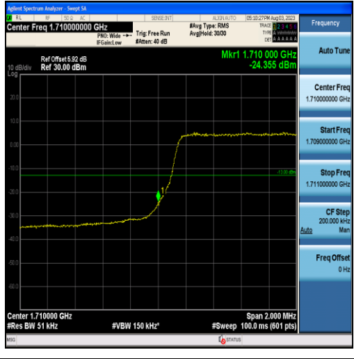
Band4-3MHz-QPSK-19965-15RB#0
