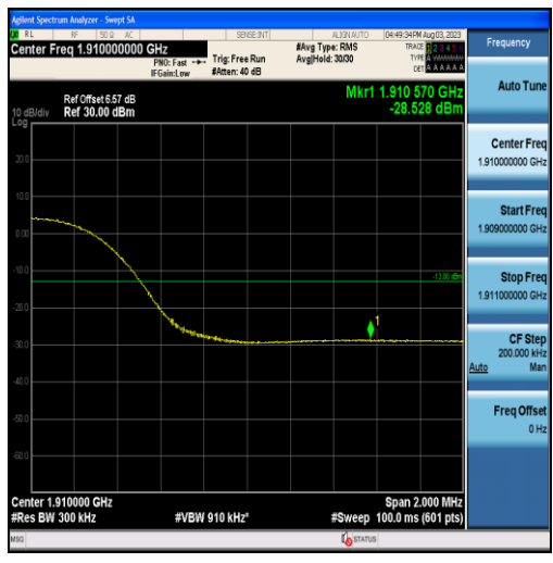
Band2-15MHz-QPSK-19125-75RB#0
