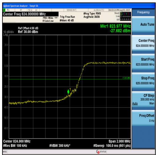
Band5-5MHz-QPSK-20425-25RB#0
