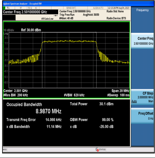
Band41-10MHz-QPSK-39700-50RB#0-8.9870
