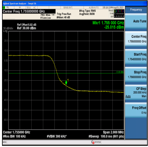
Band4-5MHz-QPSK-20375-25RB#0
