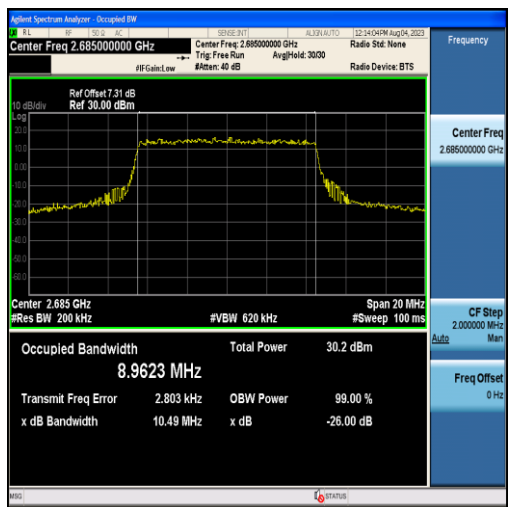
Band41-10MHz-QPSK-41540-50RB#0-8.9623
