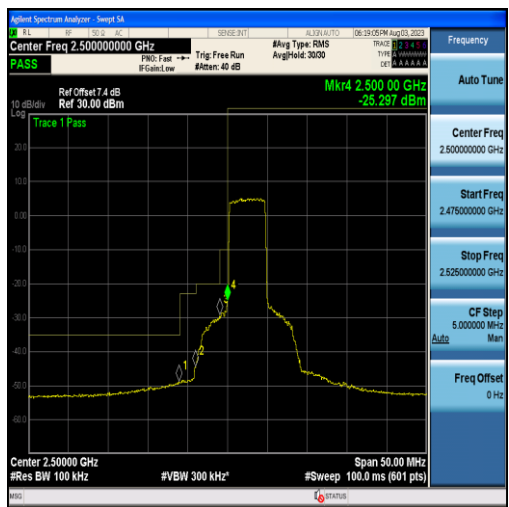
Band7-5MHz-16QAM-20775-25RB#0
