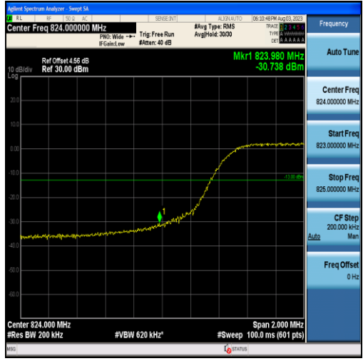
Band5-10MHz-16QAM-20450-50RB#0
