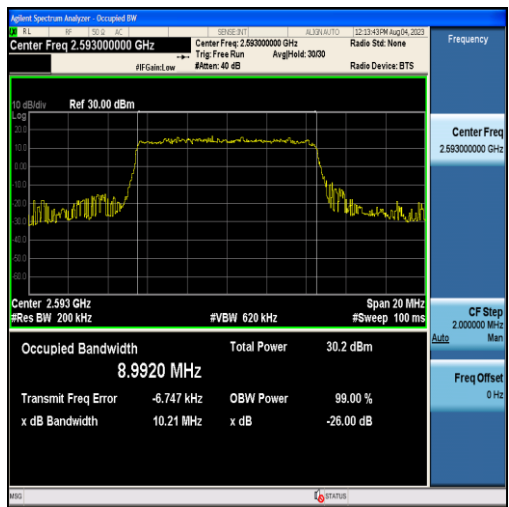
Band41-10MHz-QPSK-40620-50RB#0-8.9920
