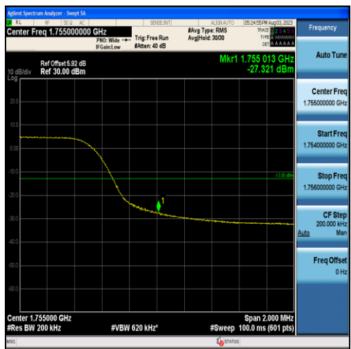
Band4-10MHz-QPSK-20350-50RB#0
