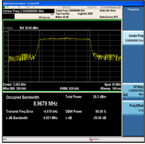
Band41-10MHz-16QAM-40620-50RB#0-8.9679
