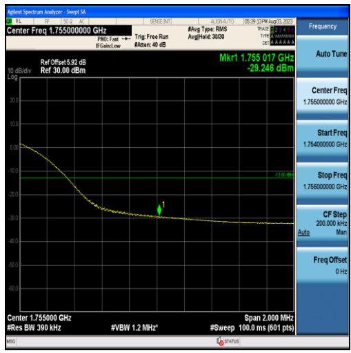
Band4-20MHz-QPSK-20300-100RB#0
