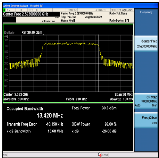
Band41-15MHz-QPSK-40620-75RB#0-13.420
