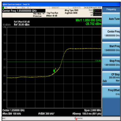
Band2-5MHz-16QAM-18625-25RB#0
