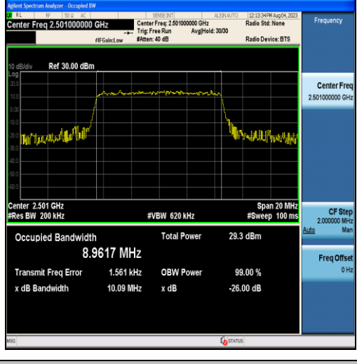
Band41-10MHz-16QAM-39700-50RB#0-8.9617
