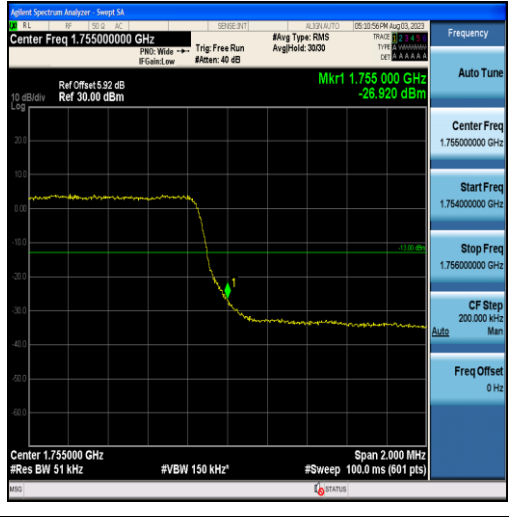
Band4-3MHz-16QAM-20385-15RB#0
