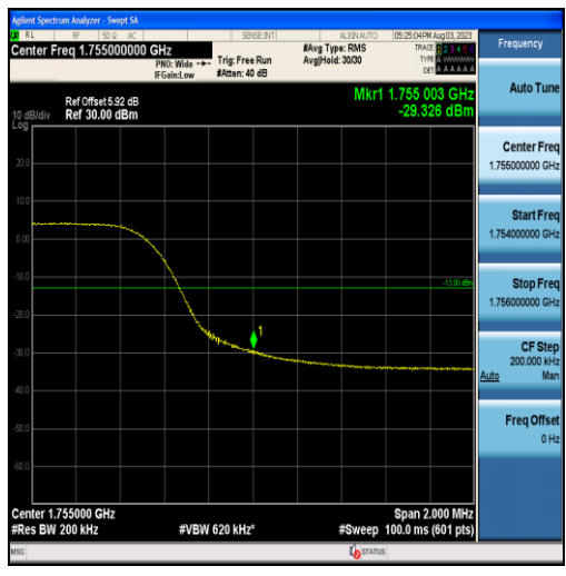
Band4-10MHz-16QAM-20350-50RB#0
