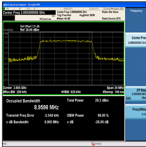
Band41-10MHz-16QAM-41540-50RB#0-8.9598
