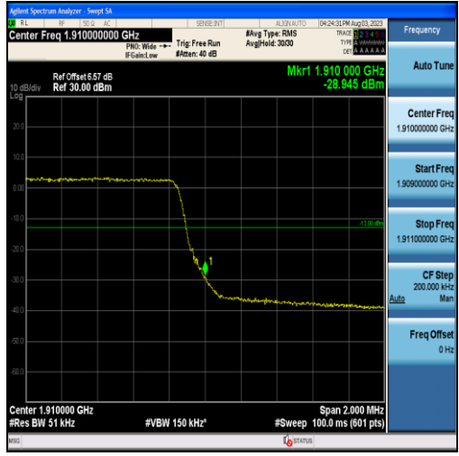
Band2-3MHz-16QAM-19185-15RB#0
