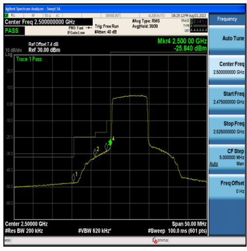
Band7-10MHz-16QAM-20800-50RB#0
