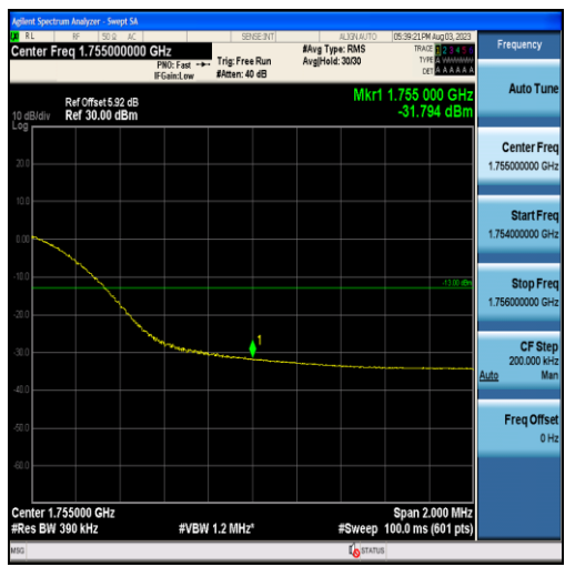
Band4-20MHz-16QAM-20300-100RB#0
