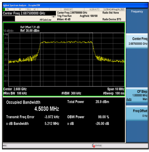
Band41-5MHz-16QAM-41565-25RB#0-4.5030
