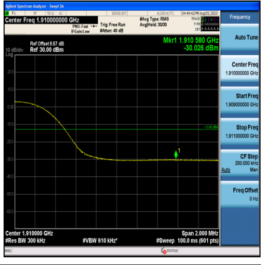
Band2-15MHz-16QAM-19125-75RB#0
