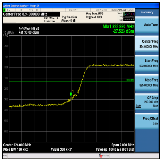
Band5-5MHz-16QAM-20425-25RB#0
