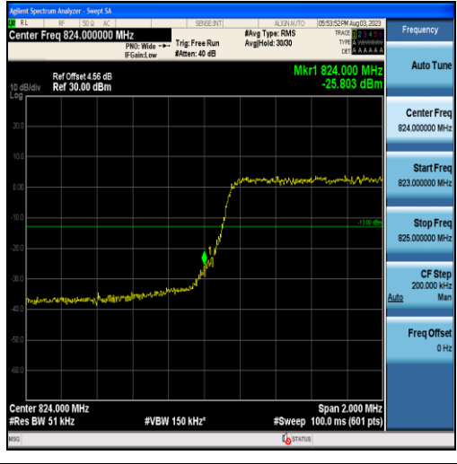
Band5-3MHz-QPSK-20415-15RB#0
