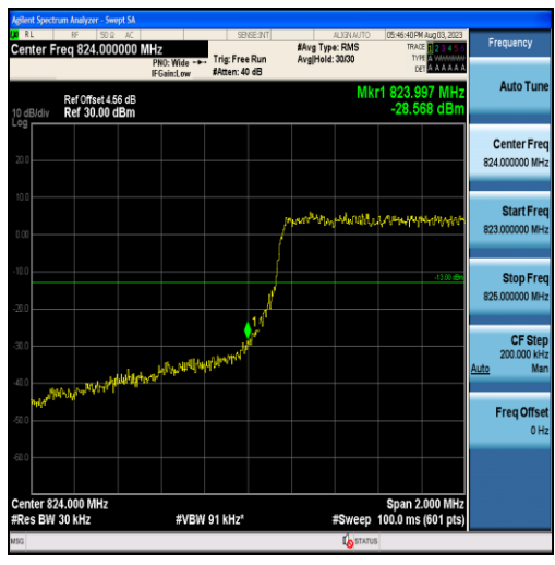
Band5-1.4MHz-QPSK-20407-6RB#0
