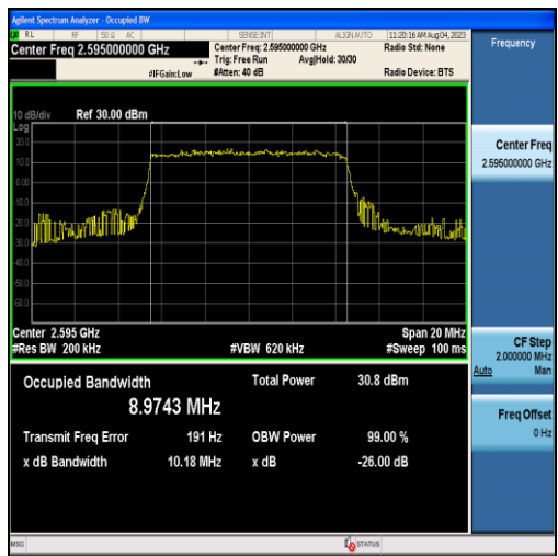
Band38-10MHz-QPSK-38000-50RB#0-8.9743
