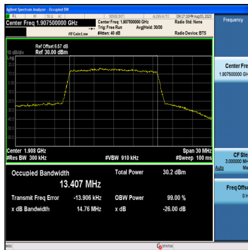
Band25-15MHz-QPSK-26615-75RB#0-13.407
