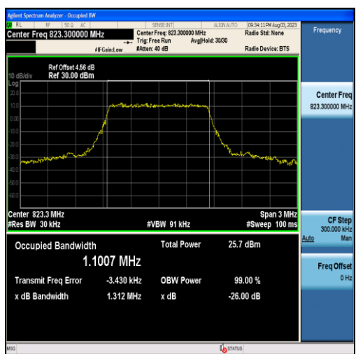
Band26-1.4MHz-16QAM-26783-6RB#0-1.1007
