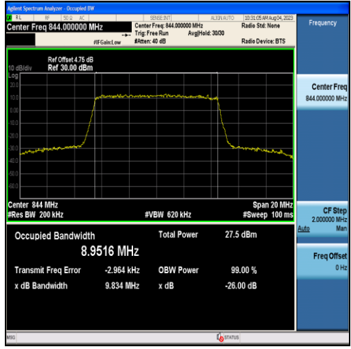
Band26-10MHz-16QAM-26990-50RB#0-8.9516
