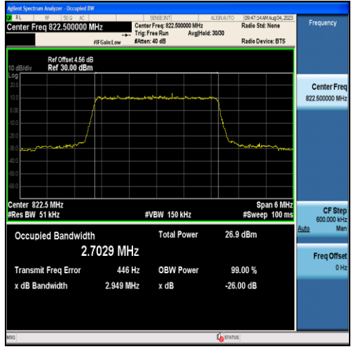
Band26-3MHz-QPSK-26775-15RB#0-2.7029
