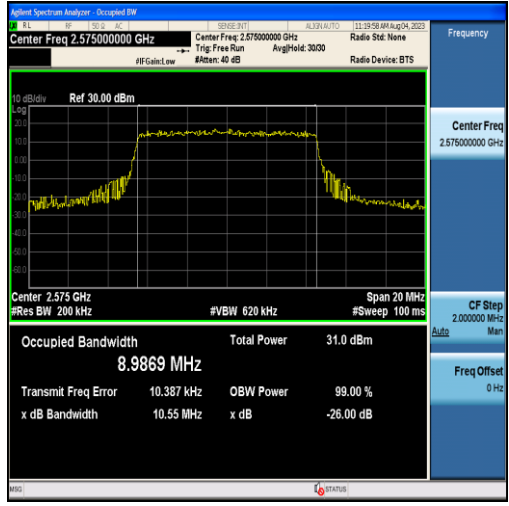
Band38-10MHz-QPSK-37800-50RB#0-8.9869
