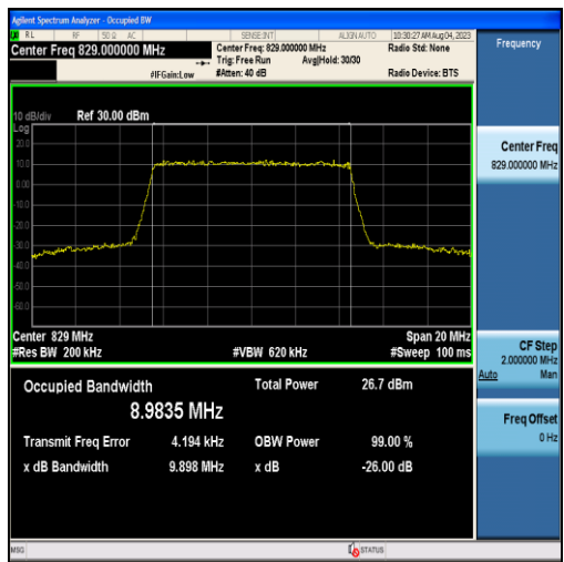
Band26-10MHz-16QAM-26840-50RB#0-8.9835
