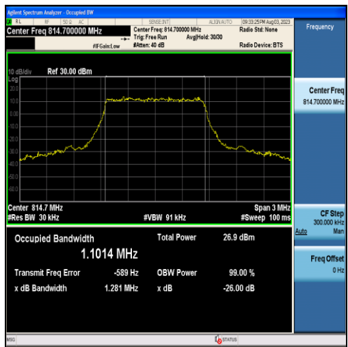
Band26-1.4MHz-QPSK-26697-6RB#0-1.1014
