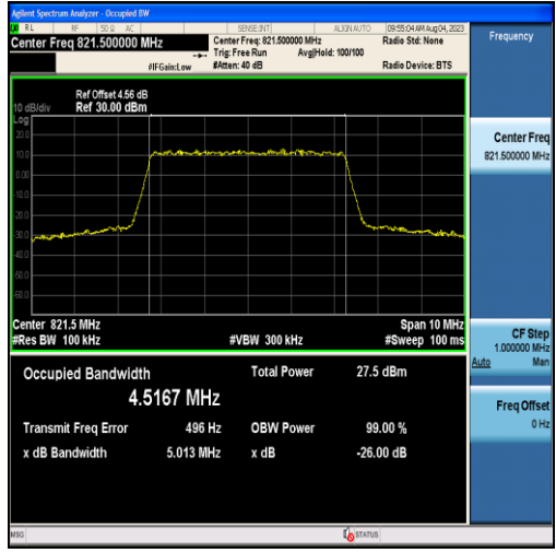
Band26-5MHz-QPSK-26765-25RB#0-4.5167
