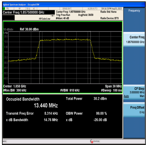
Band25-15MHz-QPSK-26115-75RB#0-13.440
