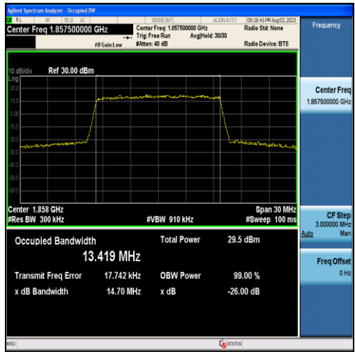
Band25-15MHz-16QAM-26115-75RB#0-13.419
