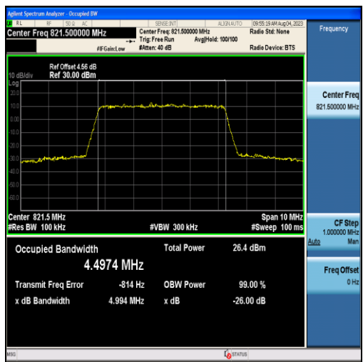
Band26-5MHz-16QAM-26765-25RB#0-4.4974
