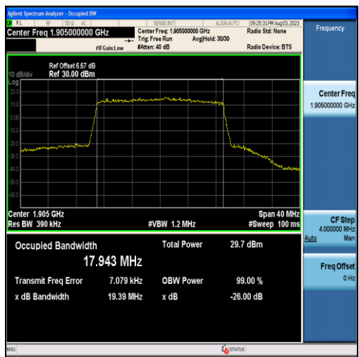
Band25-20MHz-16QAM-26590-100RB#0-17.943
