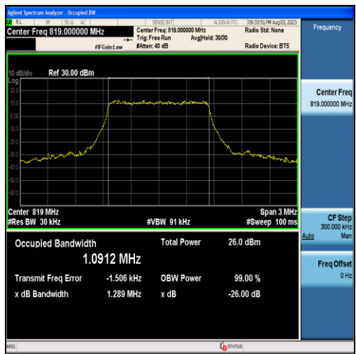
Band26-1.4MHz-16QAM-26740-6RB#0-1.0912
