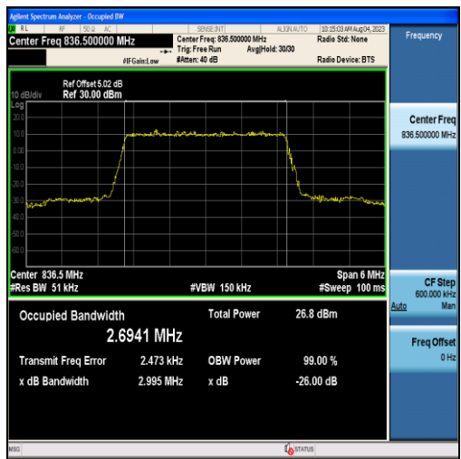
Band26-3MHz-16QAM-26915-15RB#0-2.6941
