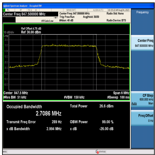
Band26-3MHz-16QAM-27025-15RB#0-2.7086
