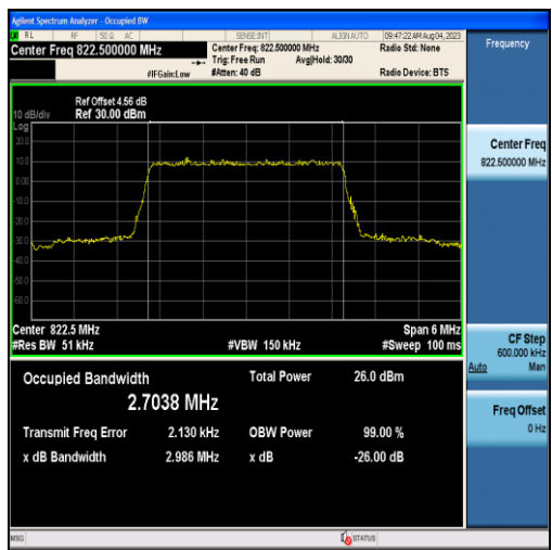
Band26-3MHz-16QAM-26775-15RB#0-2.7038
