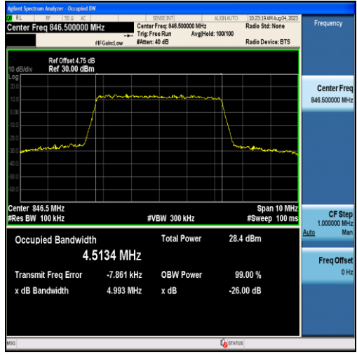
Band26-5MHz-QPSK-27015-25RB#0-4.5134
