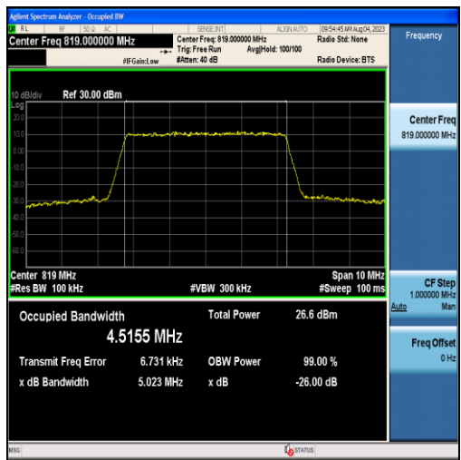
Band26-5MHz-16QAM-26740-25RB#0-4.5155
