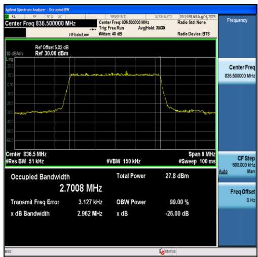
Band26-3MHz-QPSK-26915-15RB#0-2.7008
