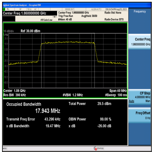
Band25-20MHz-16QAM-26140-100RB#0-17.943
