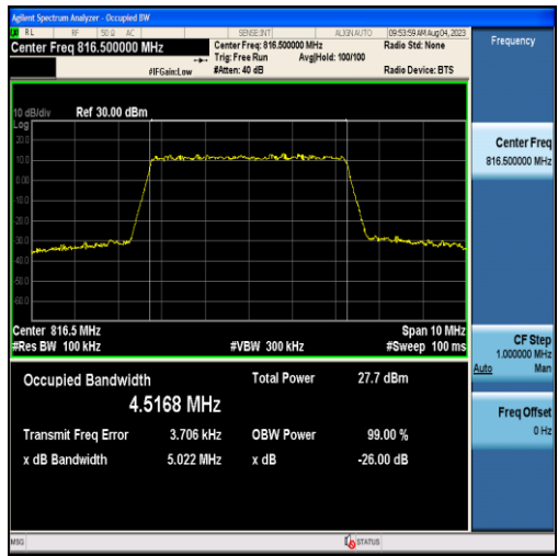
Band26-5MHz-QPSK-26715-25RB#0-4.5168
