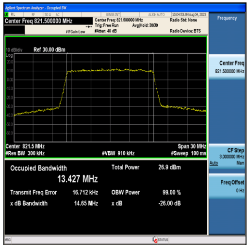
Band26-15MHz-16QAM-26765-75RB#0-13.427
