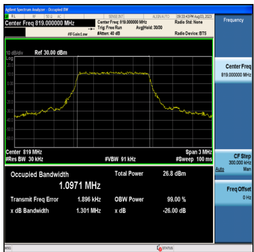
Band26-1.4MHz-QPSK-26740-6RB#0-1.0971
