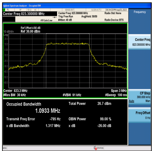
Band26-1.4MHz-QPSK-26783-6RB#0-1.0933
