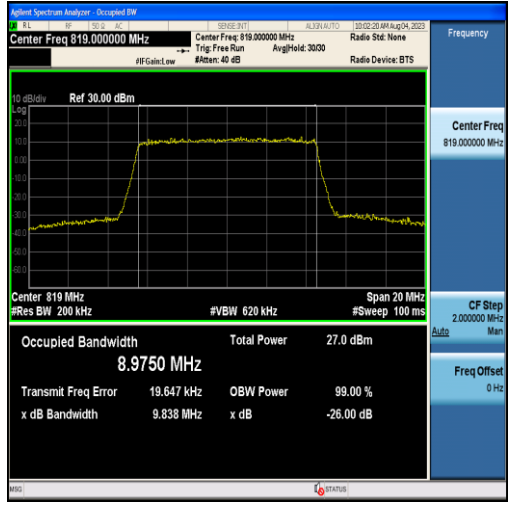
Band26-10MHz-16QAM-26740-50RB#0-8.9750
