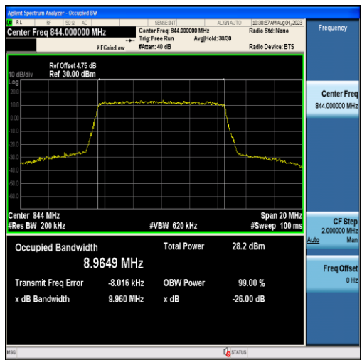
Band26-10MHz-QPSK-26990-50RB#0-8.9649
