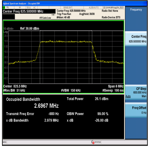
Band26-3MHz-16QAM-26805-15RB#0-2.6967
