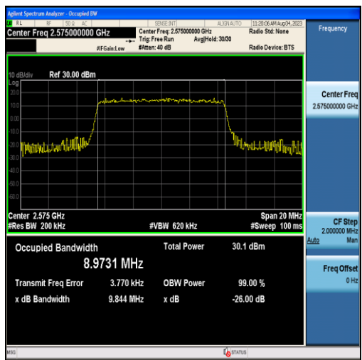
Band38-10MHz-16QAM-37800-50RB#0-8.9731
