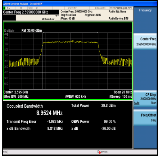
Band38-10MHz-16QAM-38000-50RB#0-8.9524
