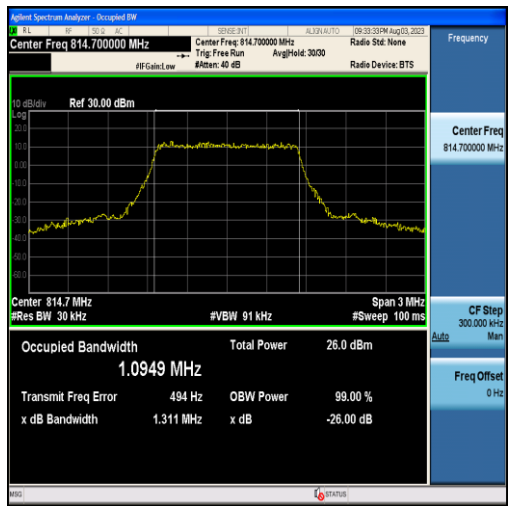
Band26-1.4MHz-16QAM-26697-6RB#0-1.0949
