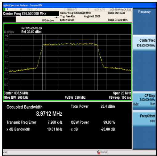
Band26-10MHz-QPSK-26915-50RB#0-8.9712
