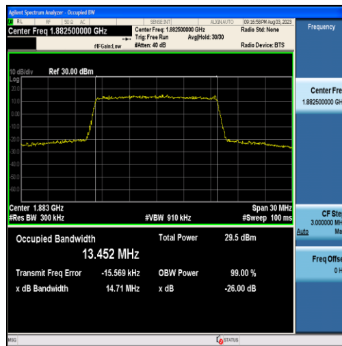
Band25-15MHz-16QAM-26365-75RB#0-13.452
