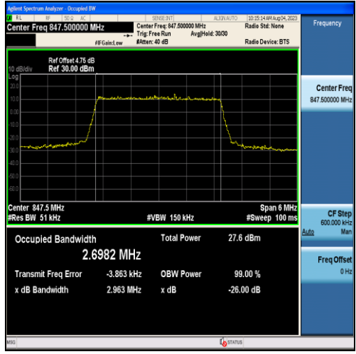
Band26-3MHz-QPSK-27025-15RB#0-2.6982
