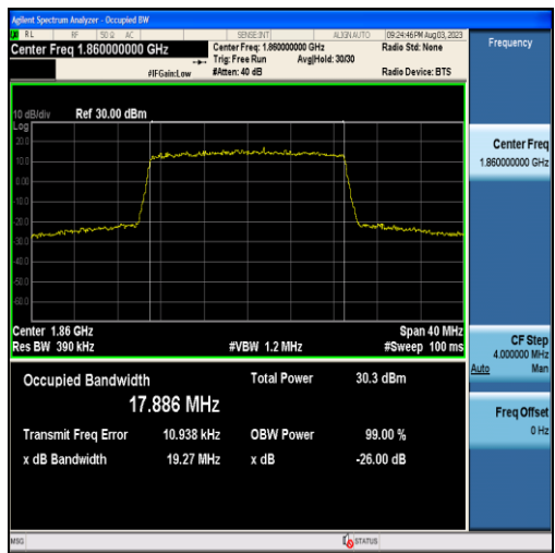
Band25-20MHz-QPSK-26140-100RB#0-17.886
