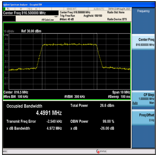
Band26-5MHz-16QAM-26715-25RB#0-4.4991
