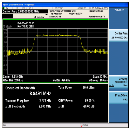
Band38-10MHz-16QAM-38200-50RB#0-8.9491
