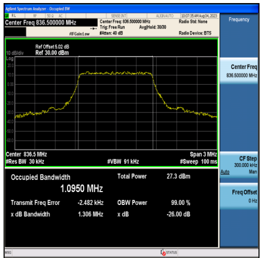
Band26-1.4MHz-QPSK-26915-6RB#0-1.0950
