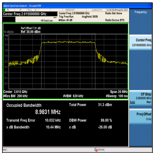
Band38-10MHz-QPSK-38200-50RB#0-8.9831
