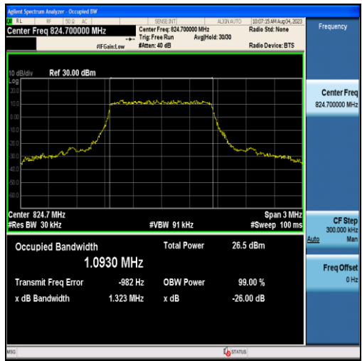
Band26-1.4MHz-QPSK-26797-6RB#0-1.0930
