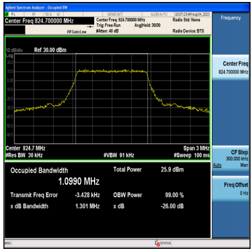
Band26-1.4MHz-16QAM-26797-6RB#0-1.0990
