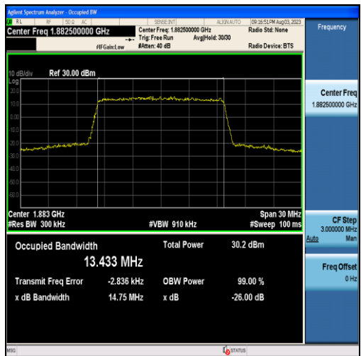
Band25-15MHz-QPSK-26365-75RB#0-13.433
