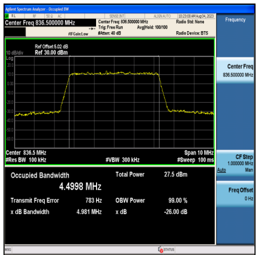
Band26-5MHz-16QAM-26915-25RB#0-4.4998
