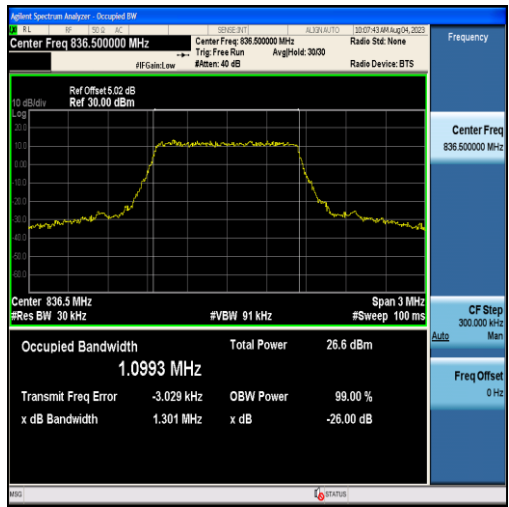
Band26-1.4MHz-16QAM-26915-6RB#0-1.0993
