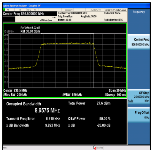
Band26-10MHz-16QAM-26915-50RB#0-8.9575
