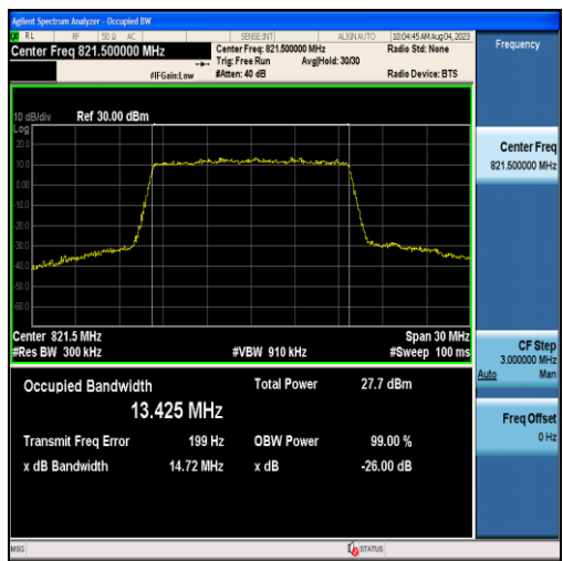
Band26-15MHz-QPSK-26765-75RB#0-13.425
