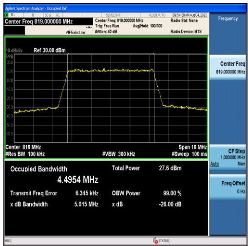
Band26-5MHz-QPSK-26740-25RB#0-4.4954
