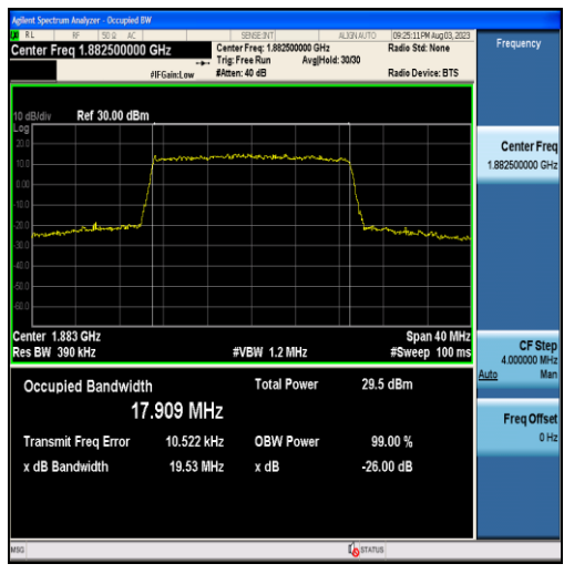
Band25-20MHz-16QAM-26365-100RB#0-17.909
