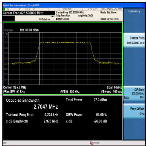
Band26-3MHz-QPSK-26805-15RB#0-2.7047
