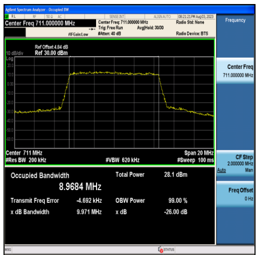
Band12-10MHz-QPSK-23130-50RB#0-8.9684
