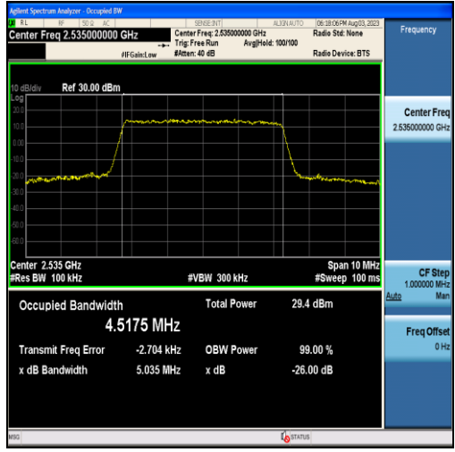
Band7-5MHz-16QAM-21100-25RB#0-4.5175
