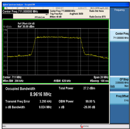
Band12-10MHz-16QAM-23130-50RB#0-8.9616
