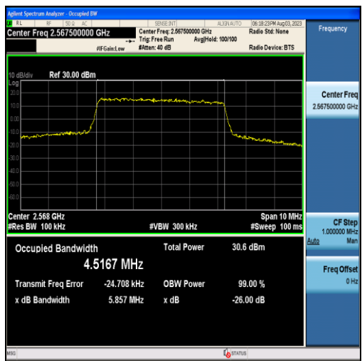
Band7-5MHz-QPSK-21425-25RB#0-4.5167
