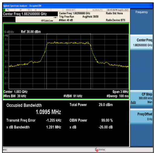
Band25-1.4MHz-QPSK-26365-6RB#0-1.0995
