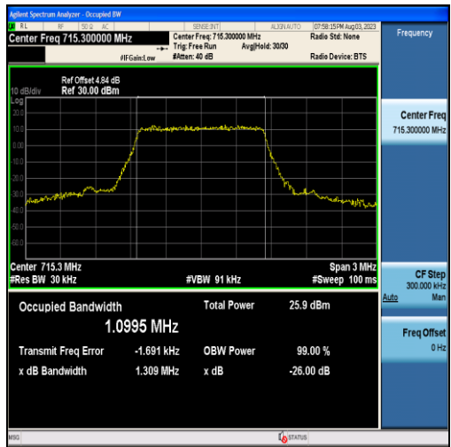
Band12-1.4MHz-16QAM-23173-6RB#0-1.0995
