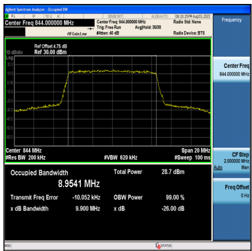
Band5-10MHz-QPSK-20600-50RB#0-8.9541
