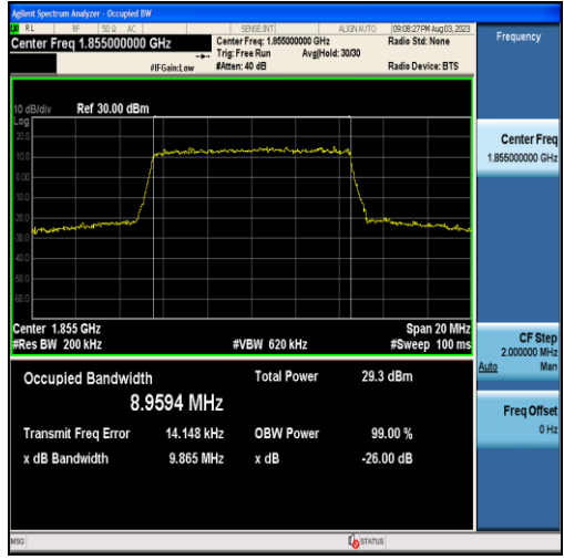
Band25-10MHz-16QAM-26090-50RB#0-8.9594
