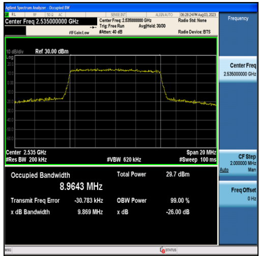
Band7-10MHz-16QAM-21100-50RB#0-8.9643
