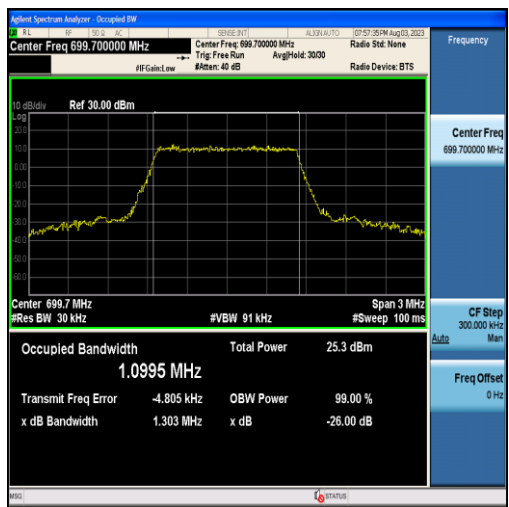
Band12-1.4MHz-16QAM-23017-6RB#0-1.0995
