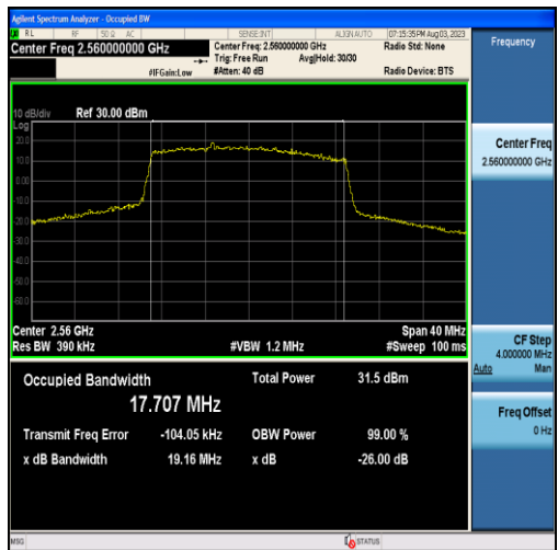
Band7-20MHz-QPSK-21350-100RB#0-17.707
