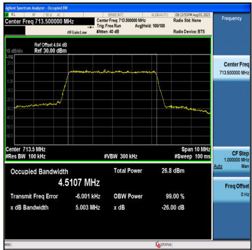
Band12-5MHz-16QAM-23155-25RB#0-4.5107
