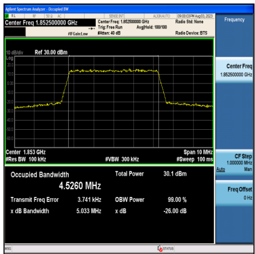
Band25-5MHz-QPSK-26065-25RB#0-4.5260
