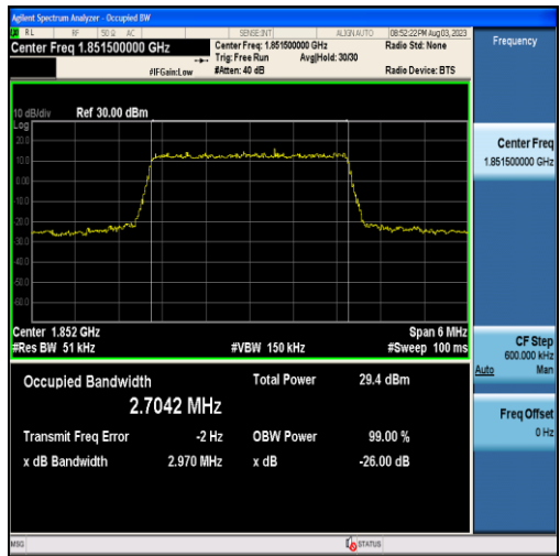
Band25-3MHz-QPSK-26055-15RB#0-2.7042
