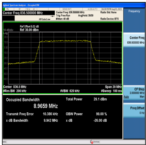
Band5-10MHz-QPSK-20525-50RB#0-8.9659
