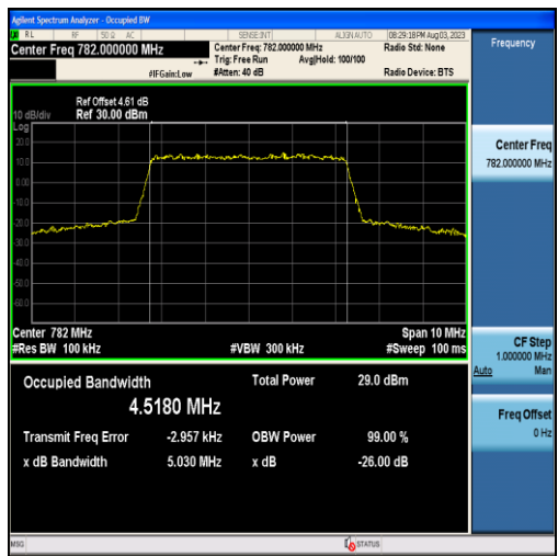
Band13-5MHz-QPSK-23230-25RB#0-4.5180
