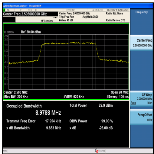
Band7-10MHz-16QAM-20800-50RB#0-8.9788
