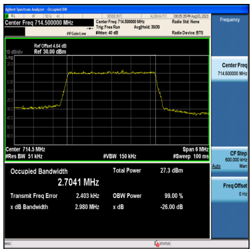
Band12-3MHz-QPSK-23165-15RB#0-2.7041
