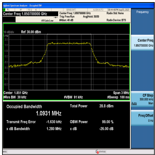
Band25-1.4MHz-QPSK-26047-6RB#0-1.0931
