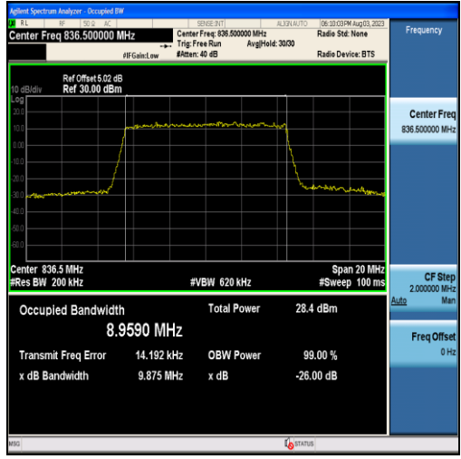
Band5-10MHz-16QAM-20525-50RB#0-8.9590
