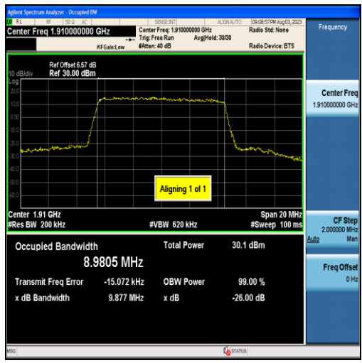
Band25-10MHz-QPSK-26640-50RB#0-8.9805
