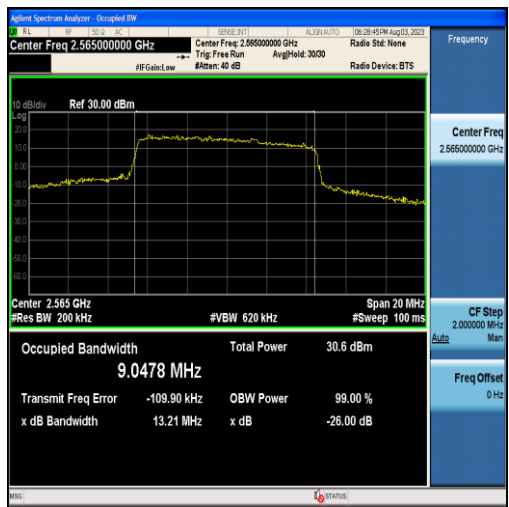
Band7-10MHz-16QAM-21400-50RB#0-9.0478
