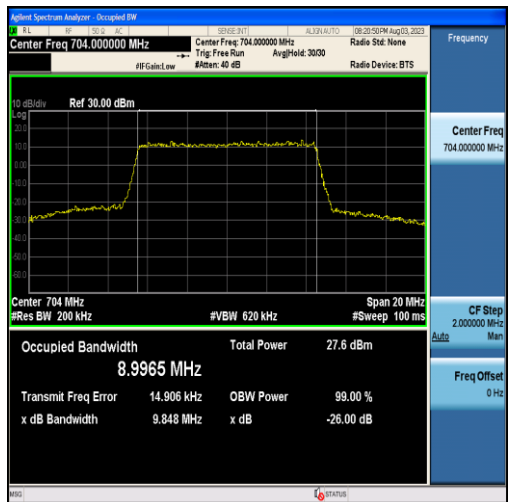
Band12-10MHz-16QAM-23060-50RB#0-8.9965
