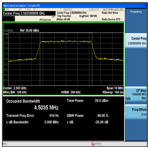
Band7-5MHz-16QAM-20775-25RB#0-4.5035
