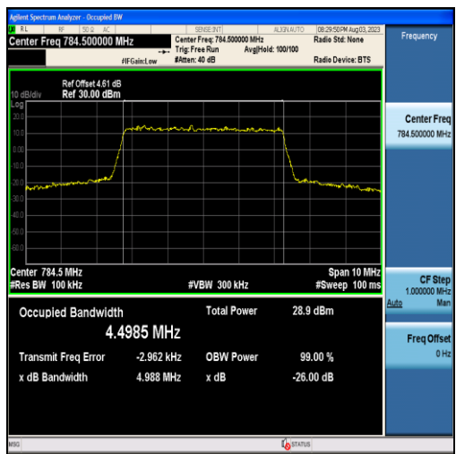
Band13-5MHz-QPSK-23255-25RB#0-4.4985
