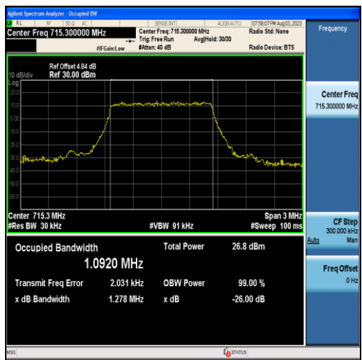
Band12-1.4MHz-QPSK-23173-6RB#0-1.0920
