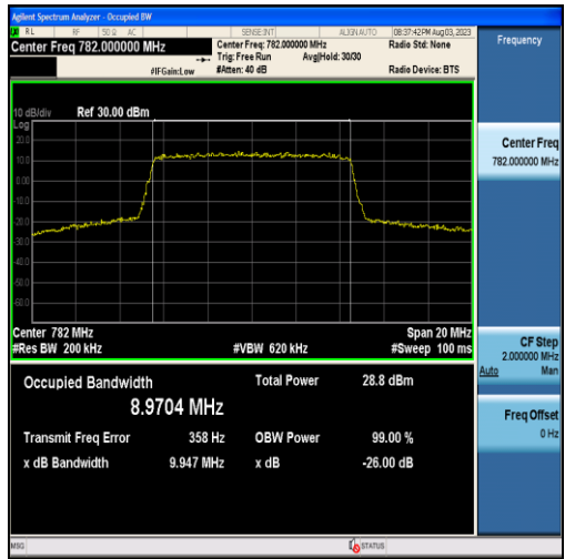
Band13-10MHz-QPSK-23230-50RB#0-8.9704
