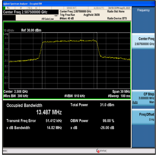
Band7-15MHz-QPSK-20825-75RB#0-13.487
