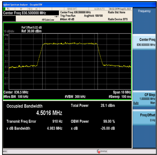
Band5-5MHz-16QAM-20525-25RB#0-4.5016
