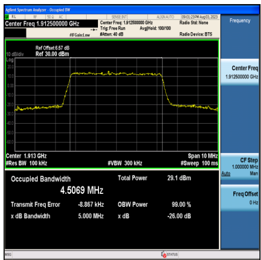
Band25-5MHz-16QAM-26665-25RB#0-4.5069
