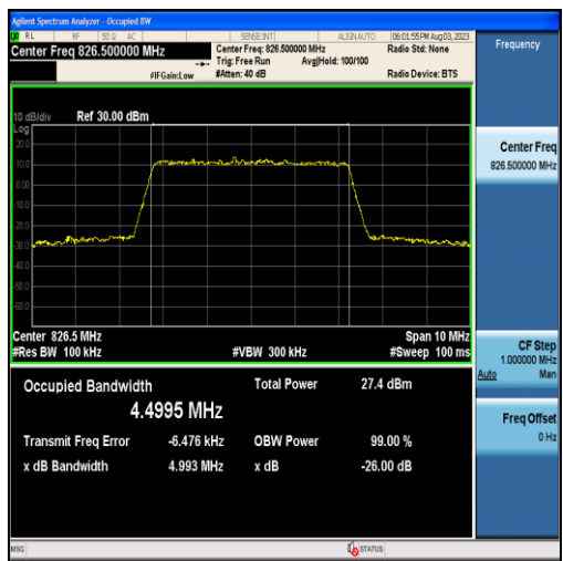
Band5-5MHz-16QAM-20425-25RB#0-4.4995
