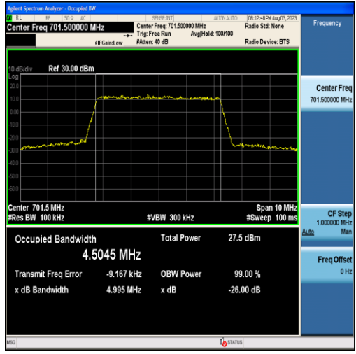
Band12-5MHz-16QAM-23035-25RB#0-4.5045
