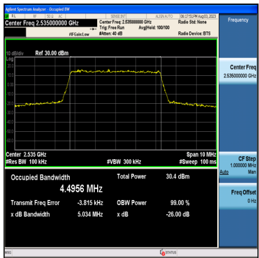
Band7-5MHz-QPSK-21100-25RB#0-4.4956
