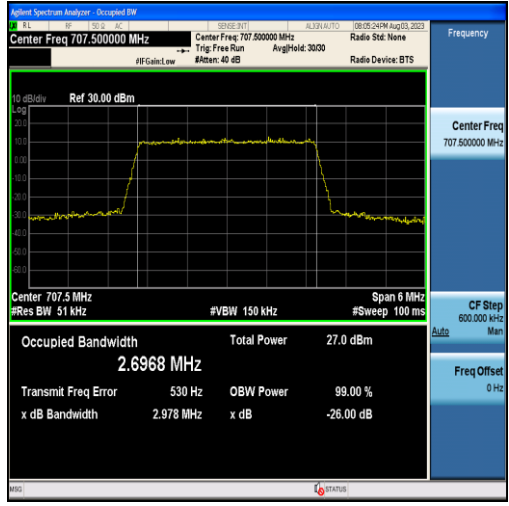
Band12-3MHz-16QAM-23095-15RB#0-2.6968
