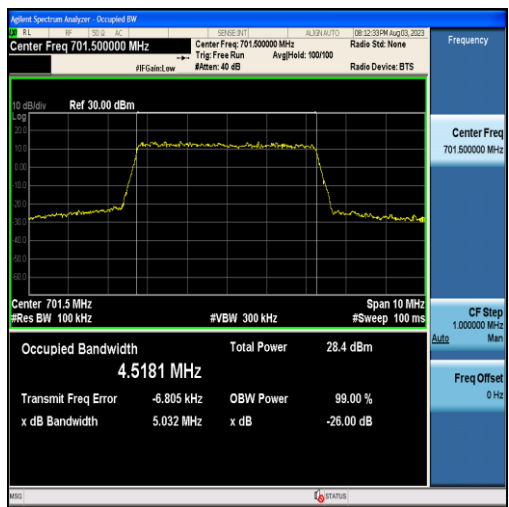
Band12-5MHz-QPSK-23035-25RB#0-4.5181
