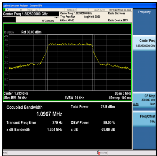
Band25-1.4MHz-16QAM-26365-6RB#0-1.0967
