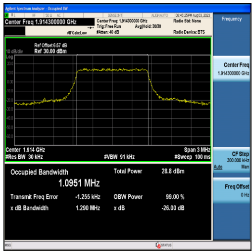
Band25-1.4MHz-QPSK-26683-6RB#0-1.0951
