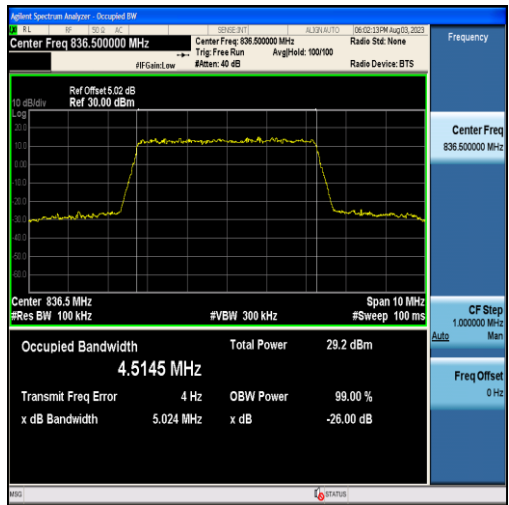
Band5-5MHz-QPSK-20525-25RB#0-4.5145
