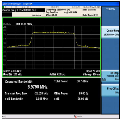
Band7-10MHz-QPSK-21100-50RB#0-8.9790
