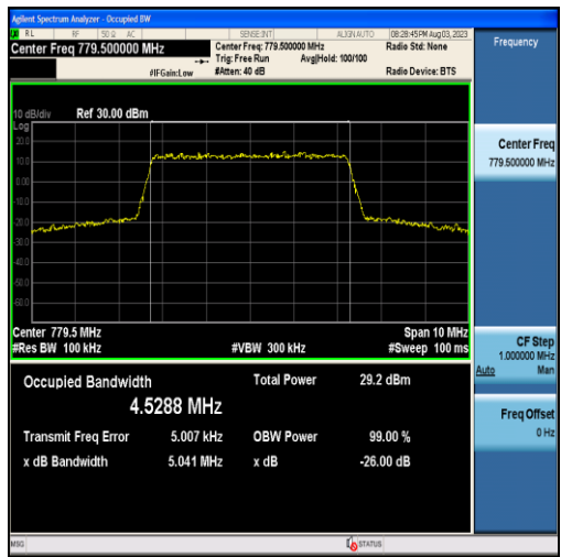
Band13-5MHz-QPSK-23205-25RB#0-4.5288
