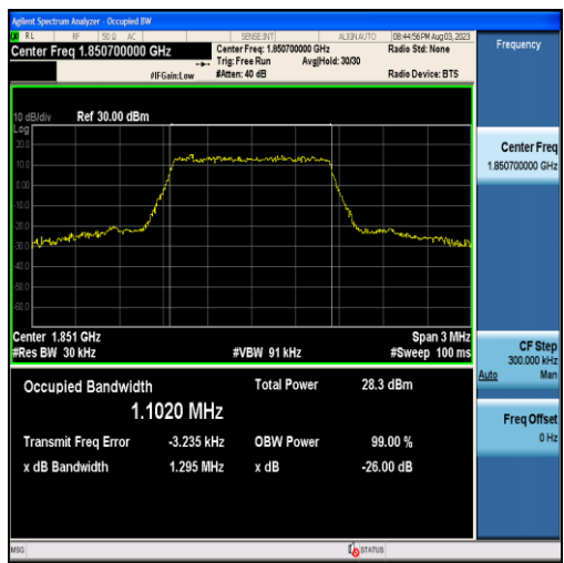
Band25-1.4MHz-16QAM-26047-6RB#0-1.1020
