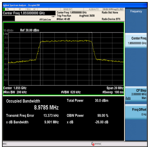
Band25-10MHz-QPSK-26090-50RB#0-8.9785
