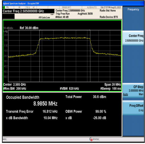
Band7-10MHz-QPSK-20800-50RB#0-8.9850
