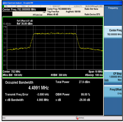
Band13-5MHz-16QAM-23230-25RB#0-4.4991
