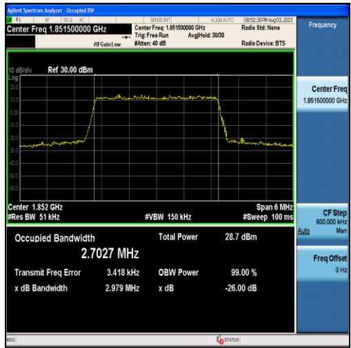
Band25-3MHz-16QAM-26055-15RB#0-2.7027
