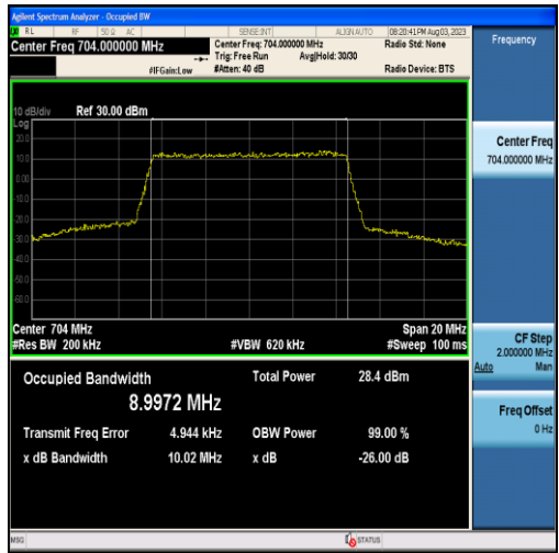
Band12-10MHz-QPSK-23060-50RB#0-8.9972
