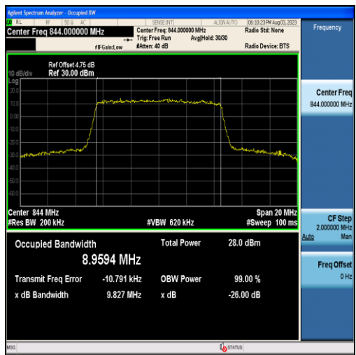
Band5-10MHz-16QAM-20600-50RB#0-8.9594
