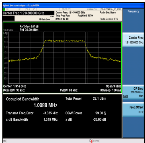
Band25-1.4MHz-16QAM-26683-6RB#0-1.0988
