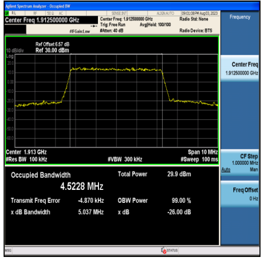
Band25-5MHz-QPSK-26665-25RB#0-4.5228
