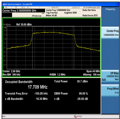
Band7-20MHz-16QAM-21350-100RB#0-17.709
