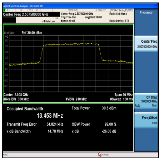
Band7-15MHz-16QAM-20825-75RB#0-13.453
