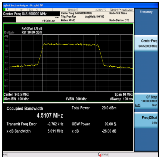
Band5-5MHz-QPSK-20625-25RB#0-4.5107
