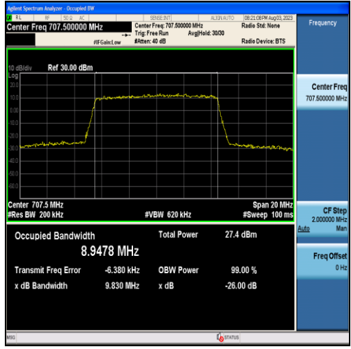
Band12-10MHz-16QAM-23095-50RB#0-8.9478
