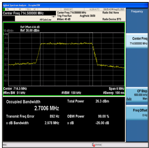
Band12-3MHz-16QAM-23165-15RB#0-2.7006
