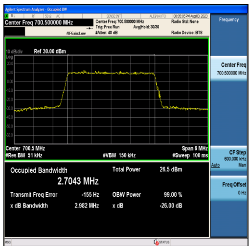
Band12-3MHz-16QAM-23025-15RB#0-2.7043
