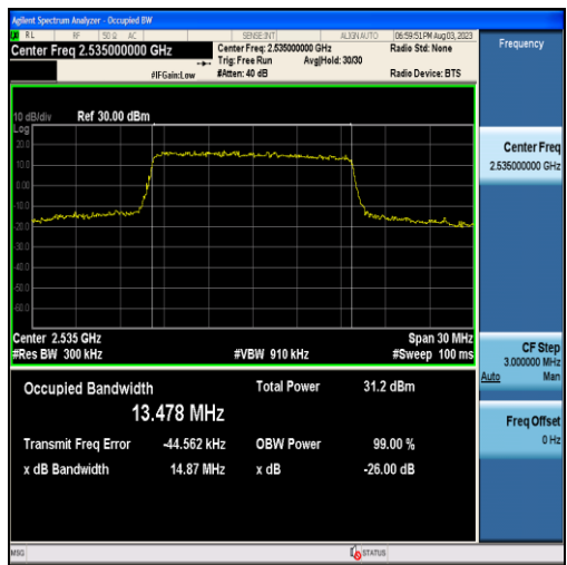
Band7-15MHz-QPSK-21100-75RB#0-13.478
