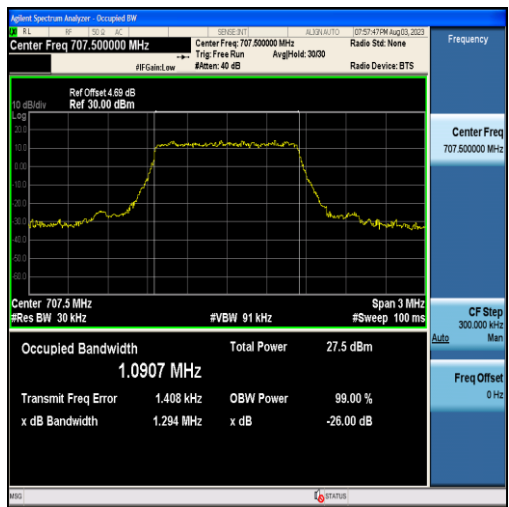
Band12-1.4MHz-QPSK-23095-6RB#0-1.0907
