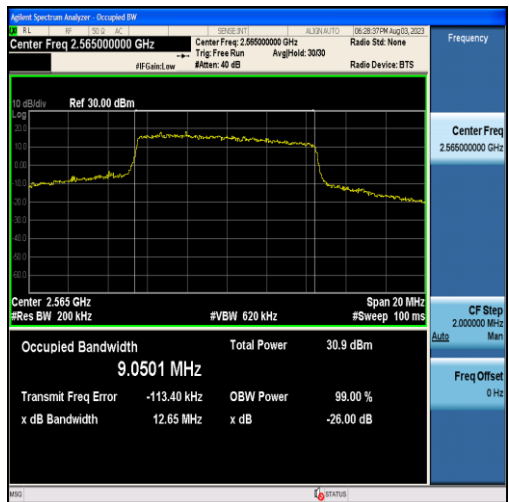
Band7-10MHz-QPSK-21400-50RB#0-9.0501
