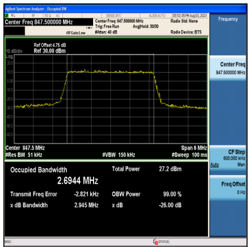
Band5-3MHz-16QAM-20635-15RB#0-2.6944
