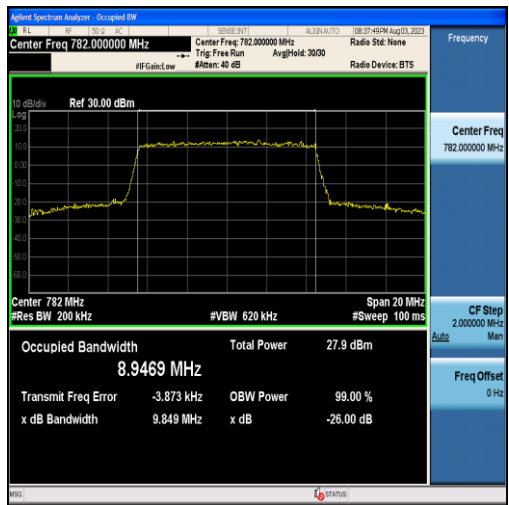
Band13-10MHz-16QAM-23230-50RB#0-8.9469
