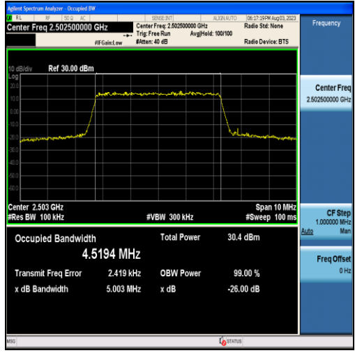
Band7-5MHz-QPSK-20775-25RB#0-4.5194
