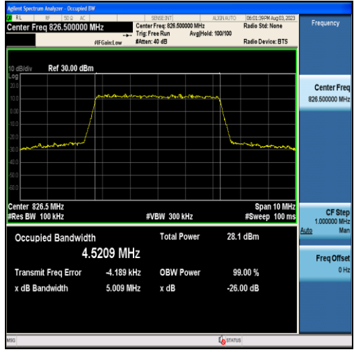
Band5-5MHz-QPSK-20425-25RB#0-4.5209
