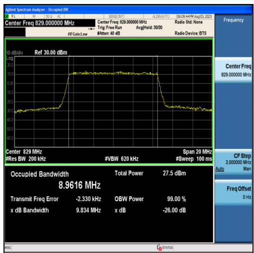
Band5-10MHz-16QAM-20450-50RB#0-8.9616
