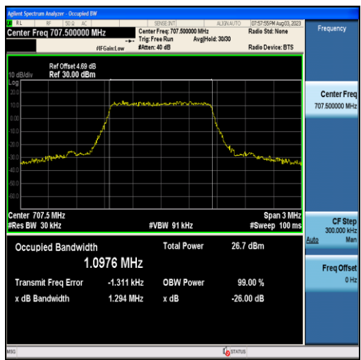
Band12-1.4MHz-16QAM-23095-6RB#0-1.0976
