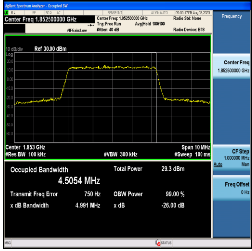
Band25-5MHz-16QAM-26065-25RB#0-4.5054
