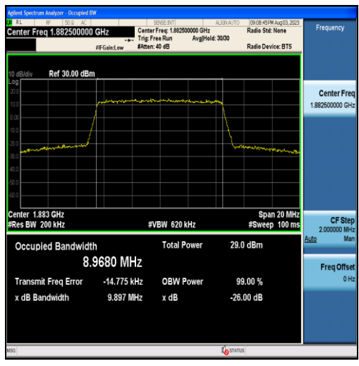
Band25-10MHz-16QAM-26365-50RB#0-8.9680
