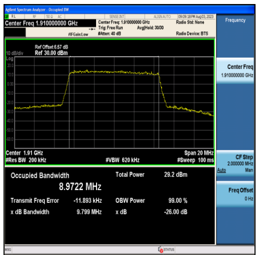
Band25-10MHz-16QAM-26640-50RB#0-8.9722
