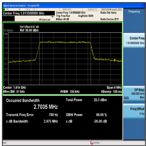
Band25-3MHz-16QAM-26675-15RB#0-2.7035
