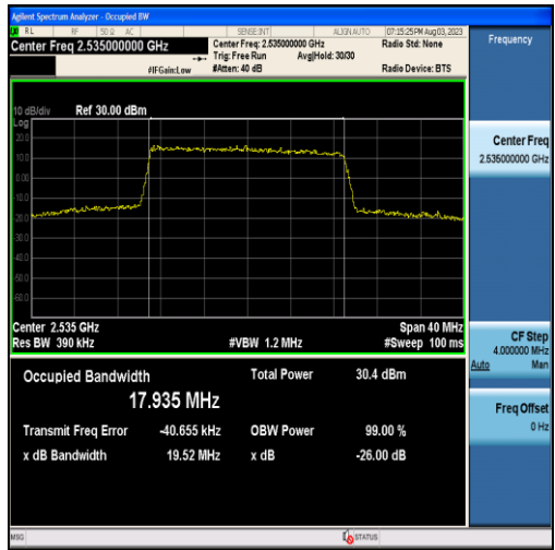
Band7-20MHz-16QAM-21100-100RB#0-17.935
