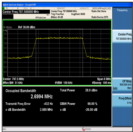
Band12-3MHz-QPSK-23095-15RB#0-2.6994
