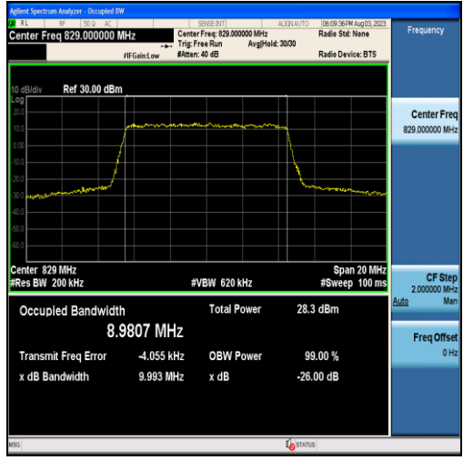
Band5-10MHz-QPSK-20450-50RB#0-8.9807
