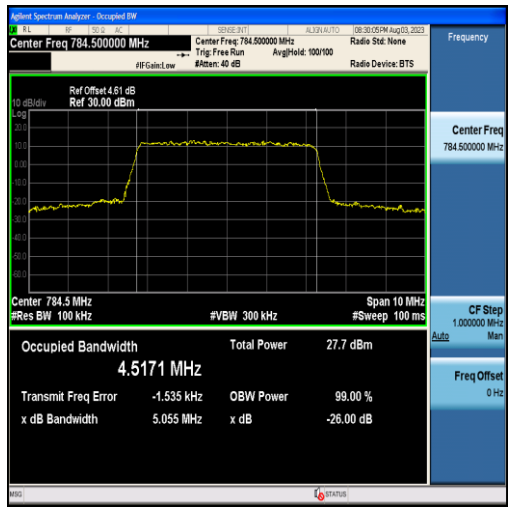
Band13-5MHz-16QAM-23255-25RB#0-4.5171
