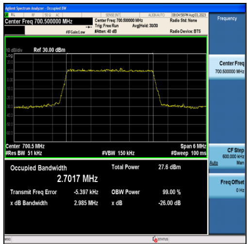
Band12-3MHz-QPSK-23025-15RB#0-2.7017
