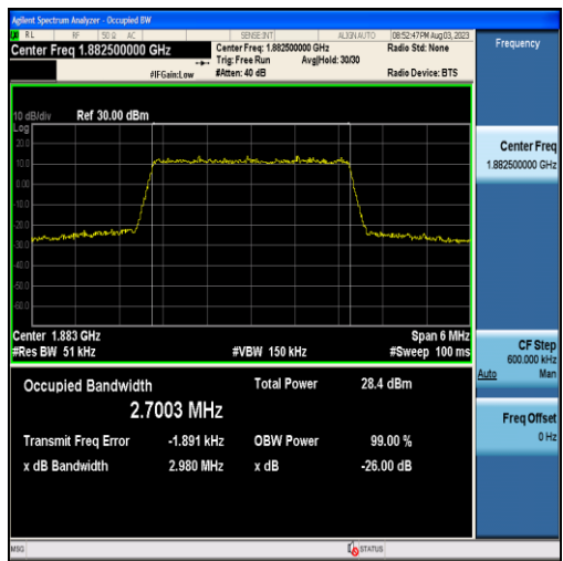
Band25-3MHz-16QAM-26365-15RB#0-2.7003
