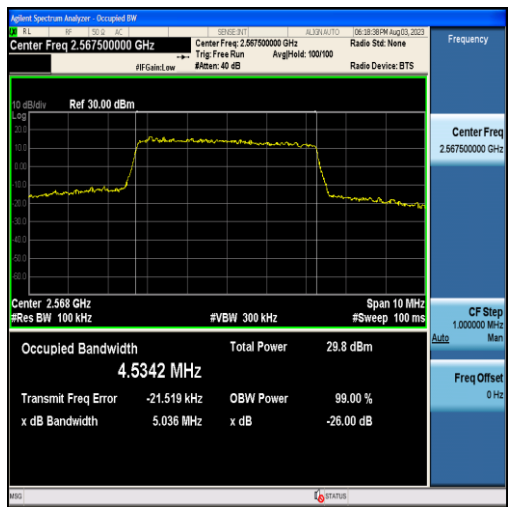
Band7-5MHz-16QAM-21425-25RB#0-4.5342
