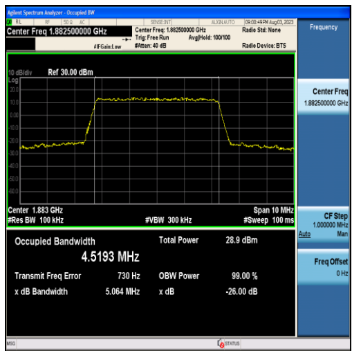
Band25-5MHz-16QAM-26365-25RB#0-4.5193
