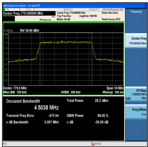
Band13-5MHz-16QAM-23205-25RB#0-4.5038
