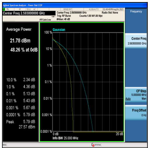
Band41-15MHz-QPSK-40620-75RB#0
