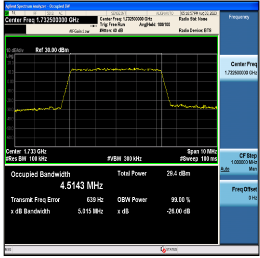
Band4-5MHz-16QAM-20175-25RB#0-4.5143
