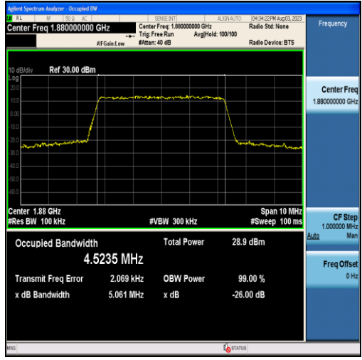
Band2-5MHz-16QAM-18900-25RB#0-4.5235
