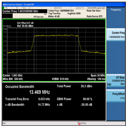
Band2-15MHz-16QAM-19125-75RB#0-13.469
