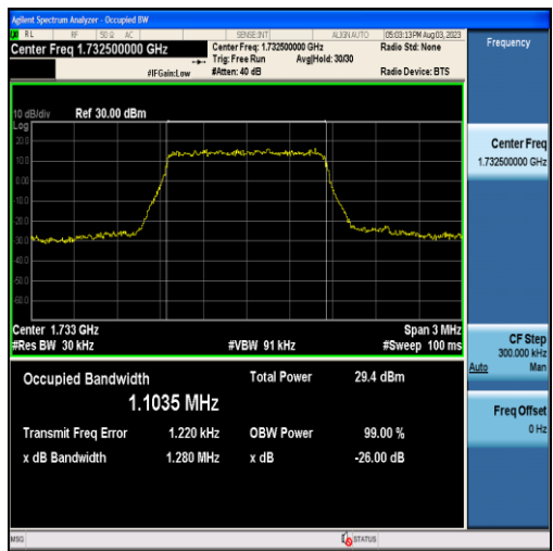
Band4-1.4MHz-QPSK-20175-6RB#0-1.1035
