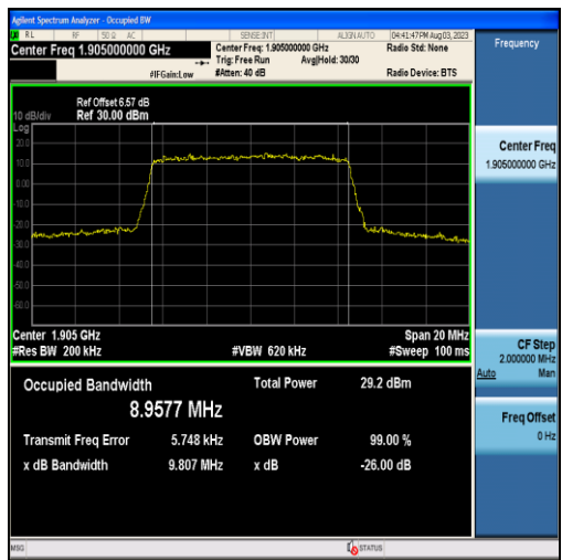
Band2-10MHz-16QAM-19150-50RB#0-8.9577
