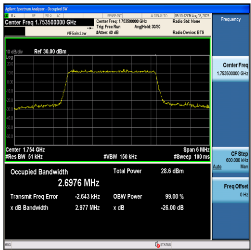
Band4-3MHz-16QAM-20385-15RB#0-2.6976
