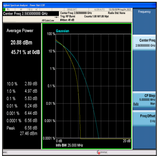
Band41-15MHz-16QAM-40620-75RB#0
