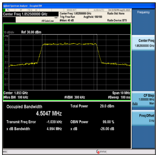
Band2-5MHz-16QAM-18625-25RB#0-4.5047
