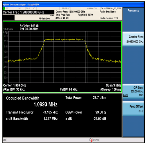
Band2-1.4MHz-16QAM-19193-6RB#0-1.0993
