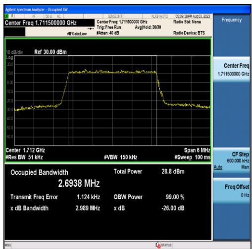
Band4-3MHz-16QAM-19965-15RB#0-2.6938
