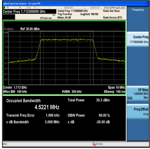
Band4-5MHz-QPSK-19975-25RB#0-4.5221
