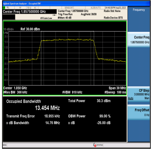
Band2-15MHz-QPSK-18675-75RB#0-13.454
