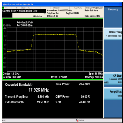
Band2-20MHz-16QAM-19100-100RB#0-17.926
