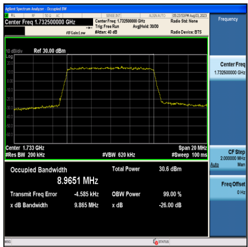
Band4-10MHz-QPSK-20175-50RB#0-8.9651
