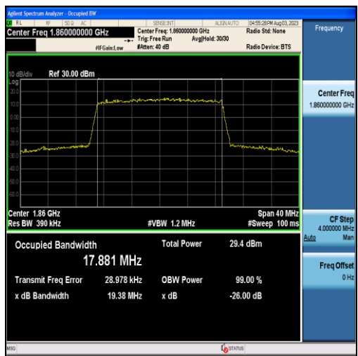
Band2-20MHz-16QAM-18700-100RB#0-17.881
