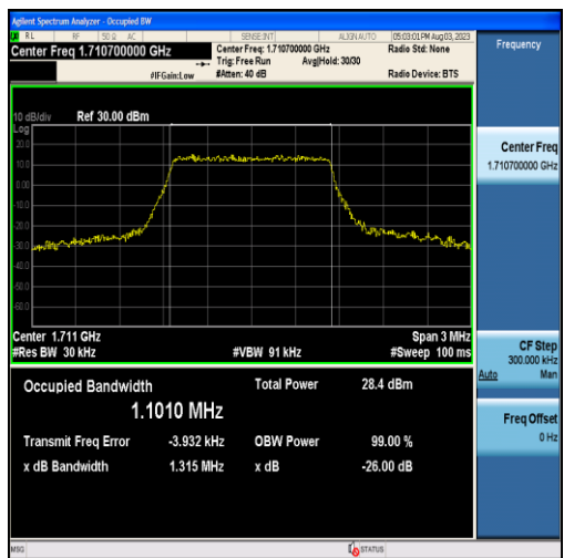
Band4-1.4MHz-16QAM-19957-6RB#0-1.1010
