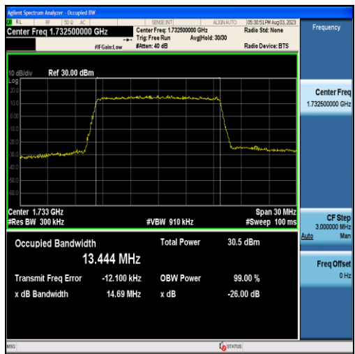
Band4-15MHz-QPSK-20175-75RB#0-13.444
