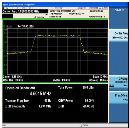
Band2-5MHz-QPSK-18900-25RB#0-4.5015
