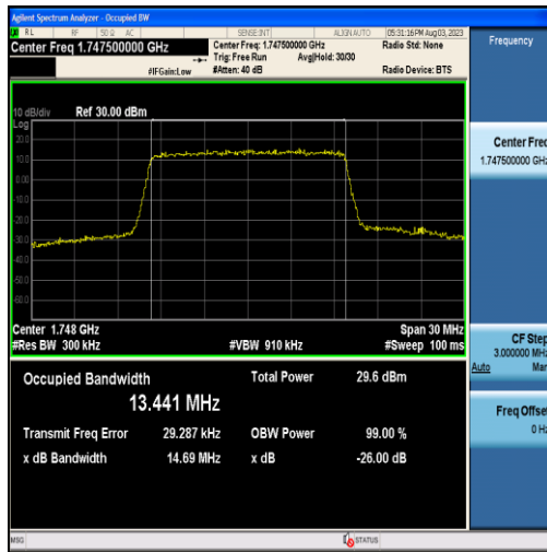
Band4-15MHz-16QAM-20325-75RB#0-13.441
