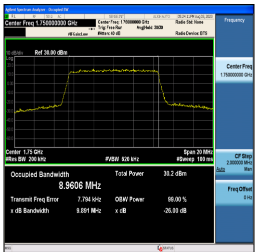
Band4-10MHz-QPSK-20350-50RB#0-8.9606
