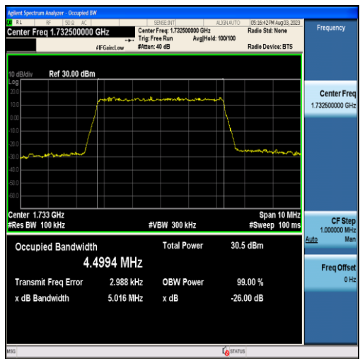
Band4-5MHz-QPSK-20175-25RB#0-4.4994
