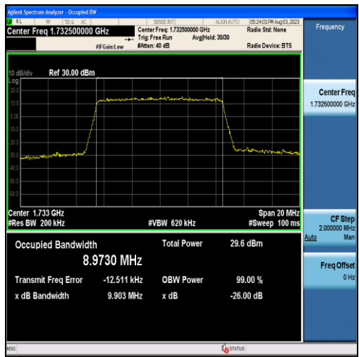
Band4-10MHz-16QAM-20175-50RB#0-8.9730
