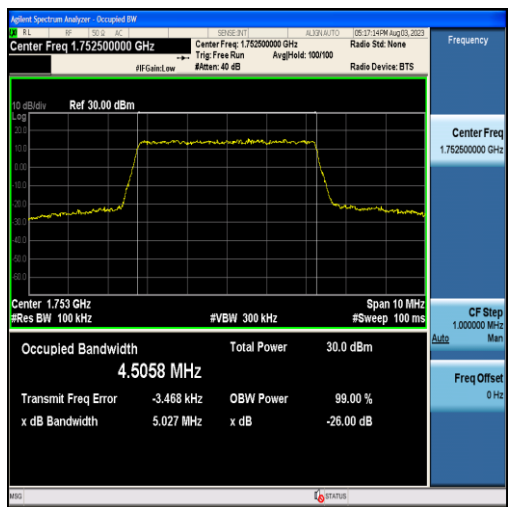
Band4-5MHz-QPSK-20375-25RB#0-4.5058
