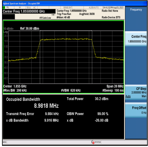
Band2-10MHz-QPSK-18650-50RB#0-8.9818
