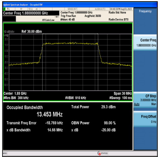
Band2-15MHz-16QAM-18900-75RB#0-13.453
