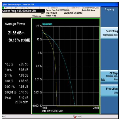
Band41-15MHz-QPSK-41515-75RB#0
