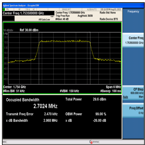
Band4-3MHz-QPSK-20385-15RB#0-2.7024
