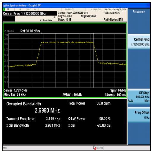
Band4-3MHz-QPSK-20175-15RB#0-2.6983
