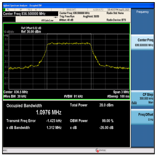
Band5-1.4MHz-QPSK-20525-6RB#0-1.0976
