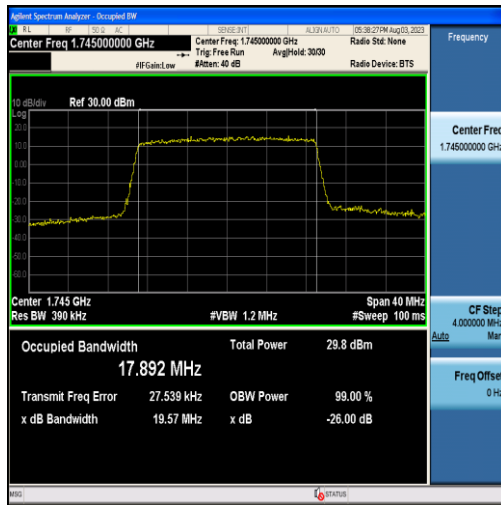
Band4-20MHz-16QAM-20300-100RB#0-17.892
