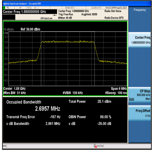
Band2-3MHz-16QAM-18900-15RB#0-2.6957
