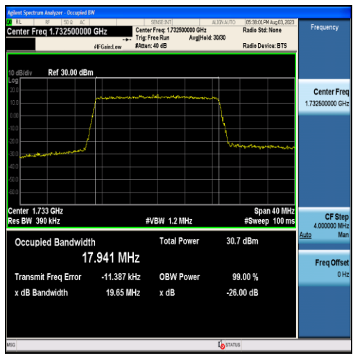
Band4-20MHz-QPSK-20175-100RB#0-17.941
