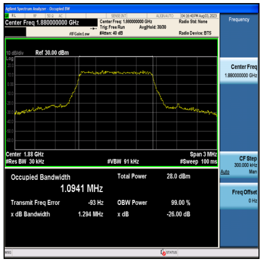
Band2-1.4MHz-16QAM-18900-6RB#0-1.0941
