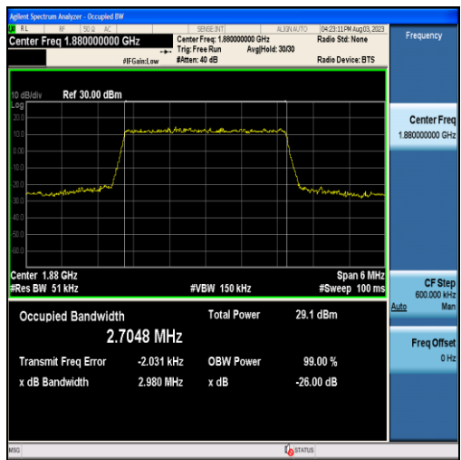
Band2-3MHz-QPSK-18900-15RB#0-2.7048
