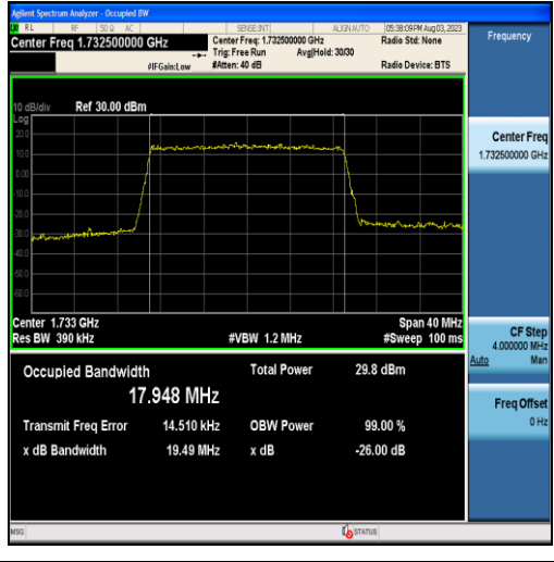
Band4-20MHz-16QAM-20175-100RB#0-17.948
