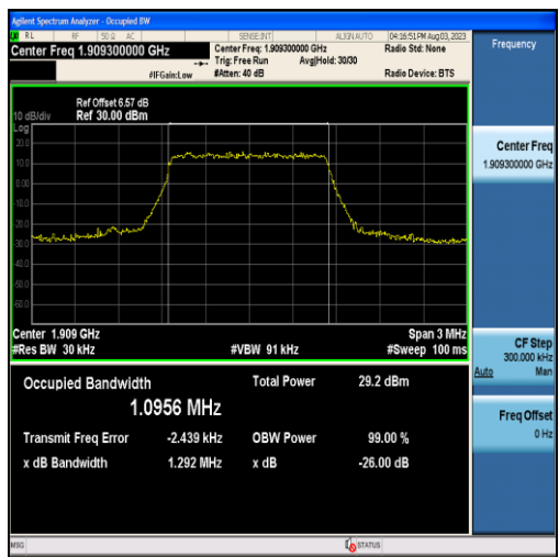
Band2-1.4MHz-QPSK-19193-6RB#0-1.0956
