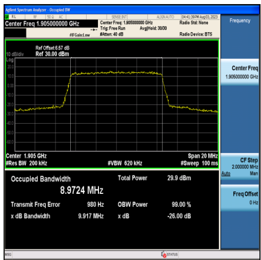
Band2-10MHz-QPSK-19150-50RB#0-8.9724
