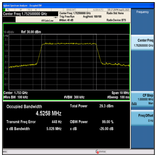
Band4-5MHz-16QAM-20375-25RB#0-4.5258
