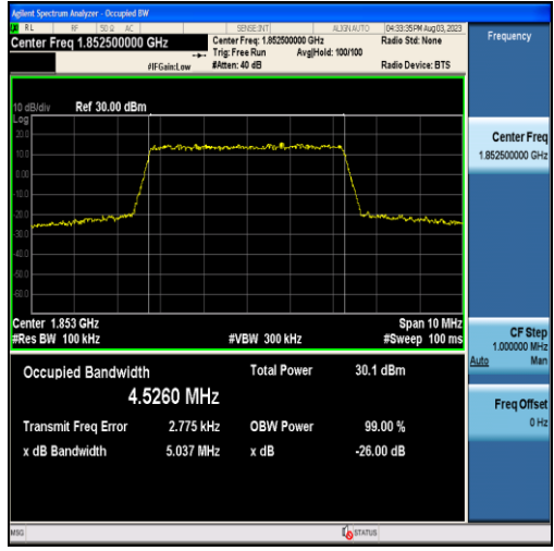
Band2-5MHz-QPSK-18625-25RB#0-4.5260
