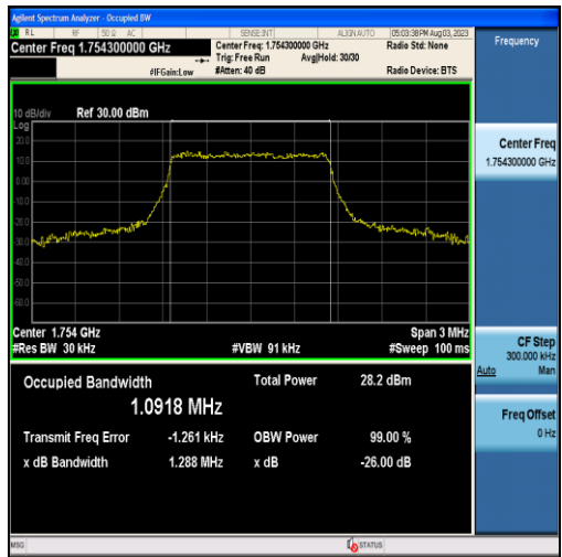
Band4-1.4MHz-16QAM-20393-6RB#0-1.0918
