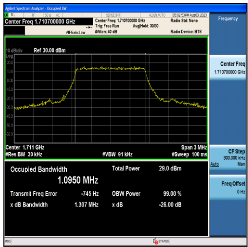
Band4-1.4MHz-QPSK-19957-6RB#0-1.0950
