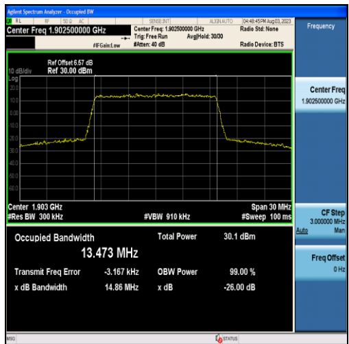
Band2-15MHz-QPSK-19125-75RB#0-13.473
