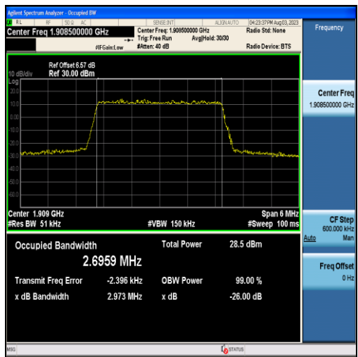
Band2-3MHz-16QAM-19185-15RB#0-2.6959
