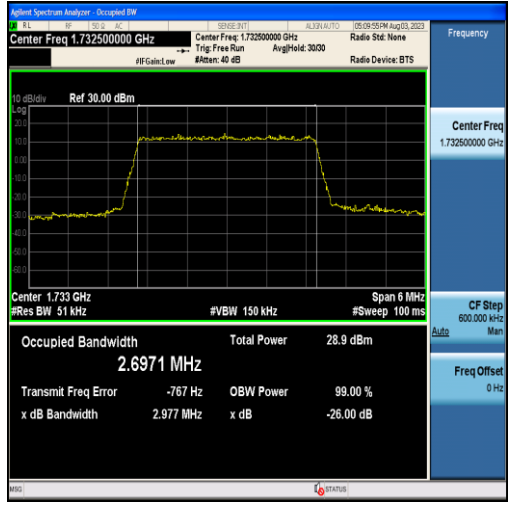
Band4-3MHz-16QAM-20175-15RB#0-2.6971
