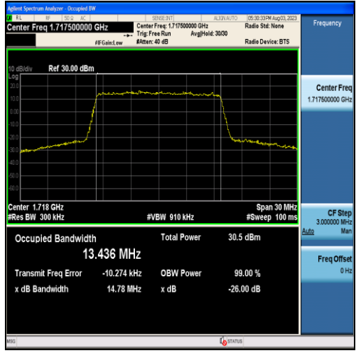
Band4-15MHz-QPSK-20025-75RB#0-13.436
