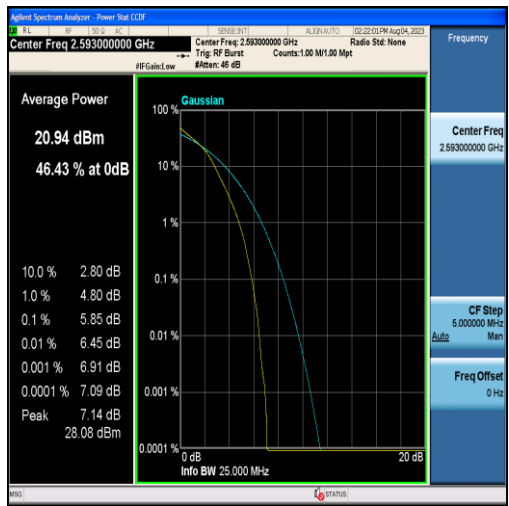
Band41-20MHz-16QAM-40620-100RB#0
