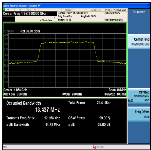
Band2-15MHz-16QAM-18675-75RB#0-13.437
