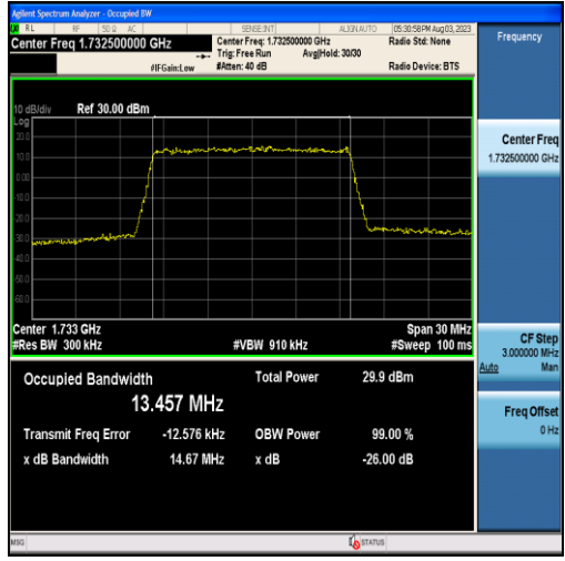
Band4-15MHz-16QAM-20175-75RB#0-13.457
