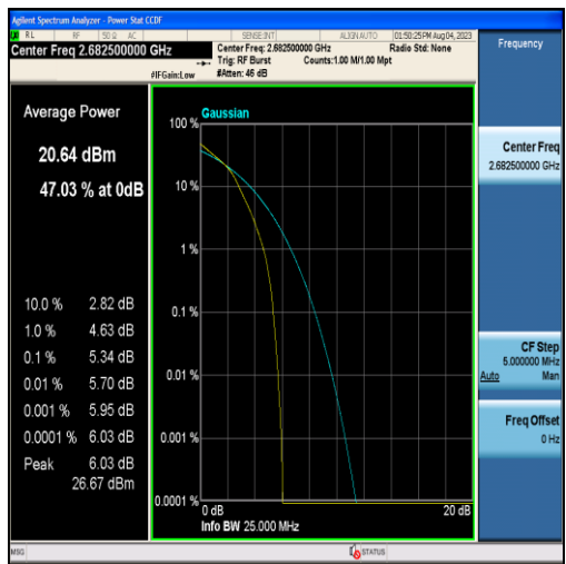
Band41-15MHz-16QAM-41515-75RB#0
