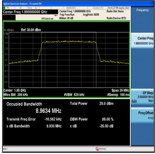
Band2-10MHz-16QAM-18900-50RB#0-8.9634
