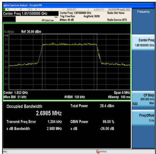
Band2-3MHz-16QAM-18615-15RB#0-2.6985
