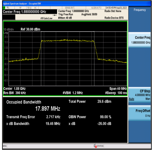
Band2-20MHz-16QAM-18900-100RB#0-17.897
