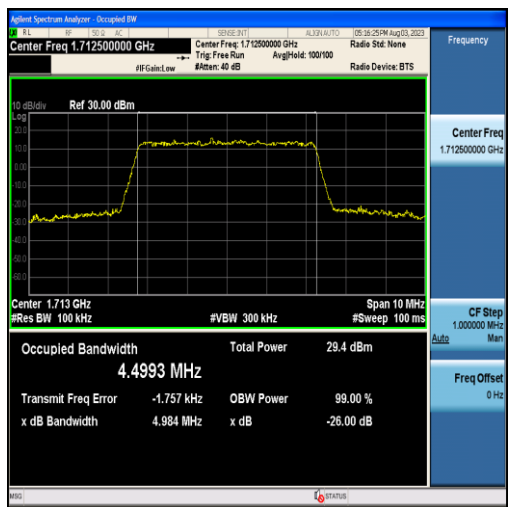
Band4-5MHz-16QAM-19975-25RB#0-4.4993
