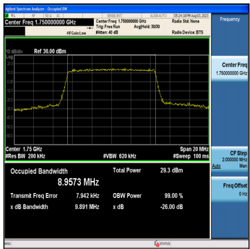
Band4-10MHz-16QAM-20350-50RB#0-8.9573
