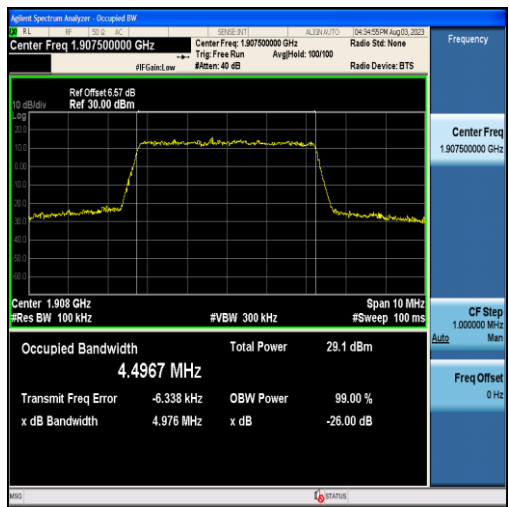
Band2-5MHz-16QAM-19175-25RB#0-4.4967
