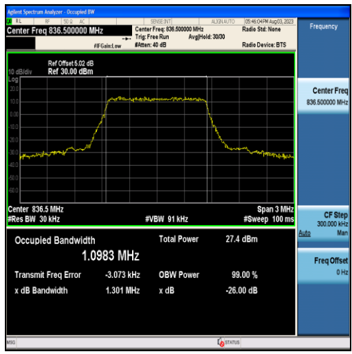
Band5-1.4MHz-16QAM-20525-6RB#0-1.0983
