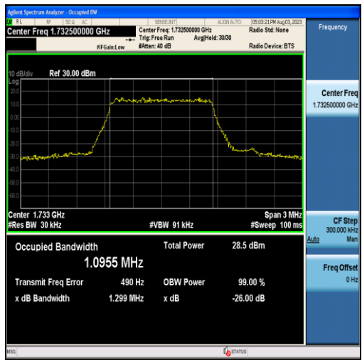
Band4-1.4MHz-16QAM-20175-6RB#0-1.0955
