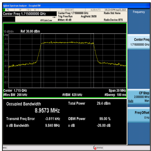
Band4-10MHz-16QAM-20000-50RB#0-8.9573
