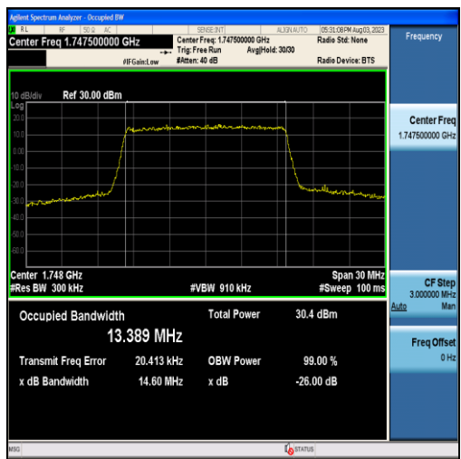
Band4-15MHz-QPSK-20325-75RB#0-13.389
