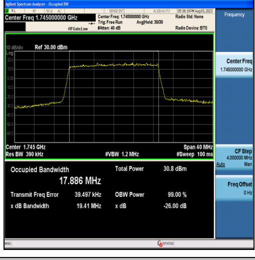
Band4-20MHz-QPSK-20300-100RB#0-17.886
