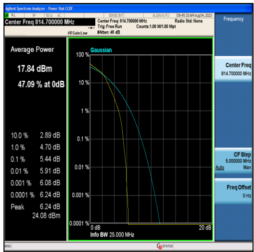
Band26-1.4MHz-16QAM-26697-6RB#0
