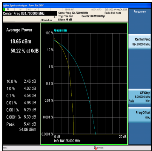
Band26-1.4MHz-QPSK-26797-6RB#0
