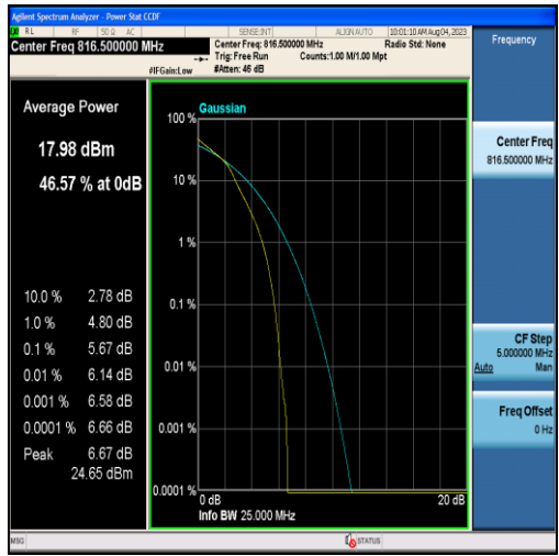
Band26-5MHz-16QAM-26715-25RB#0
