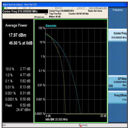
Band26-5MHz-16QAM-26740-25RB#0
