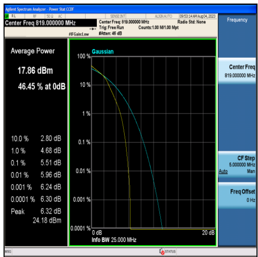
Band26-3MHz-16QAM-26740-15RB#0
