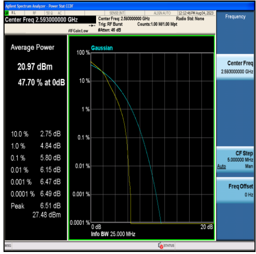
Band41-5MHz-16QAM-40620-25RB#0
