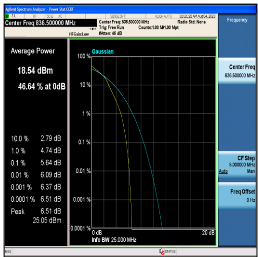
Band26-3MHz-16QAM-26915-15RB#0
