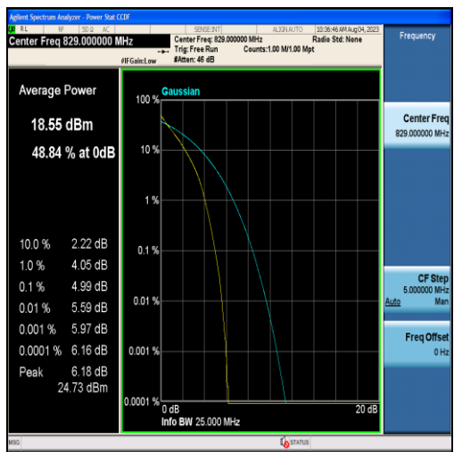
Band26-10MHz-QPSK-26840-50RB#0
