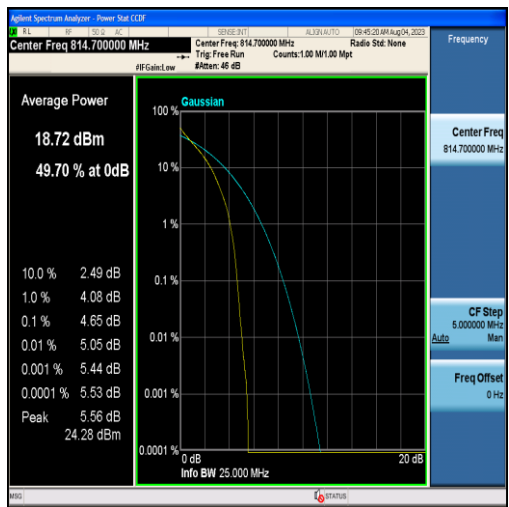
Band26-1.4MHz-QPSK-26697-6RB#0
