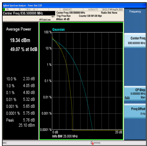
Band26-3MHz-QPSK-26915-15RB#0
