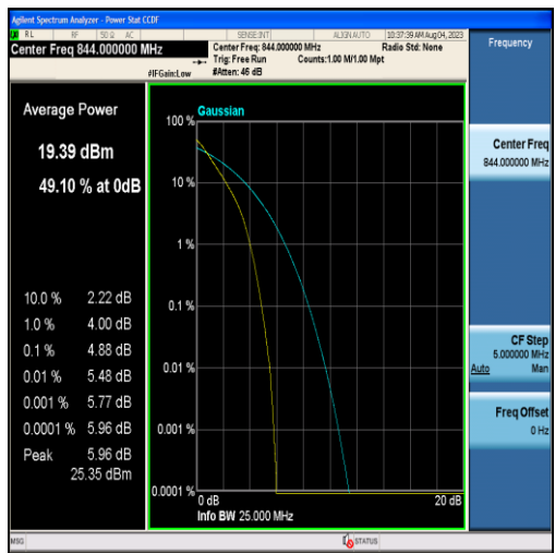
Band26-10MHz-QPSK-26990-50RB#0
