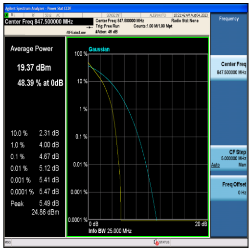
Band26-3MHz-QPSK-27025-15RB#0
