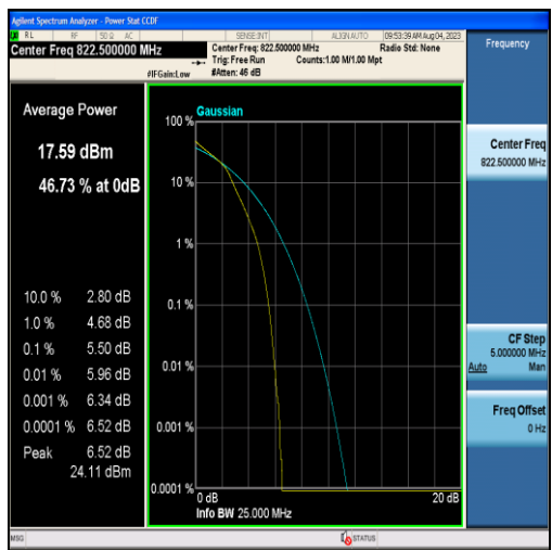
Band26-3MHz-16QAM-26775-15RB#0
