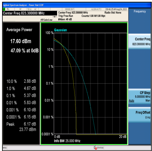
Band26-1.4MHz-16QAM-26783-6RB#0
