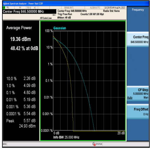
Band26-5MHz-QPSK-27015-25RB#0
