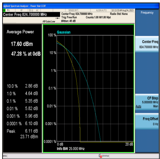
Band26-1.4MHz-16QAM-26797-6RB#0
