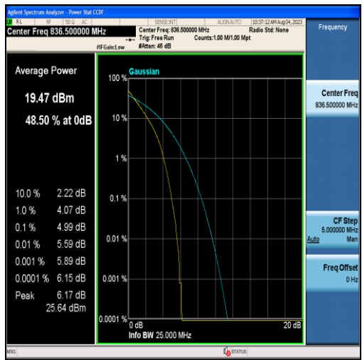
Band26-10MHz-QPSK-26915-50RB#0
