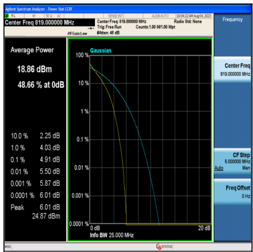
Band26-10MHz-QPSK-26740-50RB#0
