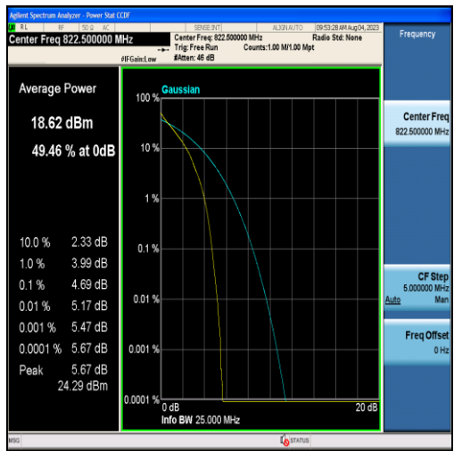
Band26-3MHz-QPSK-26775-15RB#0
