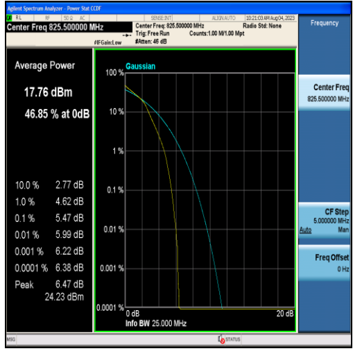
Band26-3MHz-16QAM-26805-15RB#0
