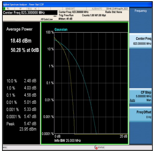
Band26-1.4MHz-QPSK-26783-6RB#0
