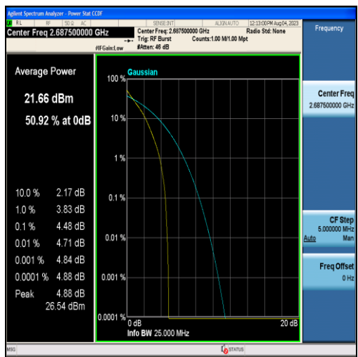
Band41-5MHz-QPSK-41565-25RB#0
