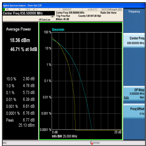
Band26-10MHz-16QAM-26915-50RB#0
