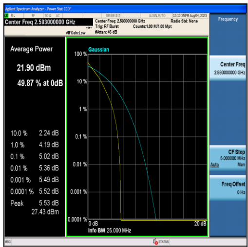
Band41-5MHz-QPSK-40620-25RB#0
