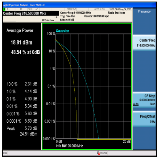
Band26-5MHz-QPSK-26715-25RB#0
