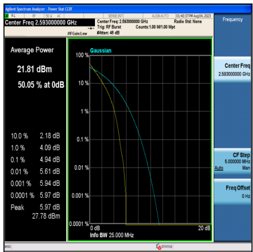
Band41-10MHz-QPSK-40620-50RB#0
