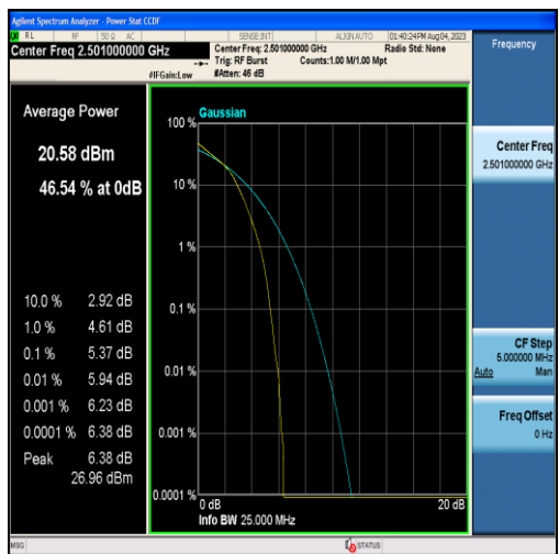
Band41-10MHz-16QAM-39700-50RB#0
