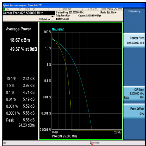
Band26-3MHz-QPSK-26805-15RB#0
