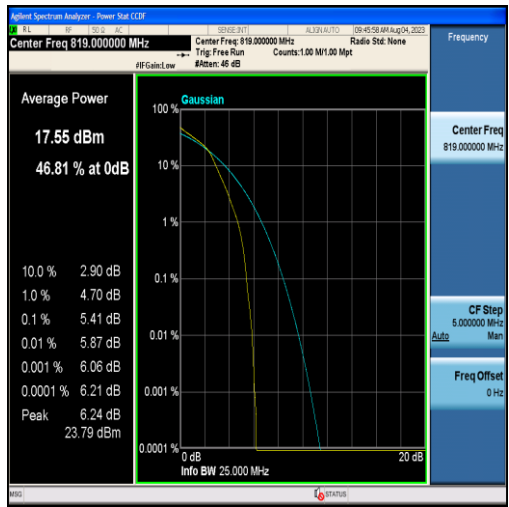
Band26-1.4MHz-16QAM-26740-6RB#0
