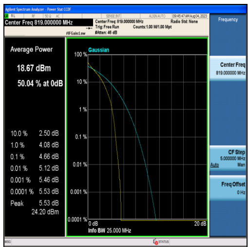
Band26-1.4MHz-QPSK-26740-6RB#0
