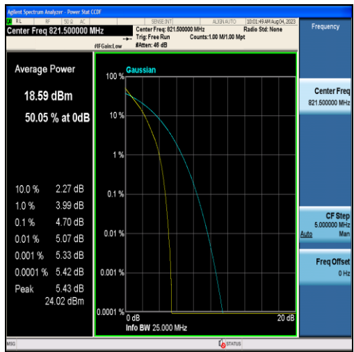
Band26-5MHz-QPSK-26765-25RB#0
