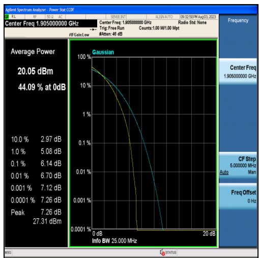
Band25-20MHz-16QAM-26590-100RB#0
