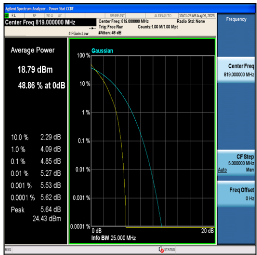
Band26-5MHz-QPSK-26740-25RB#0
