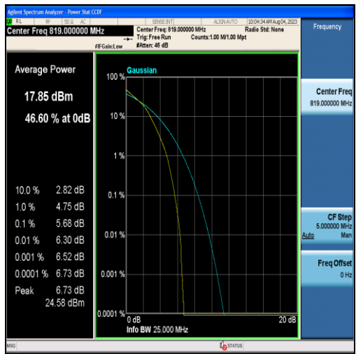
Band26-10MHz-16QAM-26740-50RB#0
