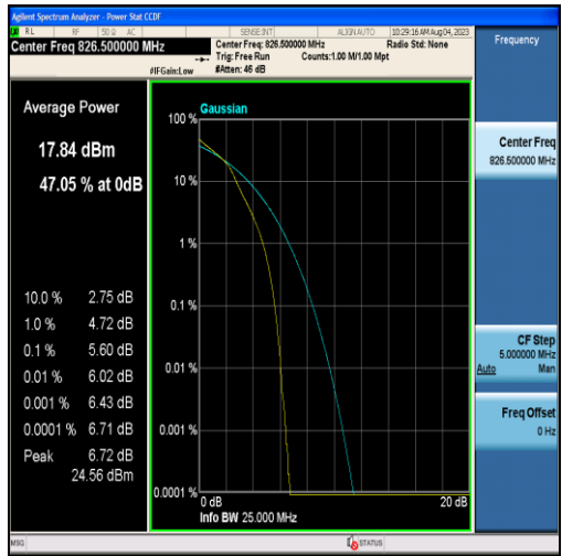
Band26-5MHz-16QAM-26815-25RB#0
