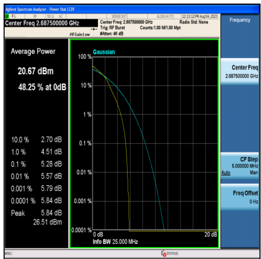
Band41-5MHz-16QAM-41565-25RB#0
