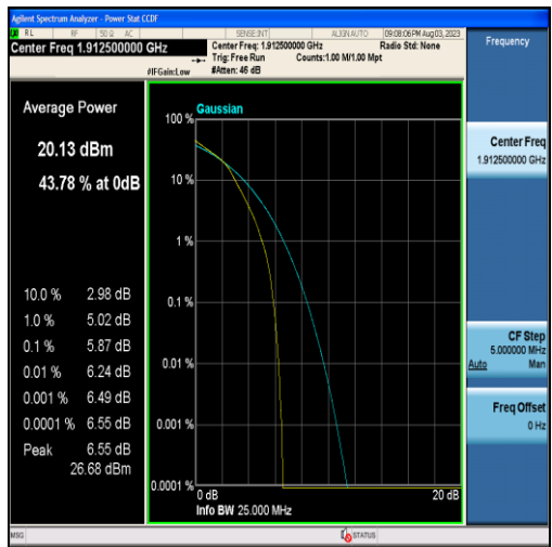
Band25-5MHz-16QAM-26665-25RB#0
