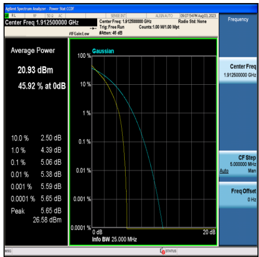
Band25-5MHz-QPSK-26665-25RB#0
