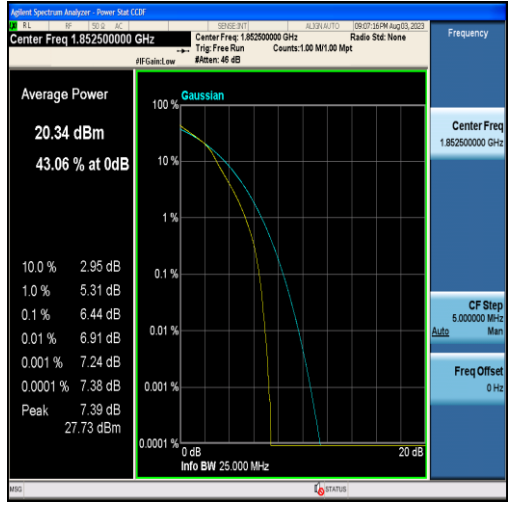
Band25-5MHz-16QAM-26065-25RB#0
