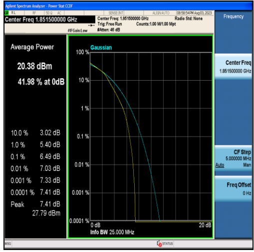
Band25-3MHz-16QAM-26055-15RB#0
