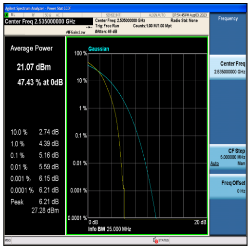
Band7-20MHz-16QAM-21100-100RB#0
