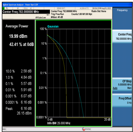
Band13-5MHz-QPSK-23230-25RB#0
