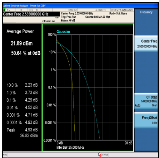
Band7-15MHz-QPSK-21100-75RB#0
