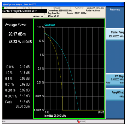
Band5-10MHz-QPSK-20525-50RB#0
