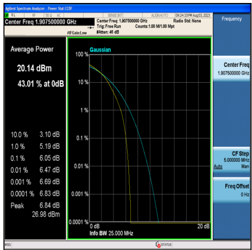
Band25-15MHz-16QAM-26615-75RB#0
