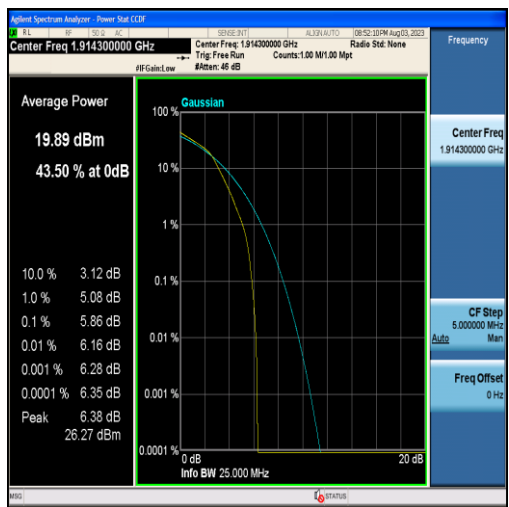
Band25-1.4MHz-16QAM-26683-6RB#0
