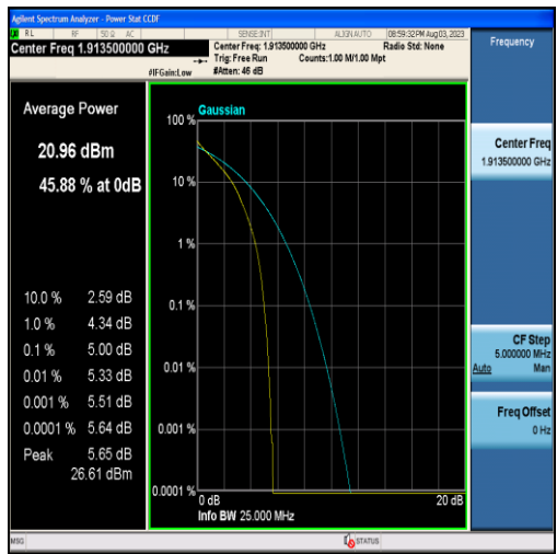
Band25-3MHz-QPSK-26675-15RB#0
