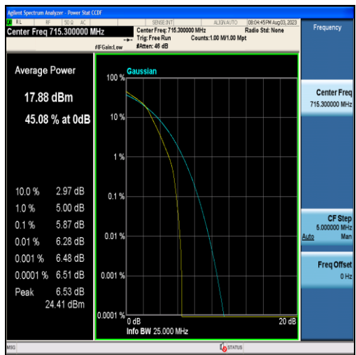
Band12-1.4MHz-16QAM-23173-6RB#0
