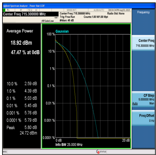
Band12-1.4MHz-QPSK-23173-6RB#0
