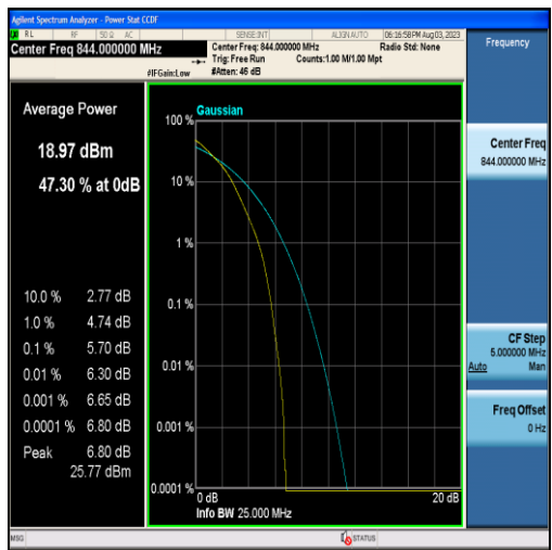
Band5-10MHz-16QAM-20600-50RB#0
