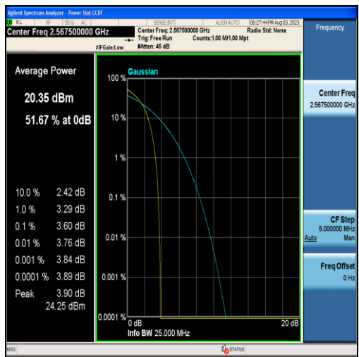
Band7-5MHz-16QAM-21425-25RB#0
