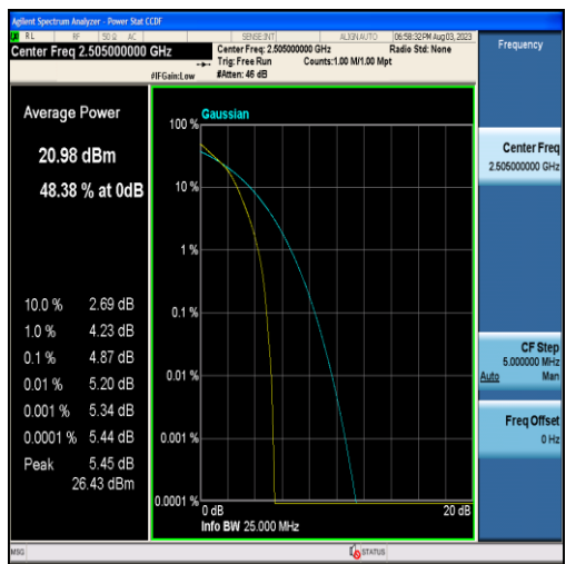
Band7-10MHz-16QAM-20800-50RB#0
