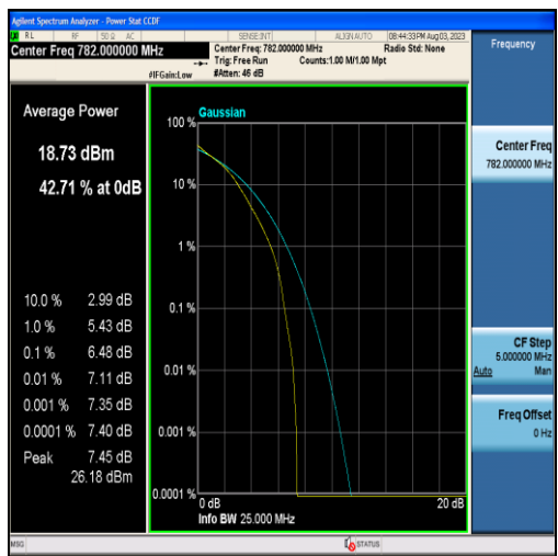
Band13-10MHz-16QAM-23230-50RB#0
