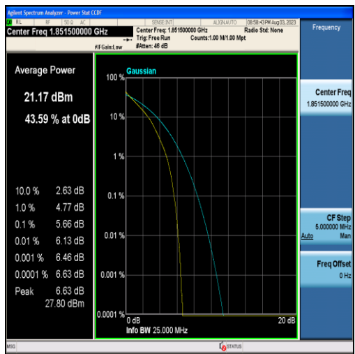
Band25-3MHz-QPSK-26055-15RB#0
