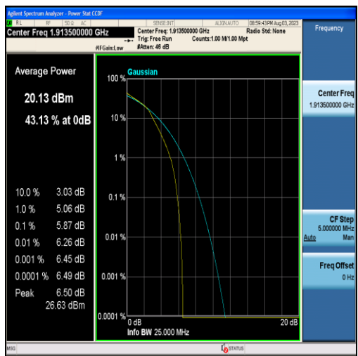
Band25-3MHz-16QAM-26675-15RB#0
