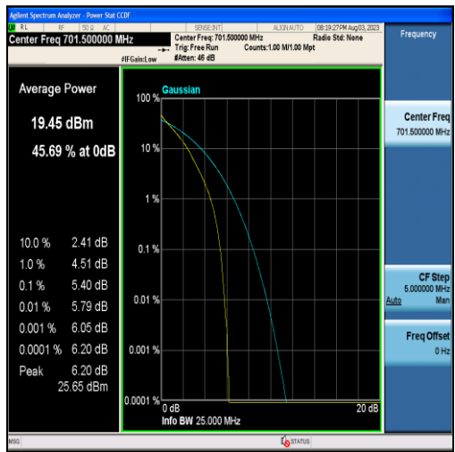
Band12-5MHz-QPSK-23035-25RB#0
