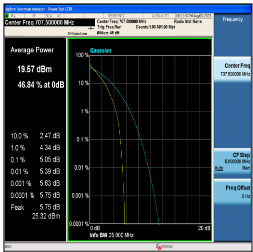
Band12-3MHz-QPSK-23095-15RB#0
