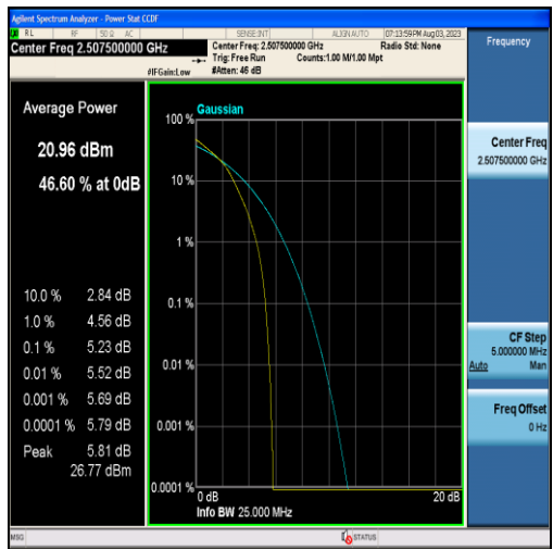
Band7-15MHz-16QAM-20825-75RB#0
