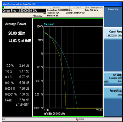
Band25-20MHz-16QAM-26140-100RB#0
