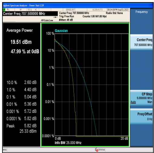
Band12-1.4MHz-QPSK-23095-6RB#0
