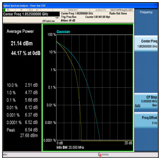
Band25-5MHz-QPSK-26065-25RB#0
