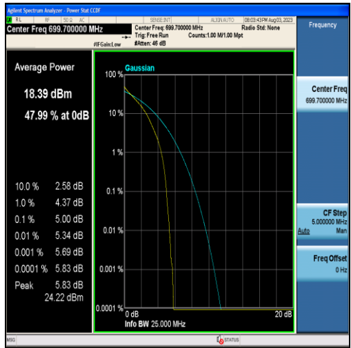
Band12-1.4MHz-QPSK-23017-6RB#0
