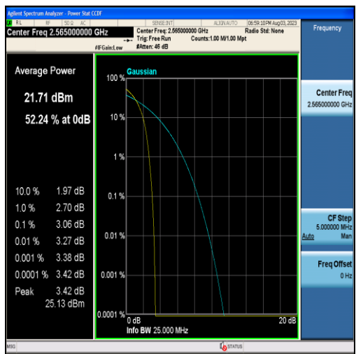
Band7-10MHz-QPSK-21400-50RB#0
