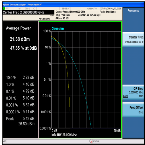
Band7-20MHz-16QAM-21350-100RB#0
