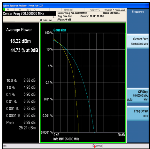
Band12-3MHz-16QAM-23025-15RB#0
