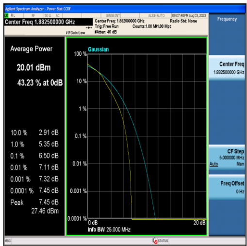
Band25-5MHz-16QAM-26365-25RB#0
