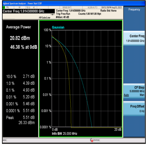
Band25-1.4MHz-QPSK-26683-6RB#0
