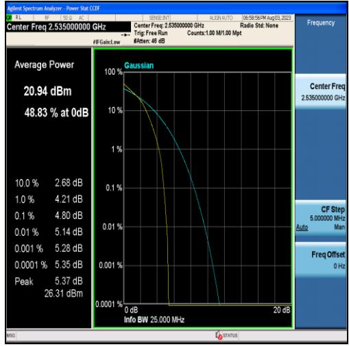
Band7-10MHz-16QAM-21100-50RB#0
