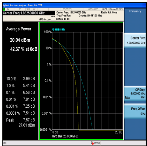
Band25-3MHz-16QAM-26365-15RB#0
