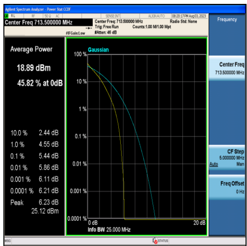
Band12-5MHz-QPSK-23155-25RB#0
