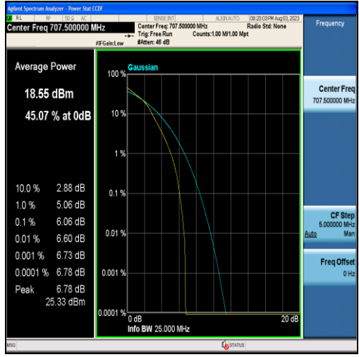
Band12-5MHz-16QAM-23095-25RB#0
