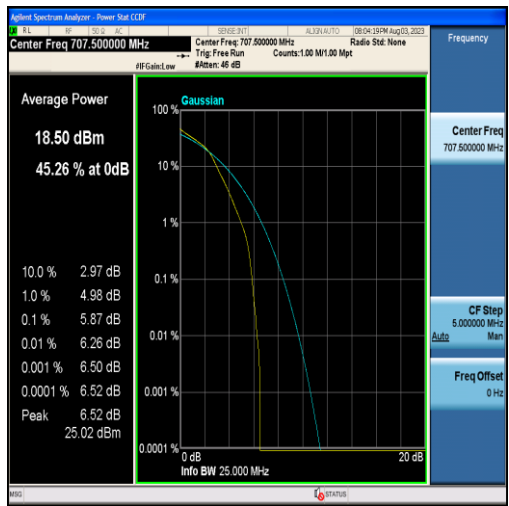
Band12-1.4MHz-16QAM-23095-6RB#0
