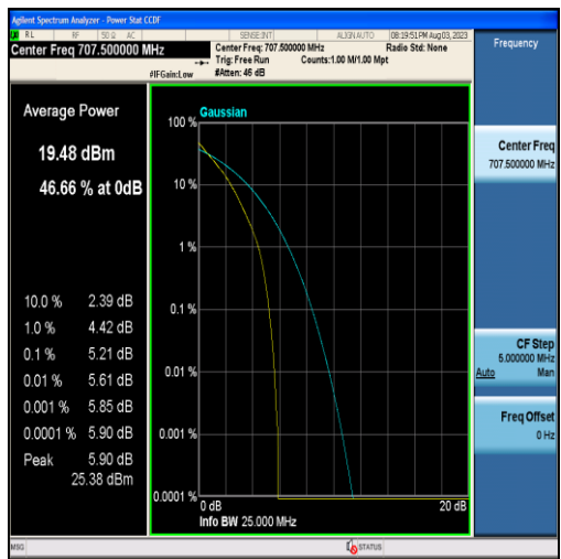
Band12-5MHz-QPSK-23095-25RB#0
