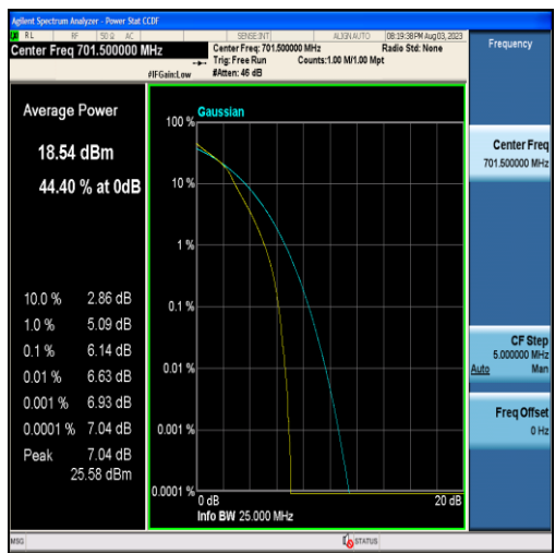
Band12-5MHz-16QAM-23035-25RB#0
