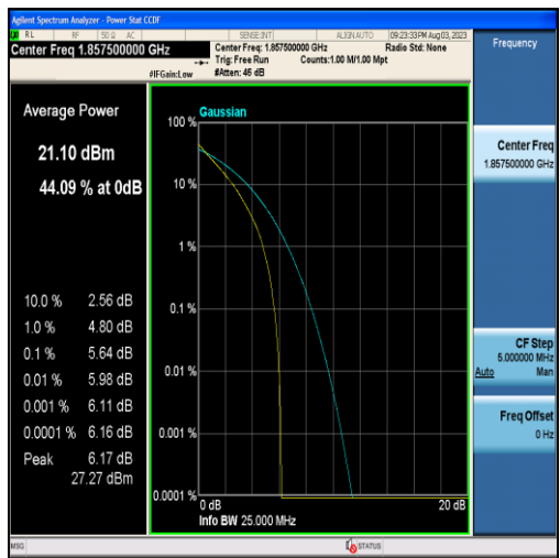
Band25-15MHz-QPSK-26115-75RB#0
