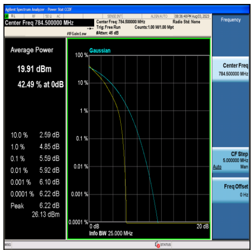
Band13-5MHz-QPSK-23255-25RB#0
