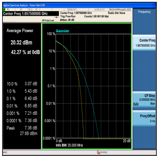
Band25-15MHz-16QAM-26115-75RB#0
