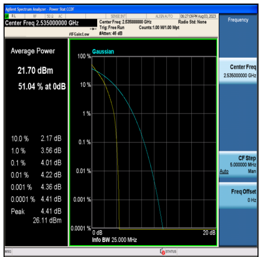
Band7-5MHz-QPSK-21100-25RB#0
