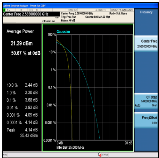
Band7-10MHz-16QAM-21400-50RB#0
