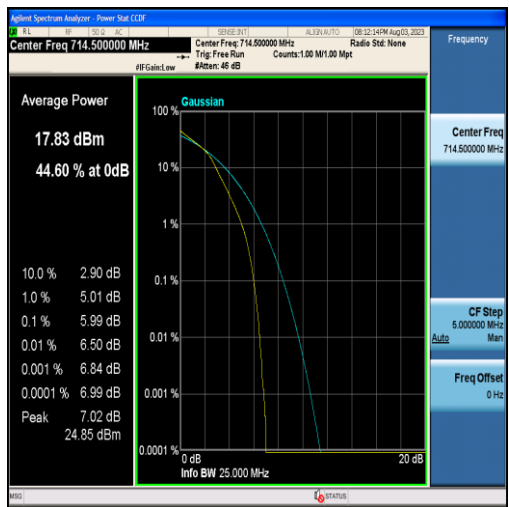
Band12-3MHz-16QAM-23165-15RB#0
