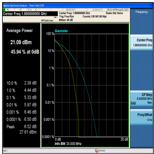
Band25-20MHz-QPSK-26140-100RB#0
