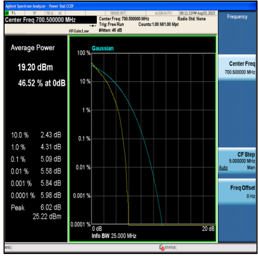
Band12-3MHz-QPSK-23025-15RB#0
