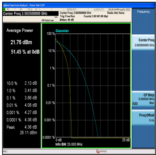
Band7-5MHz-QPSK-20775-25RB#0
