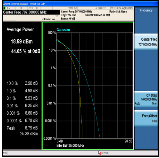
Band12-3MHz-16QAM-23095-15RB#0
