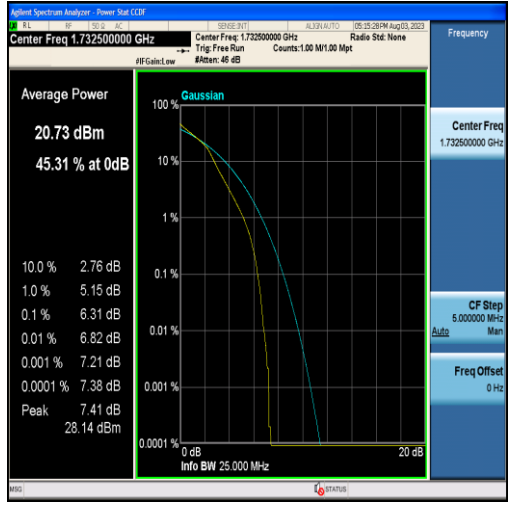
Band4-3MHz-16QAM-20175-15RB#0
