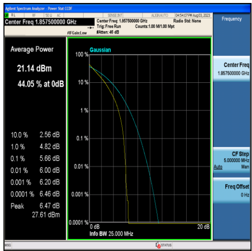
Band2-15MHz-QPSK-18675-75RB#0
