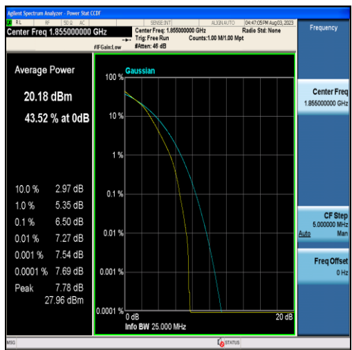
Band2-10MHz-16QAM-18650-50RB#0
