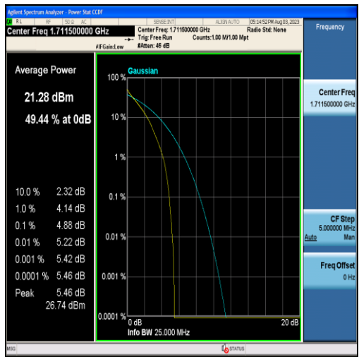
Band4-3MHz-QPSK-19965-15RB#0
