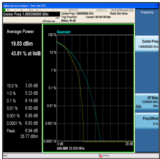
Band2-1.4MHz-16QAM-19193-6RB#0
