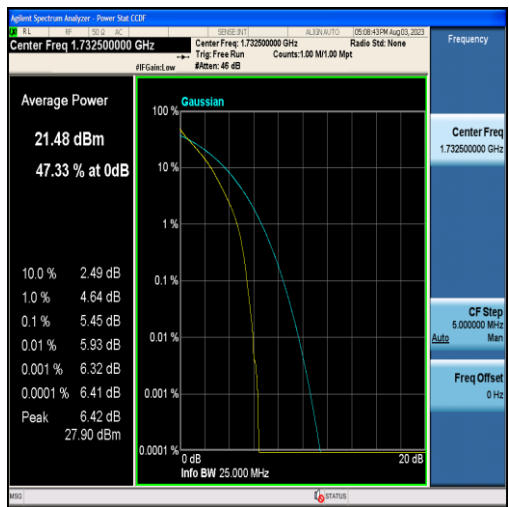
Band4-1.4MHz-QPSK-20175-6RB#0
