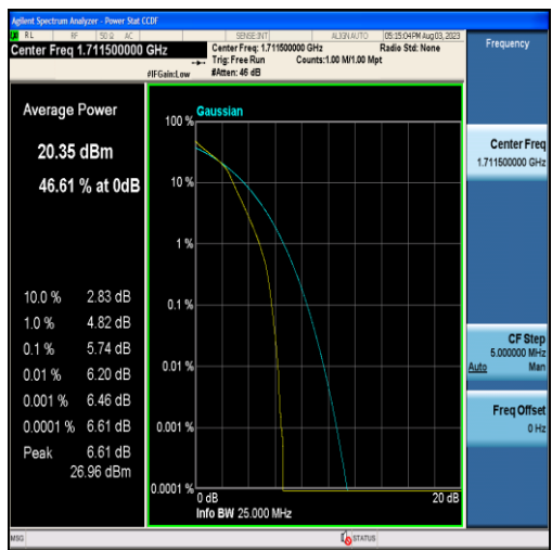
Band4-3MHz-16QAM-19965-15RB#0
