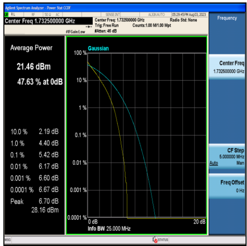
Band4-10MHz-QPSK-20175-50RB#0
