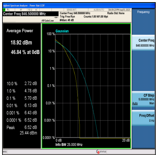
Band5-5MHz-16QAM-20625-25RB#0
