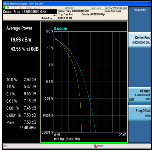
Band2-5MHz-16QAM-18900-25RB#0
