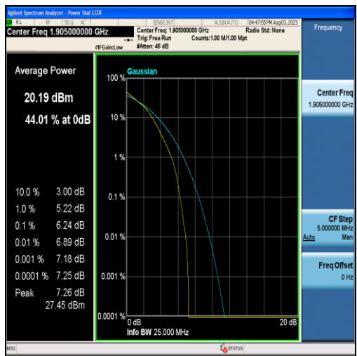
Band2-10MHz-16QAM-19150-50RB#0
