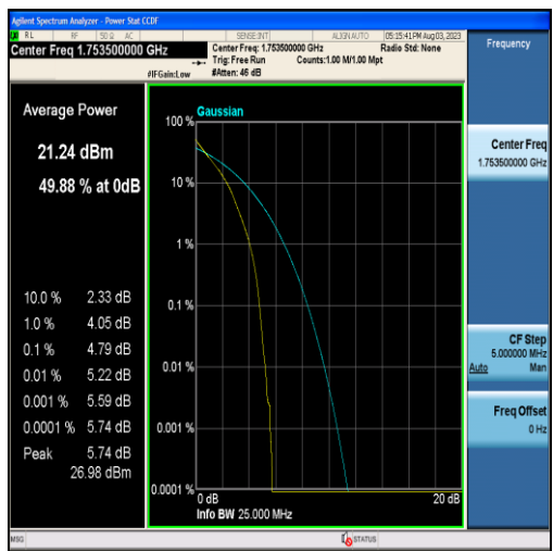
Band4-3MHz-QPSK-20385-15RB#0
