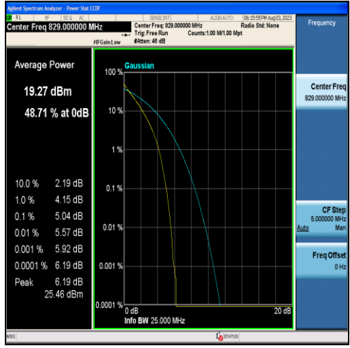
Band5-10MHz-QPSK-20450-50RB#0
