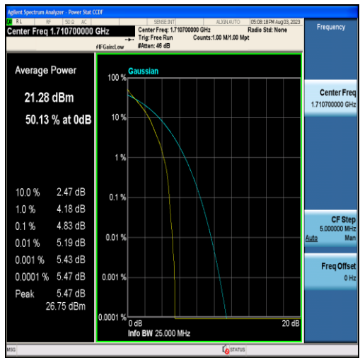
Band4-1.4MHz-QPSK-19957-6RB#0
