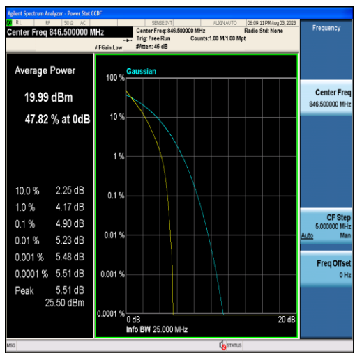
Band5-5MHz-QPSK-20625-25RB#0
