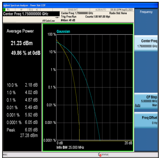
Band4-10MHz-QPSK-20350-50RB#0
