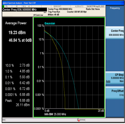
Band5-5MHz-16QAM-20525-25RB#0
