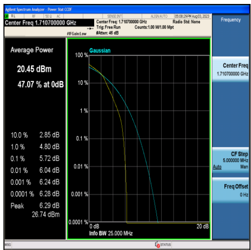
Band4-1.4MHz-16QAM-19957-6RB#0
