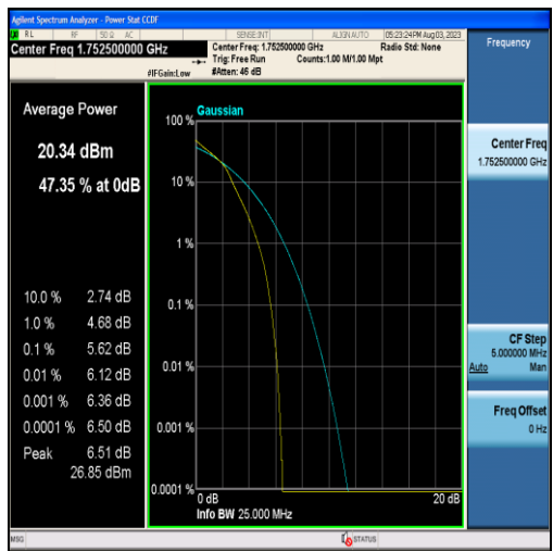
Band4-5MHz-16QAM-20375-25RB#0
