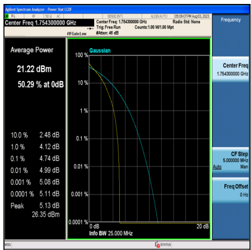
Band4-1.4MHz-QPSK-20393-6RB#0
