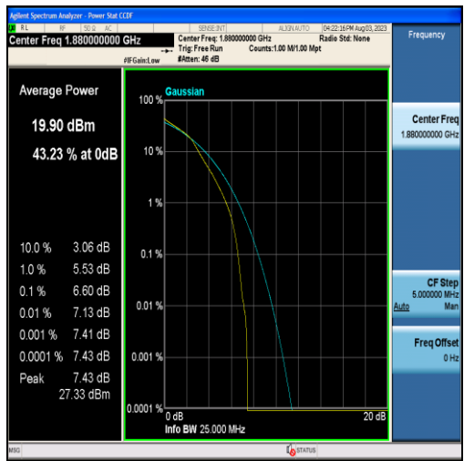
Band2-1.4MHz-16QAM-18900-6RB#0
