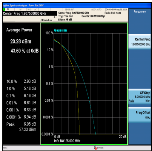
Band2-5MHz-16QAM-19175-25RB#0
