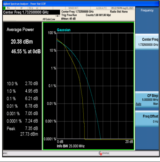
Band4-5MHz-16QAM-20175-25RB#0
