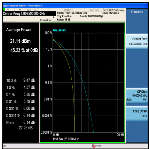
Band2-5MHz-QPSK-19175-25RB#0
