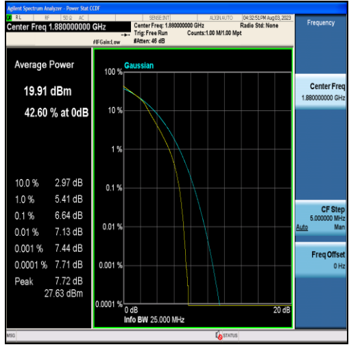
Band2-3MHz-16QAM-18900-15RB#0
