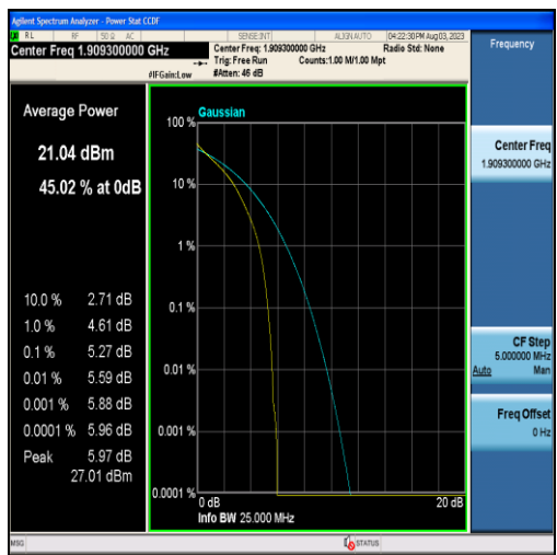
Band2-1.4MHz-QPSK-19193-6RB#0
