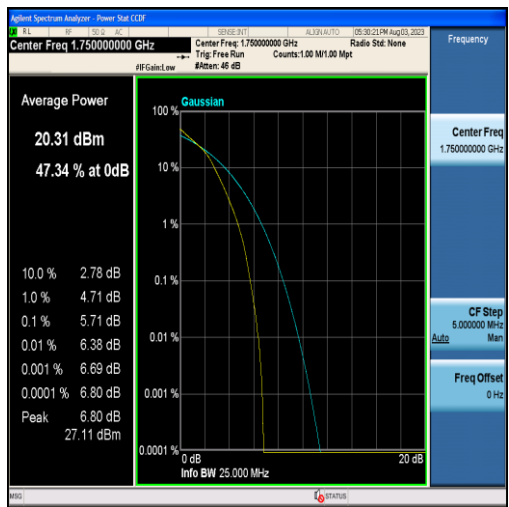
Band4-10MHz-16QAM-20350-50RB#0
