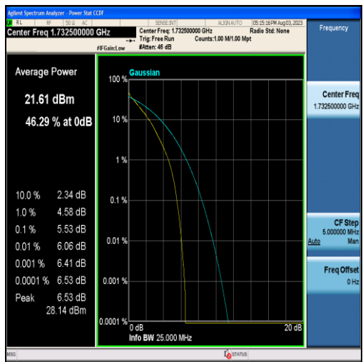
Band4-3MHz-QPSK-20175-15RB#0
