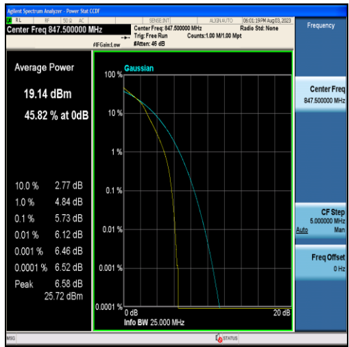
Band5-3MHz-16QAM-20635-15RB#0
