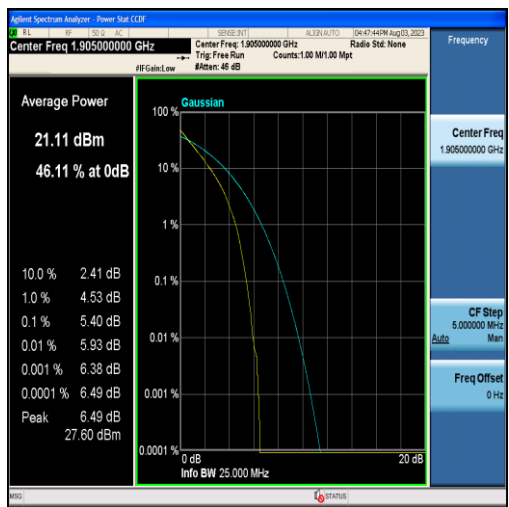
Band2-10MHz-QPSK-19150-50RB#0
