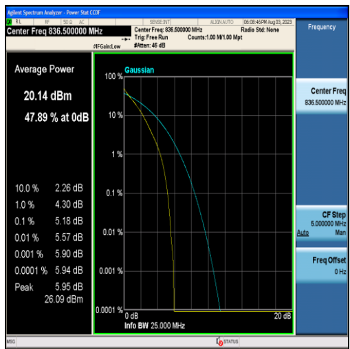
Band5-5MHz-QPSK-20525-25RB#0
