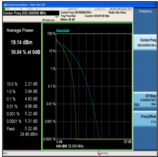
Band5-5MHz-QPSK-20425-25RB#0
