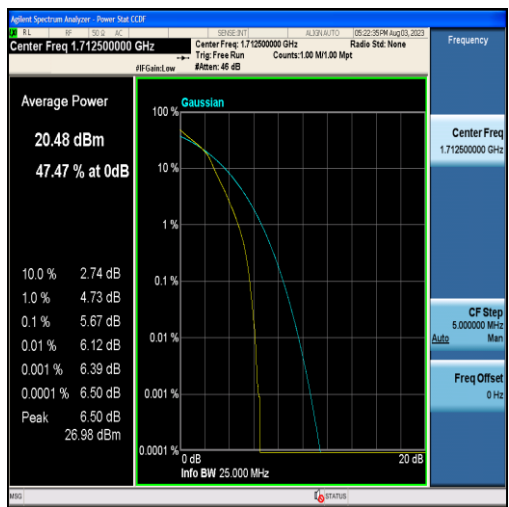
Band4-5MHz-16QAM-19975-25RB#0
