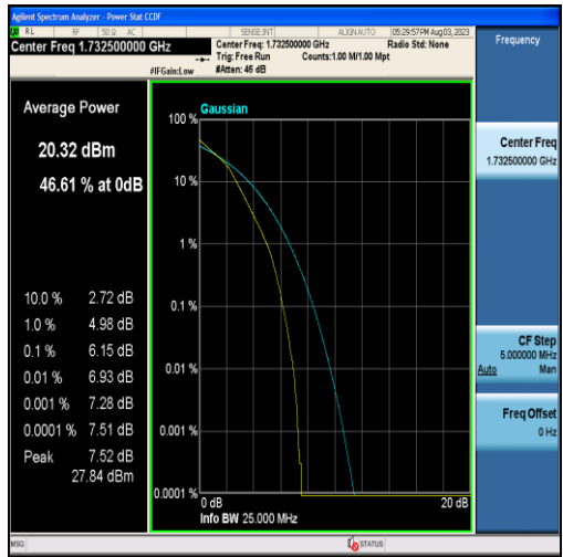
Band4-10MHz-16QAM-20175-50RB#0
