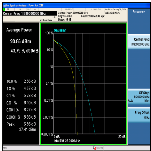
Band2-15MHz-QPSK-18900-75RB#0
