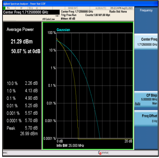
Band4-5MHz-QPSK-19975-25RB#0
