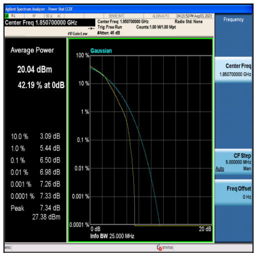
Band2-1.4MHz-16QAM-18607-6RB#0
