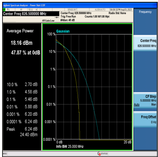
Band5-5MHz-16QAM-20425-25RB#0
