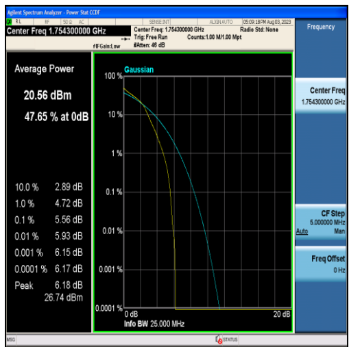
Band4-1.4MHz-16QAM-20393-6RB#0
