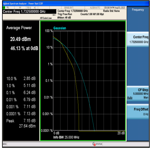
Band4-1.4MHz-16QAM-20175-6RB#0
