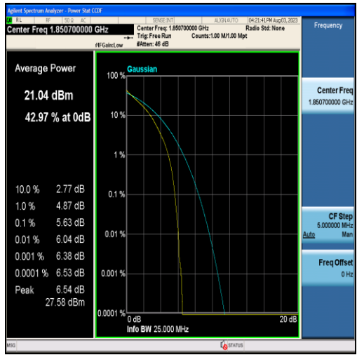
Band2-1.4MHz-QPSK-18607-6RB#0
