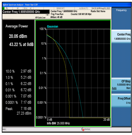
Band2-3MHz-16QAM-19185-15RB#0
