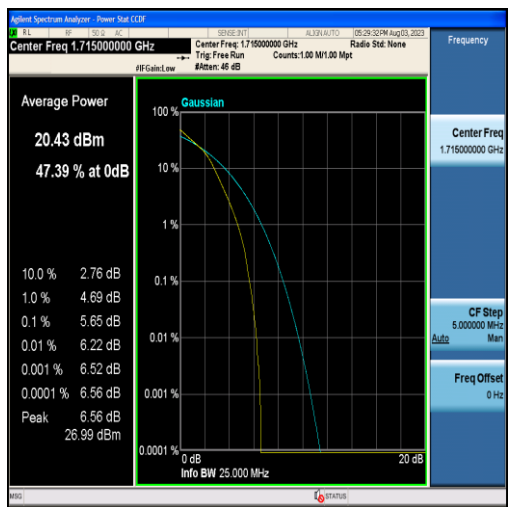
Band4-10MHz-16QAM-20000-50RB#0
