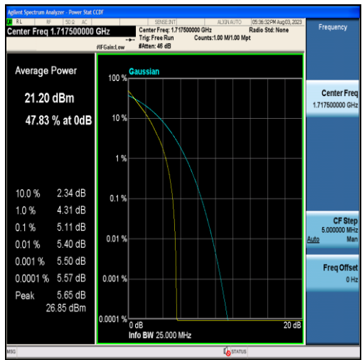
Band4-15MHz-QPSK-20025-75RB#0
