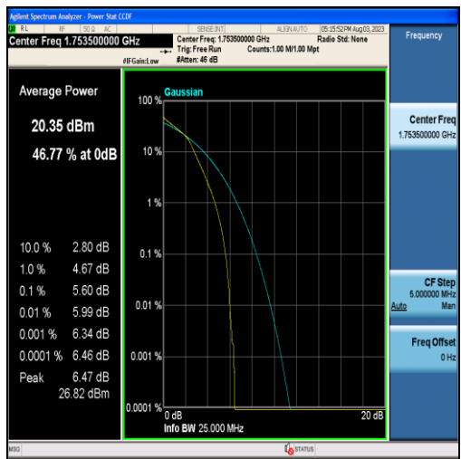
Band4-3MHz-16QAM-20385-15RB#0
