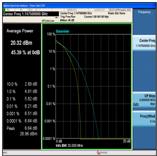
Band4-15MHz-16QAM-20325-75RB#0
