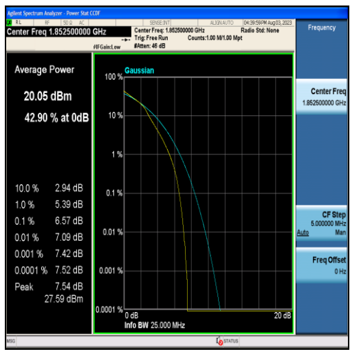
Band2-5MHz-16QAM-18625-25RB#0
