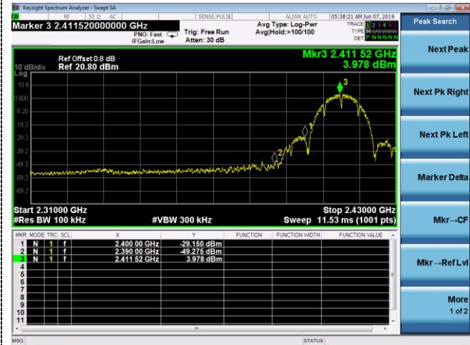
Left bandedge
