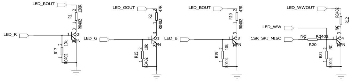
Circuit of 20001 Strip Light
